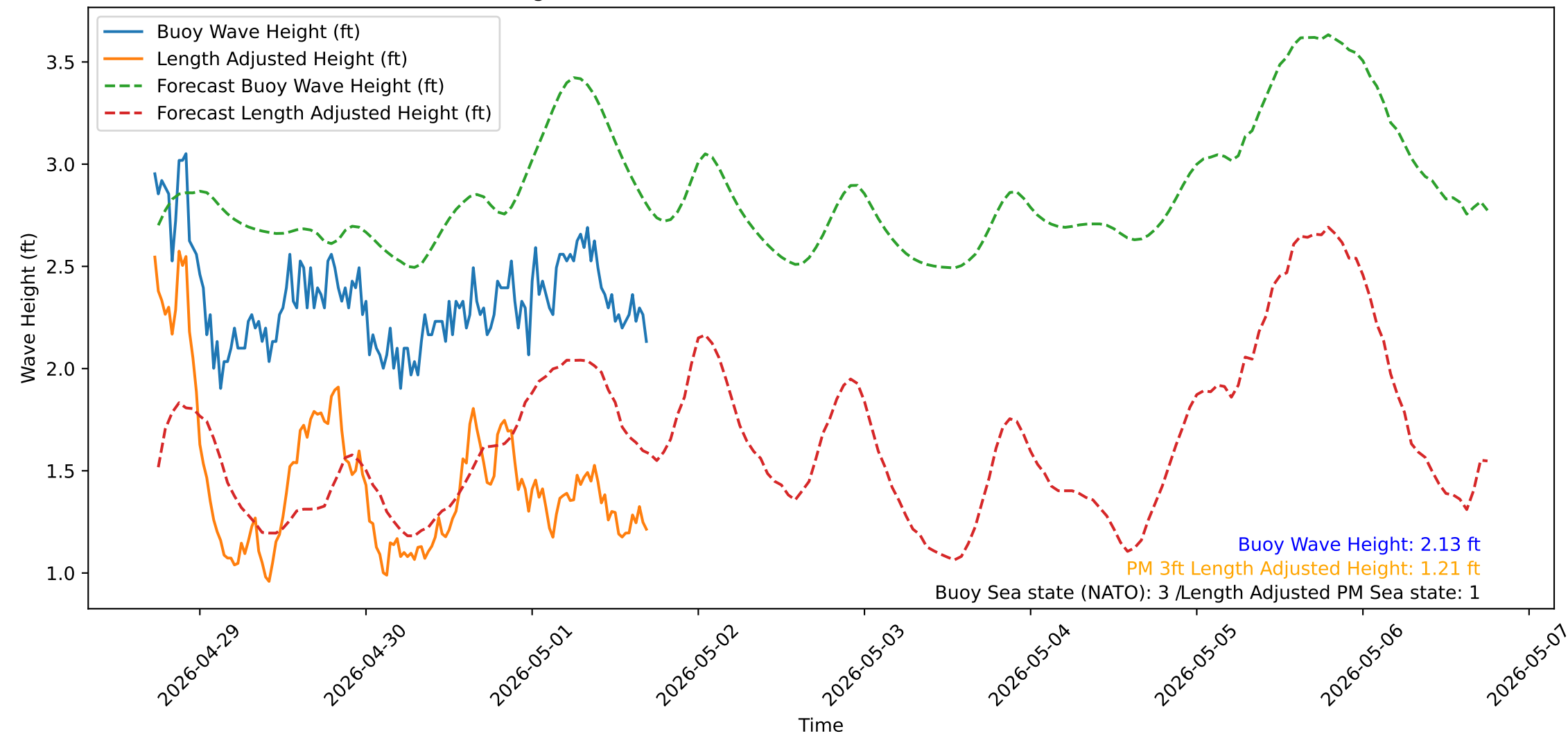
Wave Heights over Time for Oceanside Harbor at 2026-05-01 17:30:31
