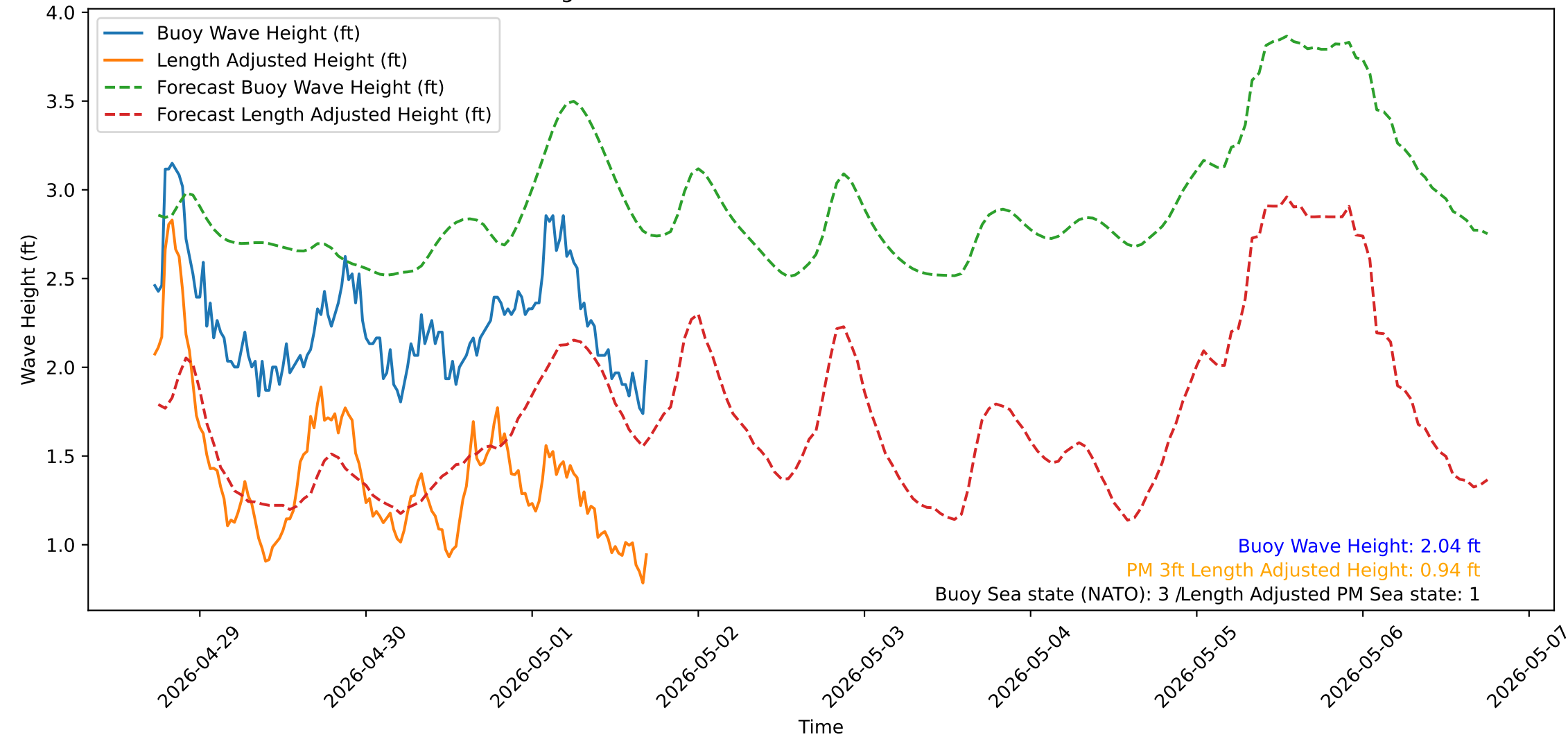
Wave Heights over Time for Green Beach at 2026-05-01 17:31:13
