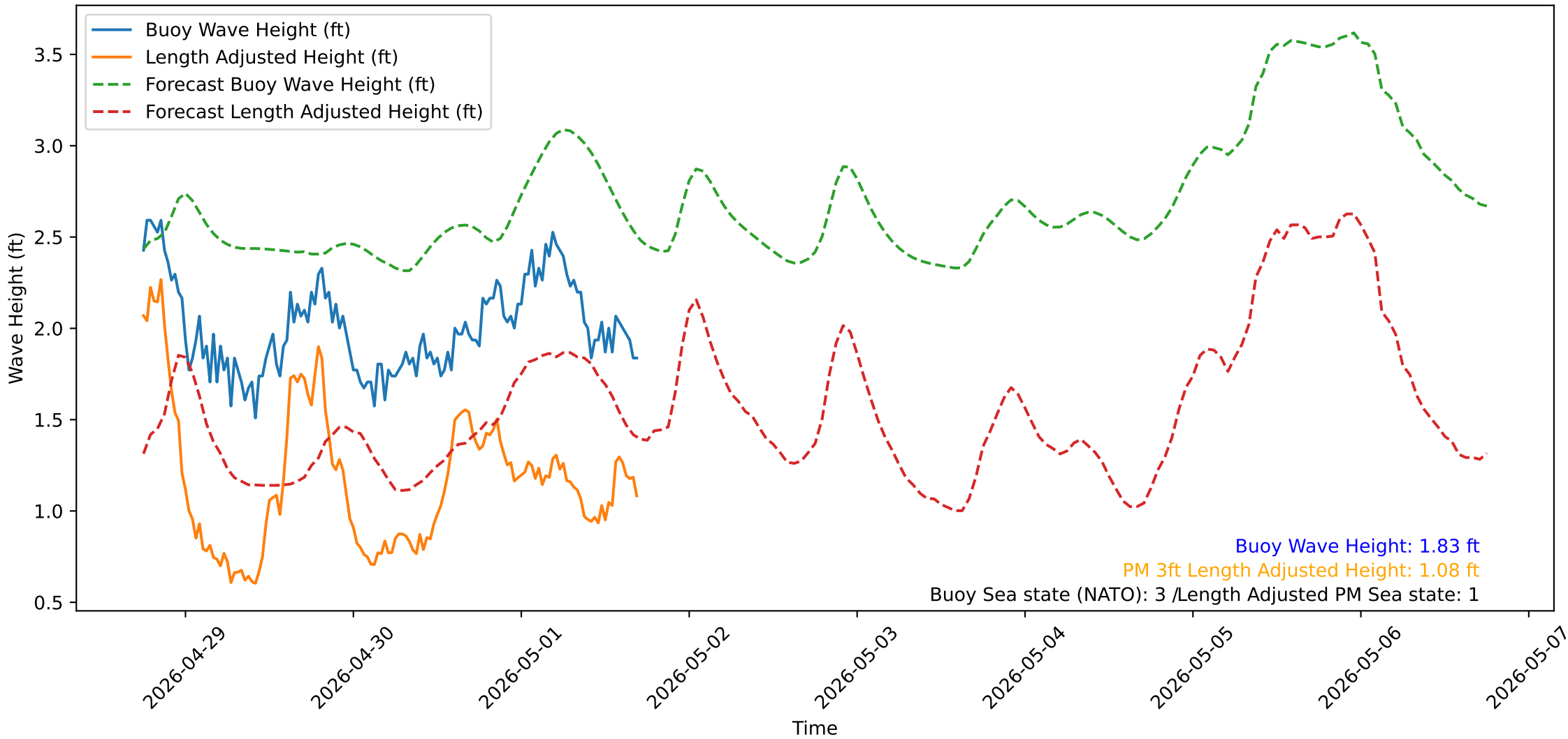
Wave Heights over Time for Red Beach at 2026-05-01 17:30:50
