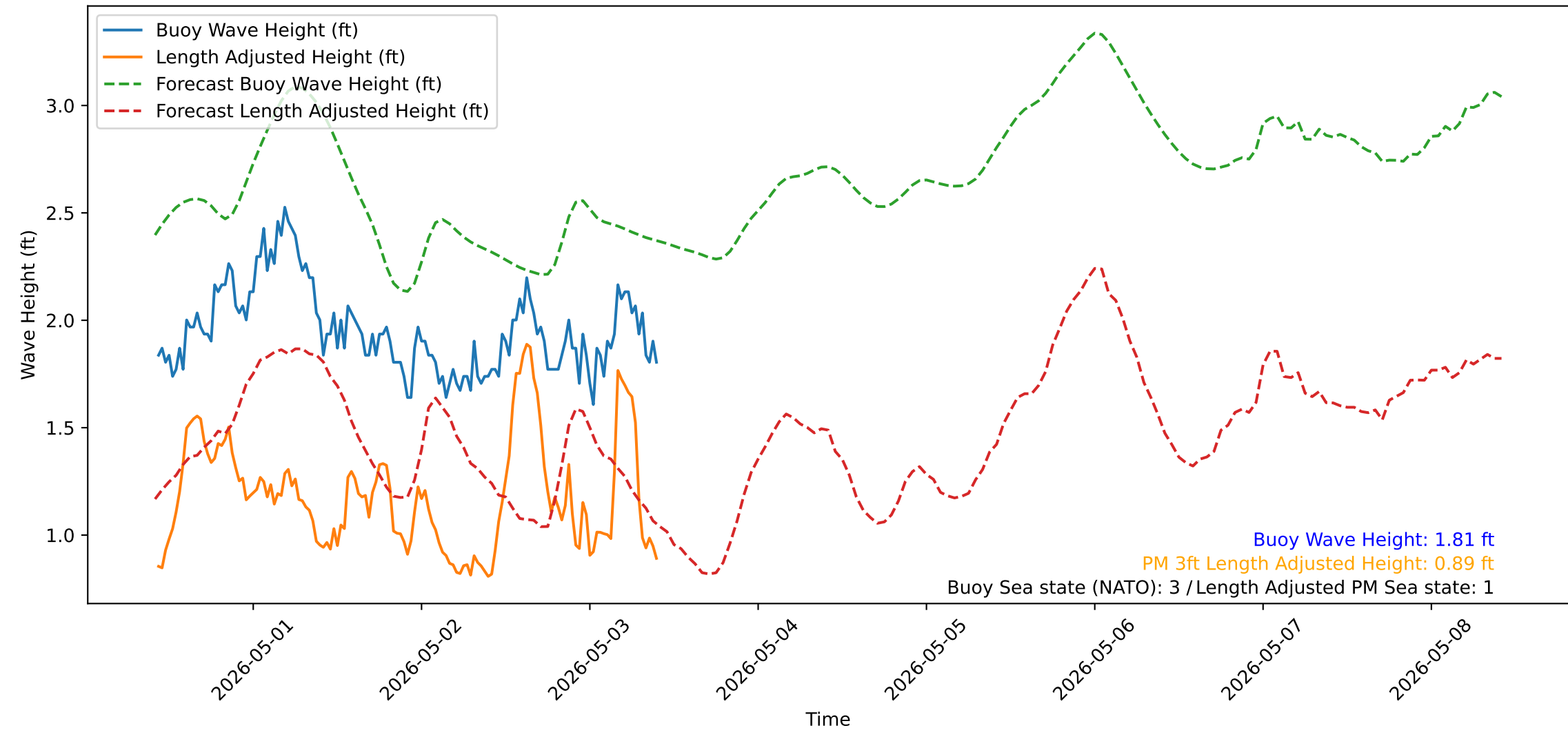
Wave Heights over Time for Red Beach at 2026-05-03 10:20:51
