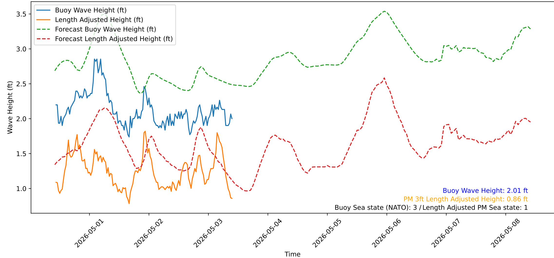
Wave Heights over Time for Green Beach at 2026-05-03 10:21:14
