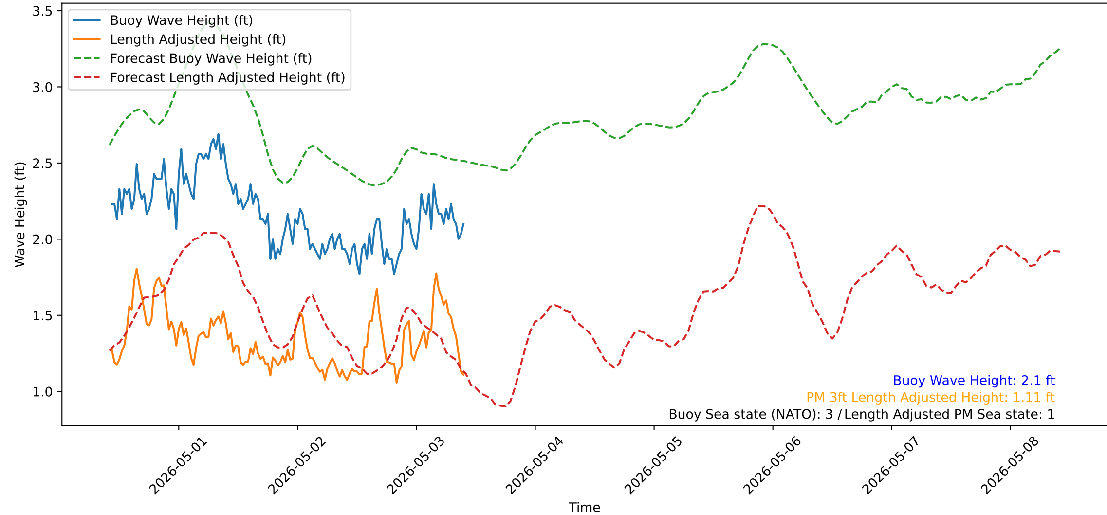
Wave Heights over Time for Oceanside Harbor at 2026-05-03 10:20:31
