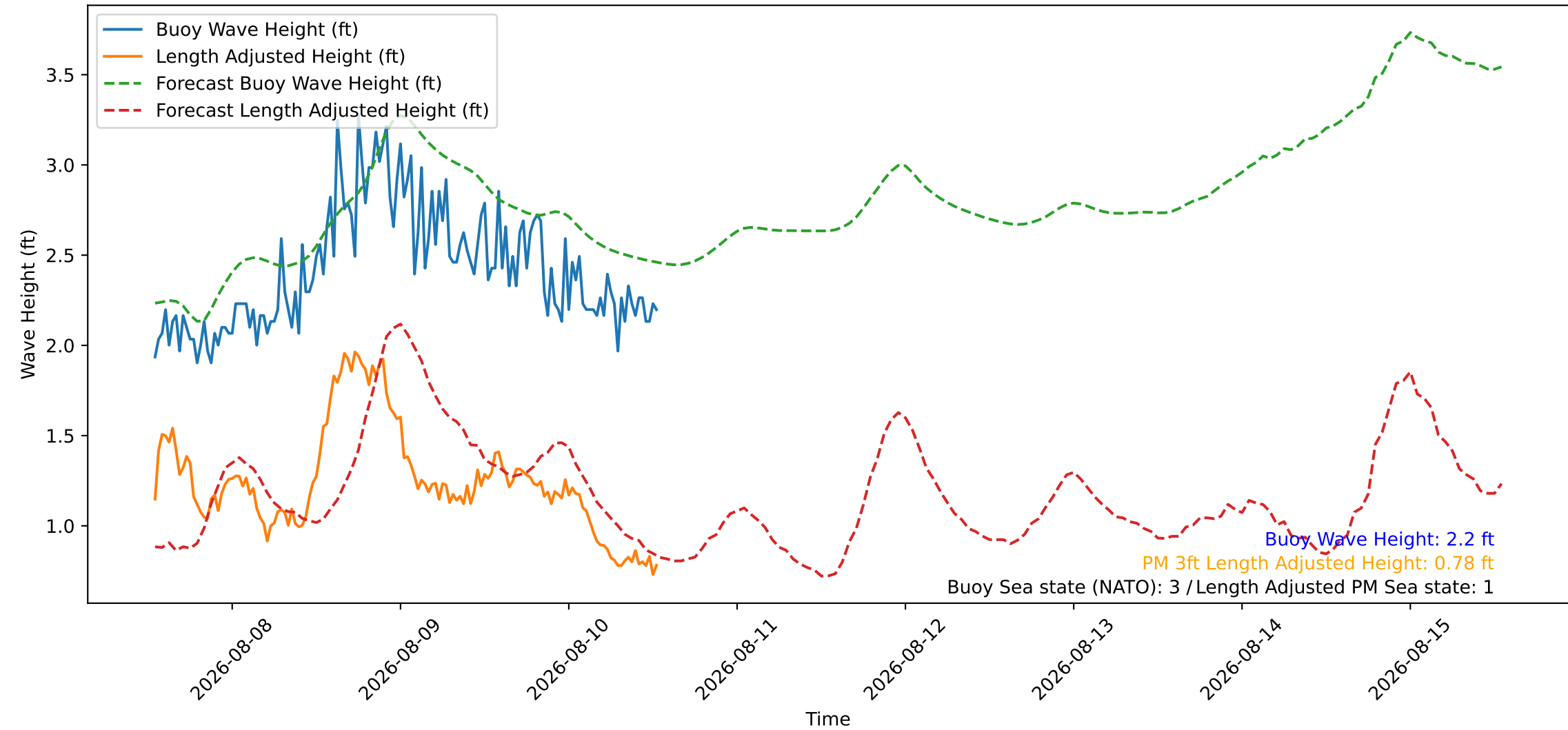
Wave Heights over Time for Oceanside Harbor at 2026-08-10 13:10:27
