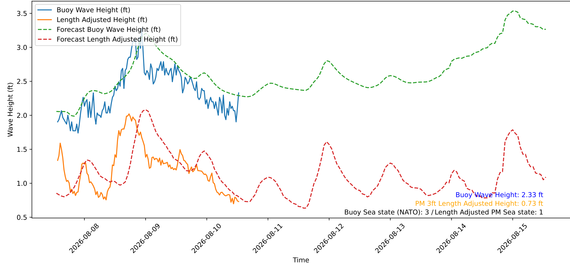
Wave Heights over Time for Red Beach at 2026-08-10 13:10:46
