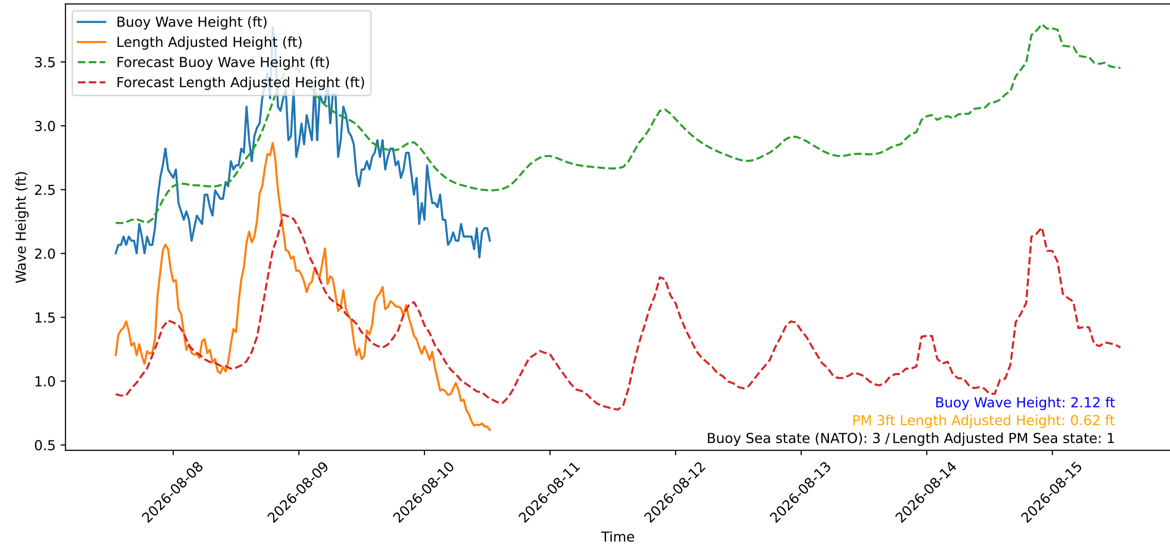
Wave Heights over Time for Green Beach at 2026-08-10 13:11:09
