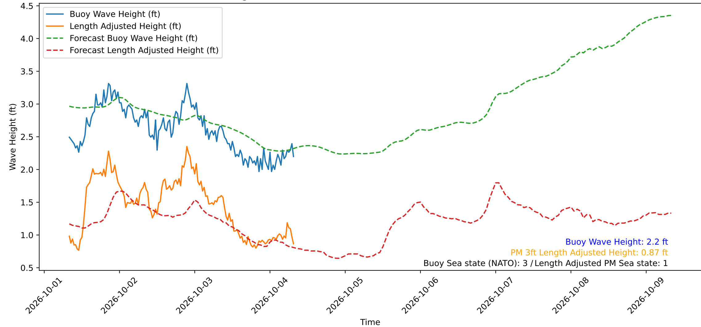
Wave Heights over Time for Oceanside Harbor at 2026-10-04 08:10:29
