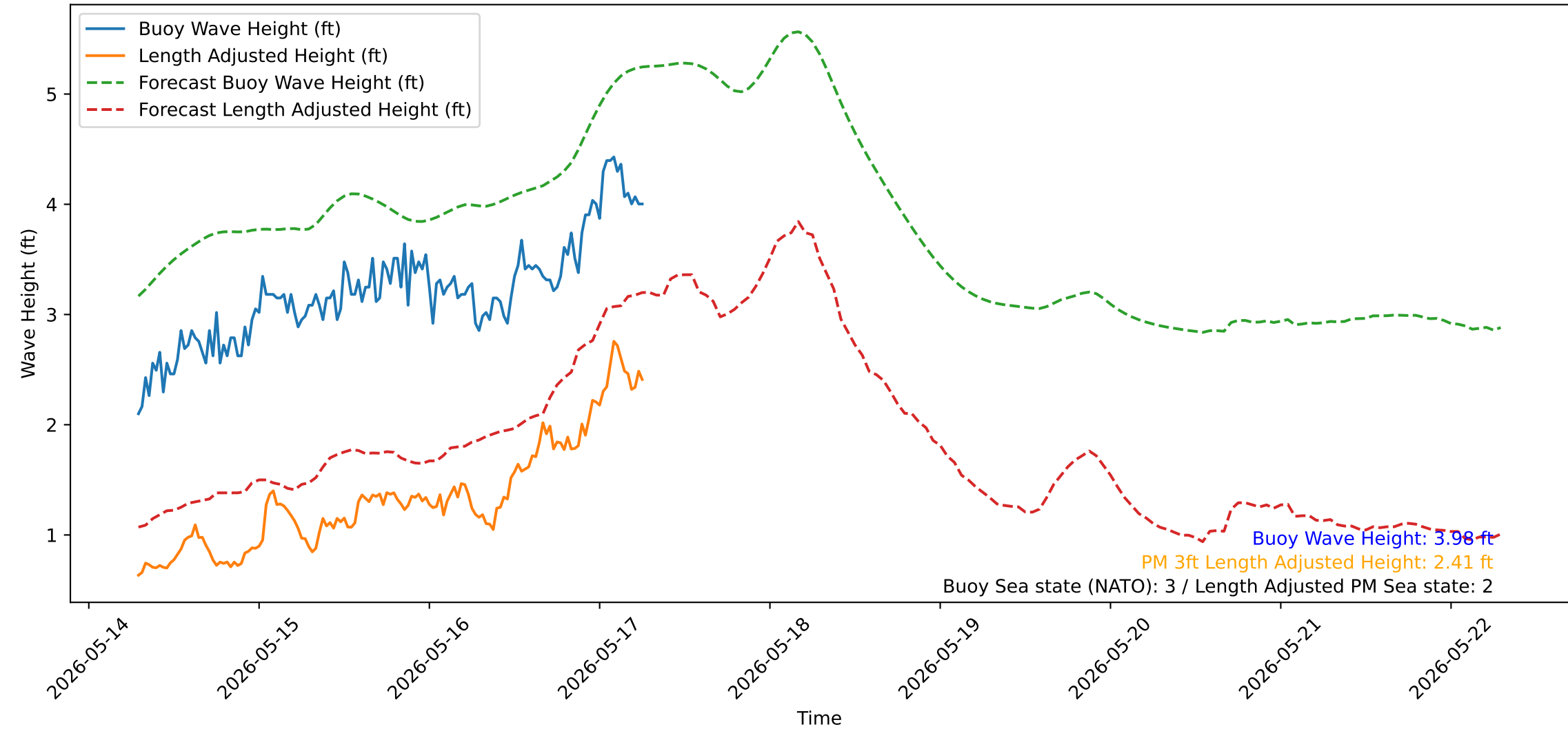
Wave Heights over Time for Green Beach at 2026-05-17 07:01:13
