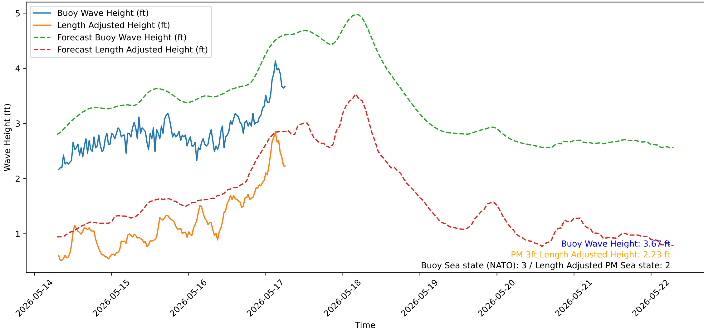
Wave Heights over Time for Red Beach at 2026-05-17 07:00:51
