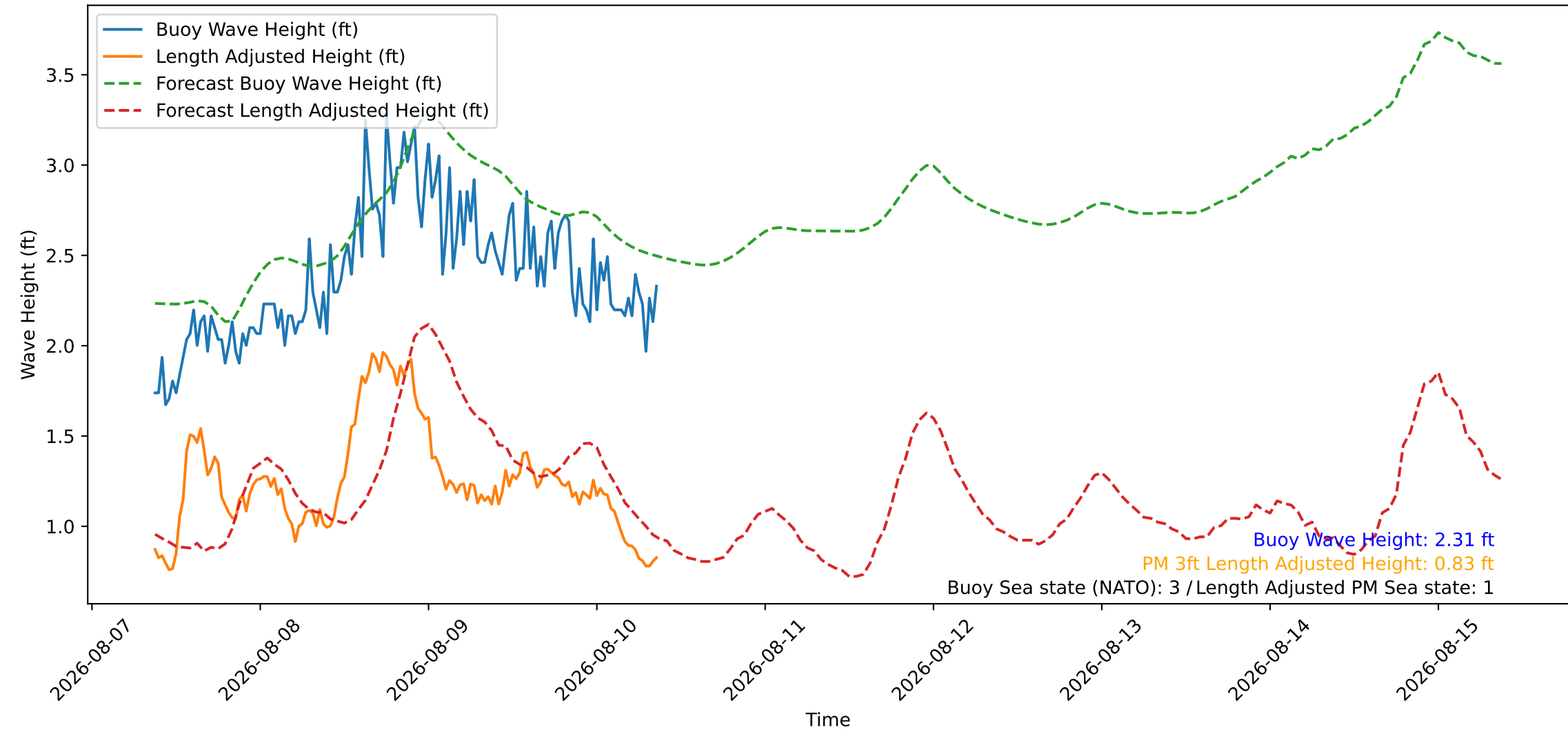
Wave Heights over Time for Oceanside Harbor at 2026-08-10 09:10:26
