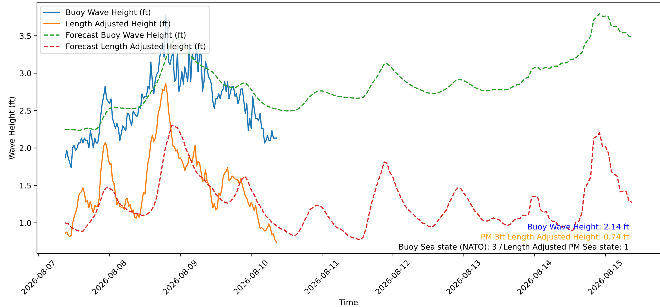
Wave Heights over Time for Green Beach at 2026-08-10 09:11:09
