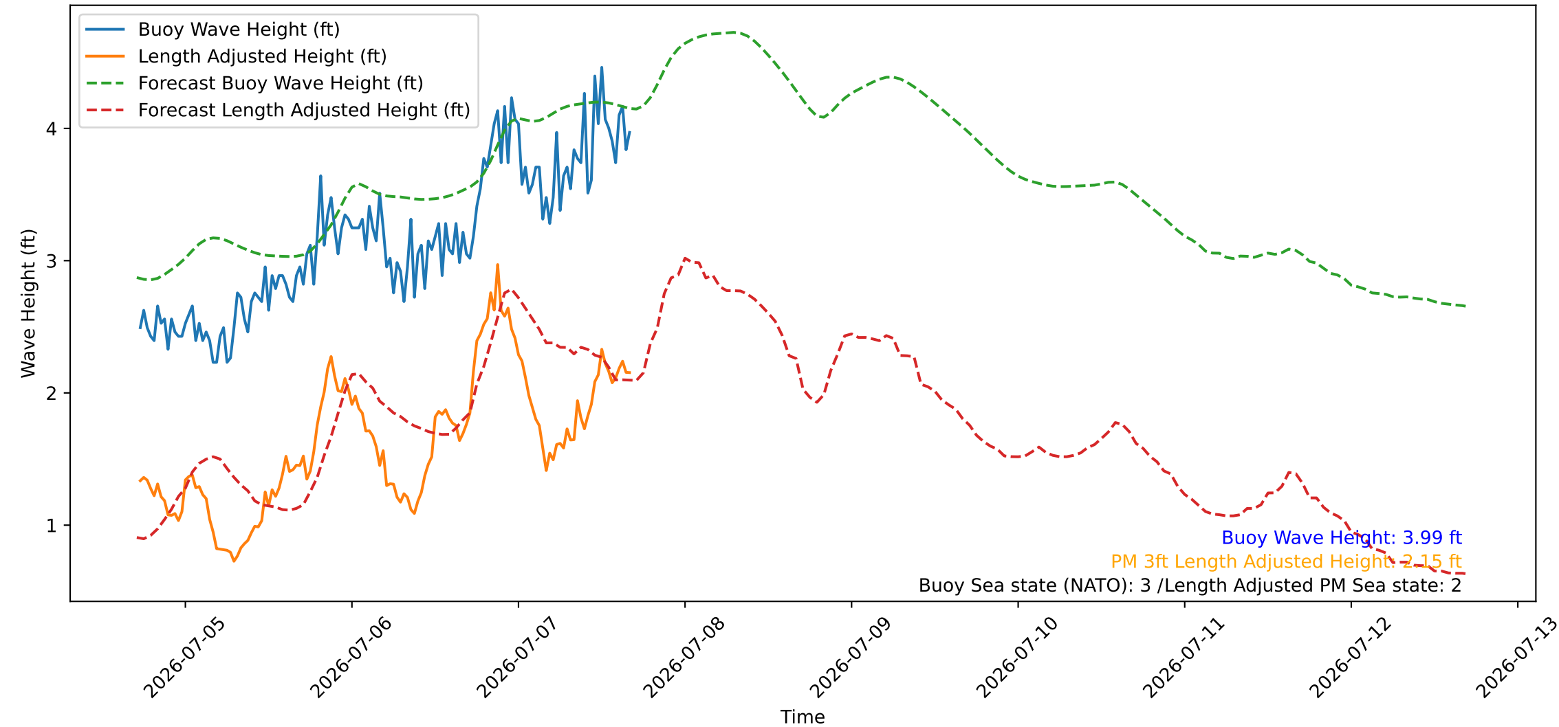
Wave Heights over Time for Red Beach at 2026-07-07 17:10:46
