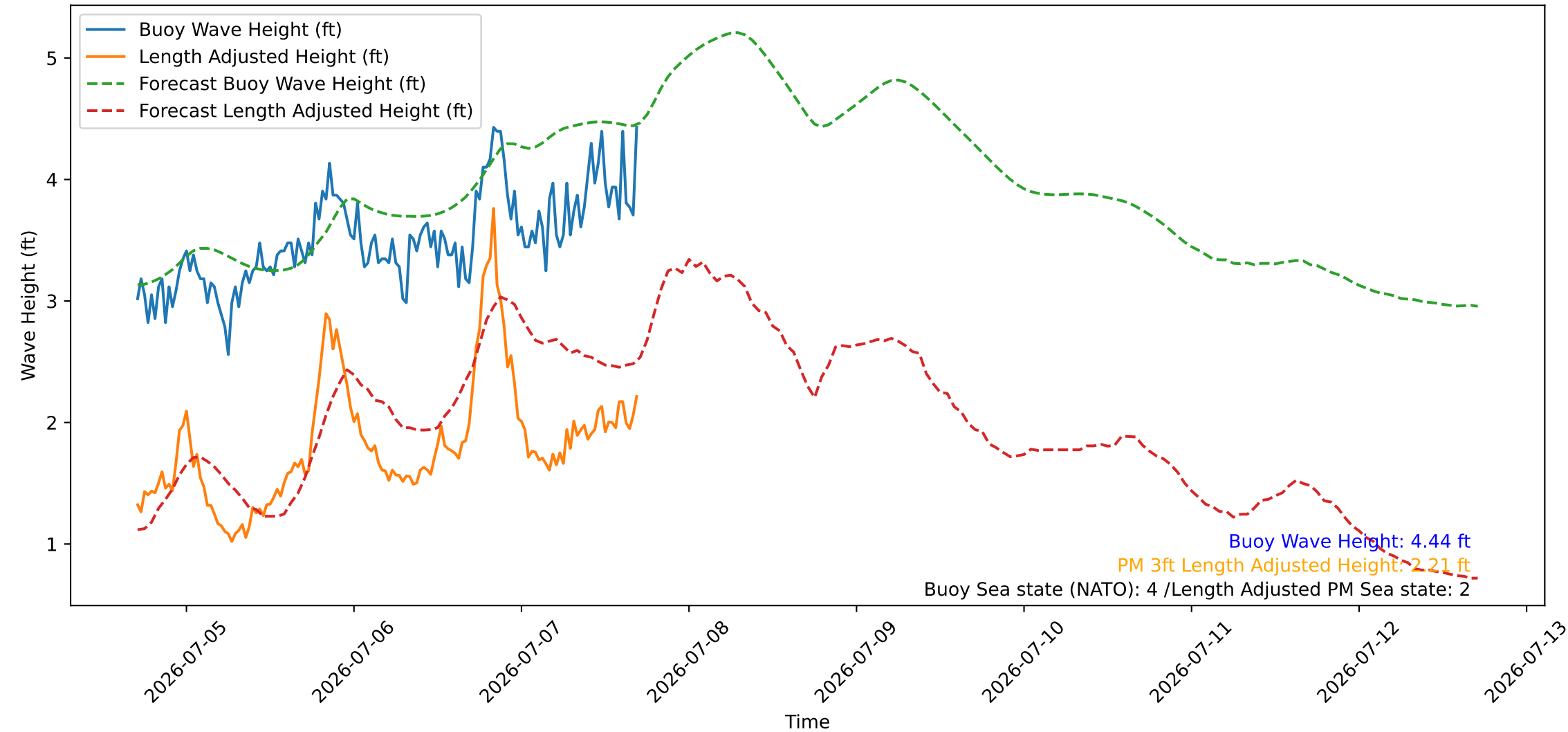
Wave Heights over Time for Green Beach at 2026-07-07 17:11:08
