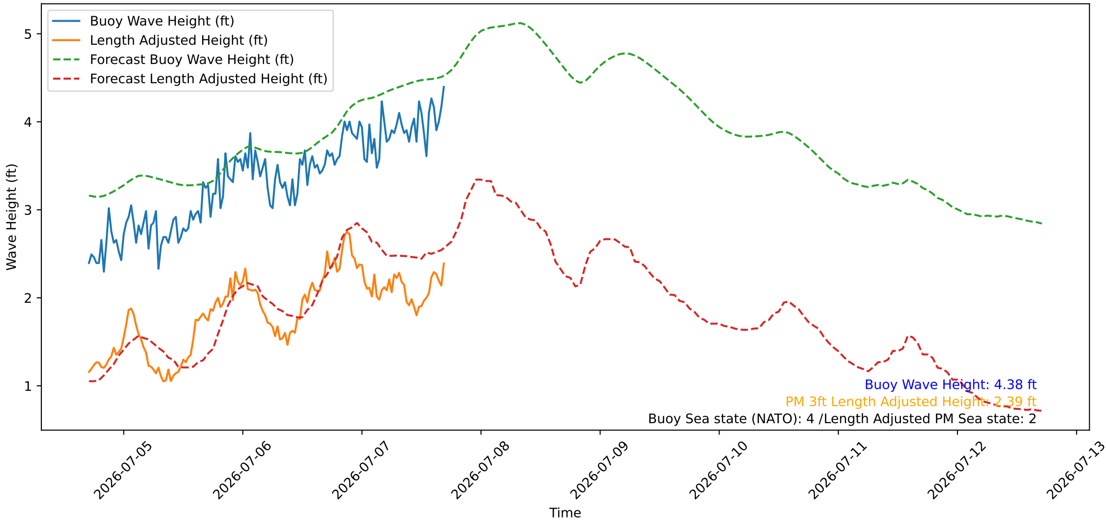
Wave Heights over Time for Oceanside Harbor at 2026-07-07 17:10:26
