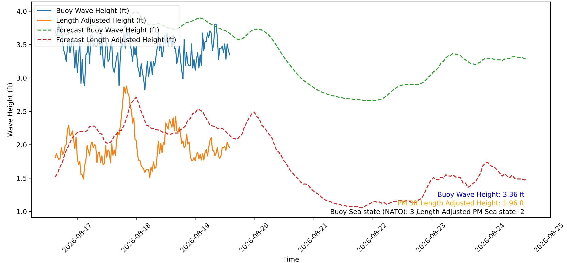
Wave Heights over Time for Oceanside Harbor at 2026-08-19 14:50:26
