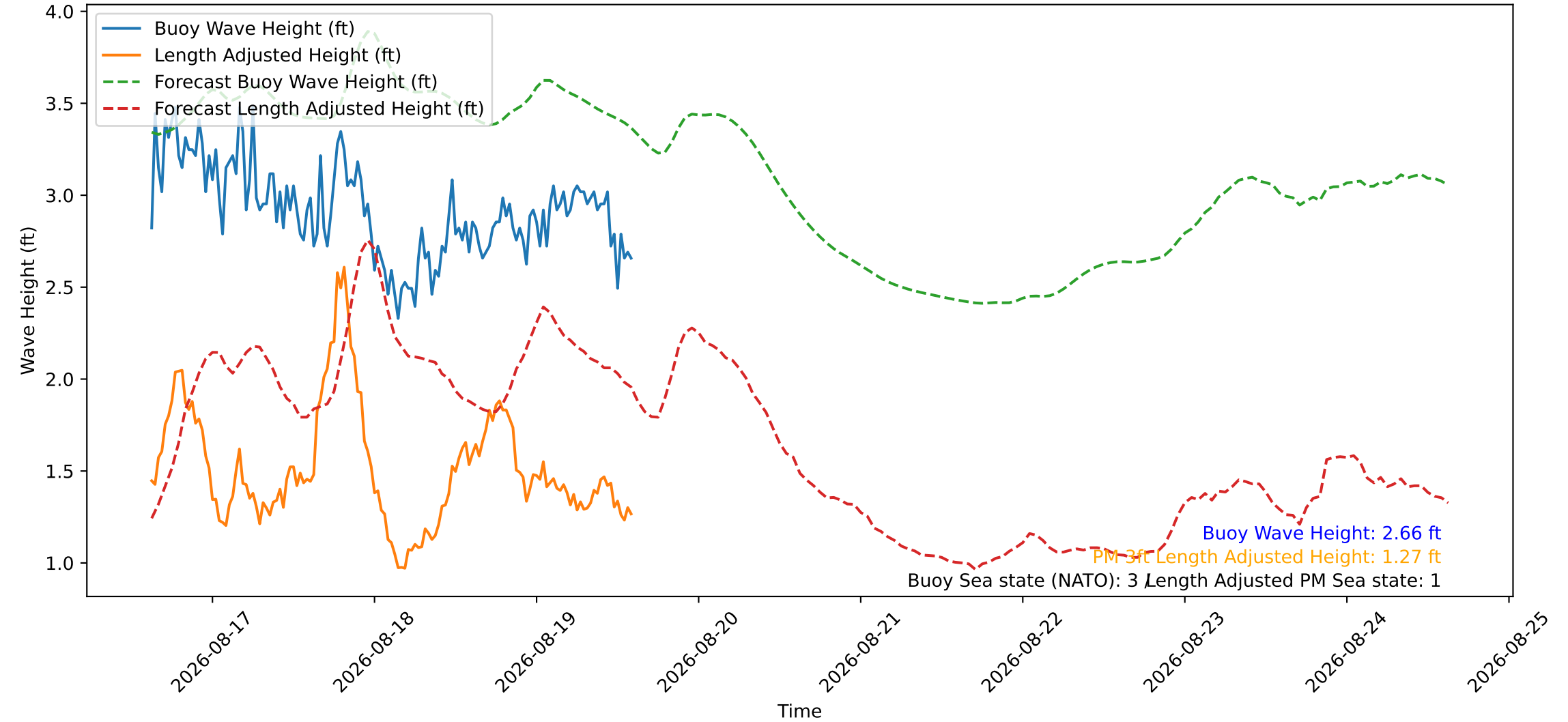
Wave Heights over Time for Red Beach at 2026-08-19 14:50:47
