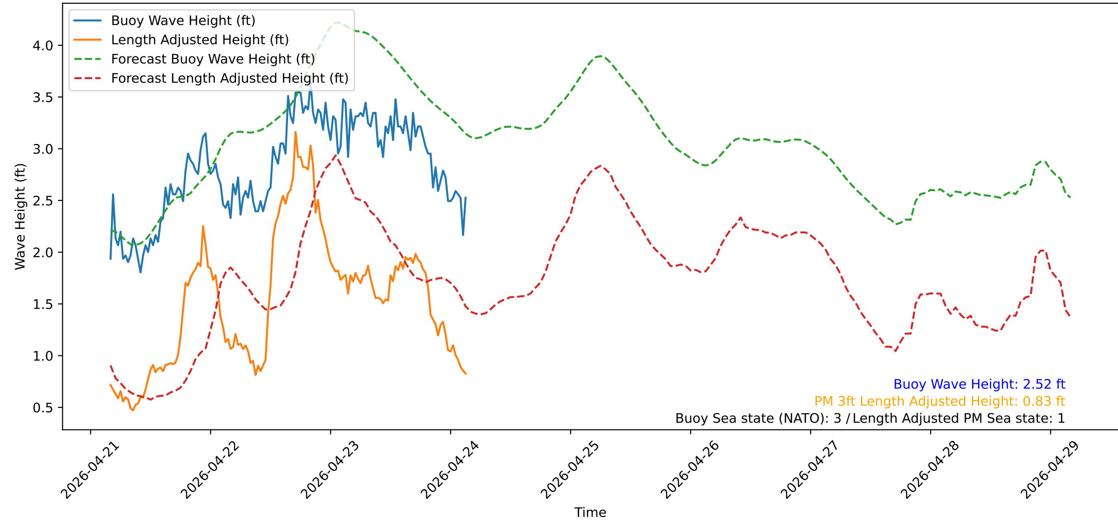
Wave Heights over Time for Red Beach at 2026-04-24 03:40:50
