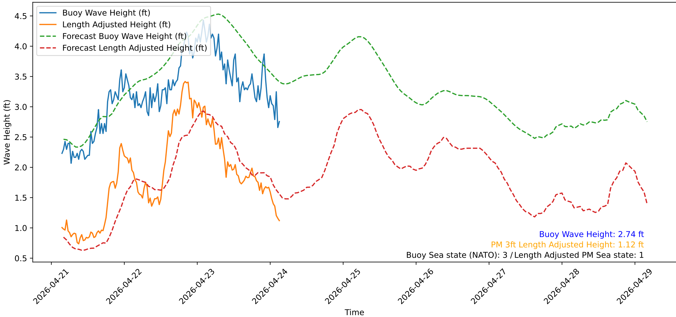
Wave Heights over Time for Oceanside Harbor at 2026-04-24 03:40:31
