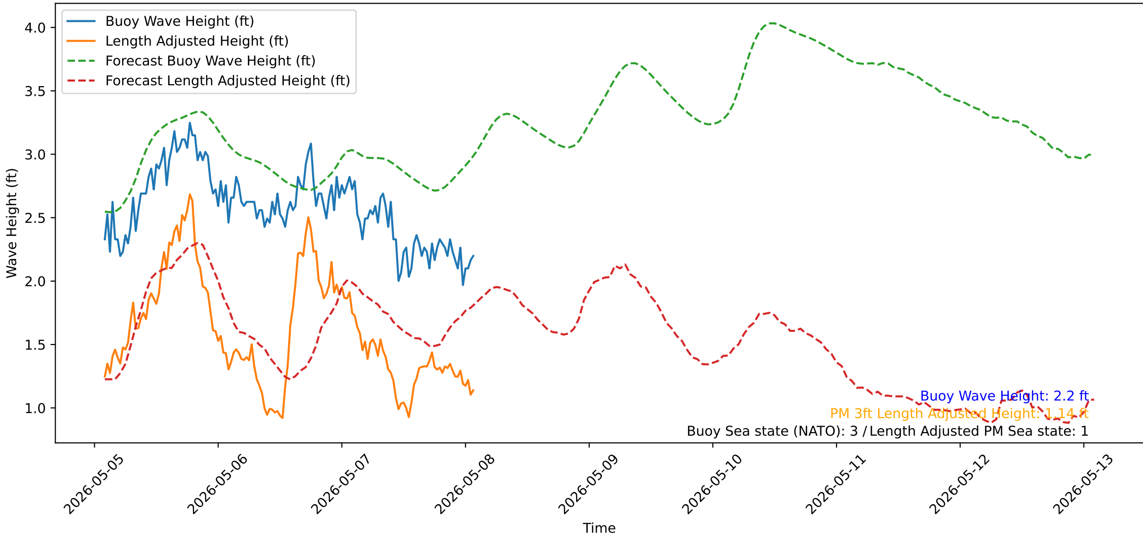
Wave Heights over Time for Oceanside Harbor at 2026-05-08 02:00:31
