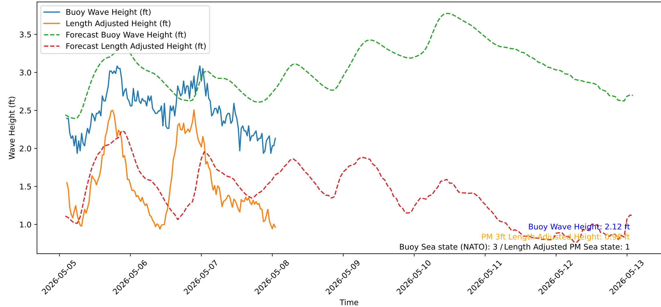
Wave Heights over Time for Red Beach at 2026-05-08 02:00:50
