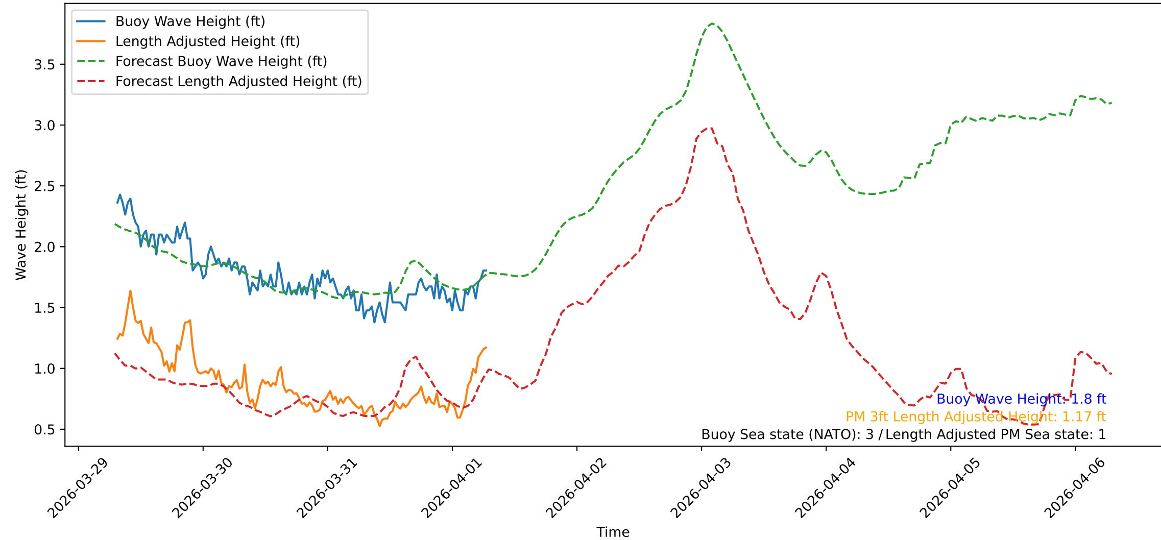
Wave Heights over Time for Red Beach at 2026-04-01 07:10:47
