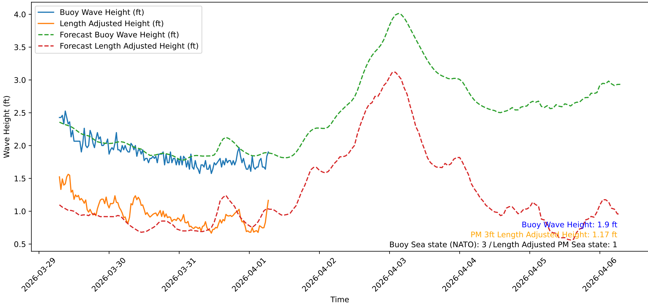
Wave Heights over Time for Oceanside Harbor at 2026-04-01 07:10:31
