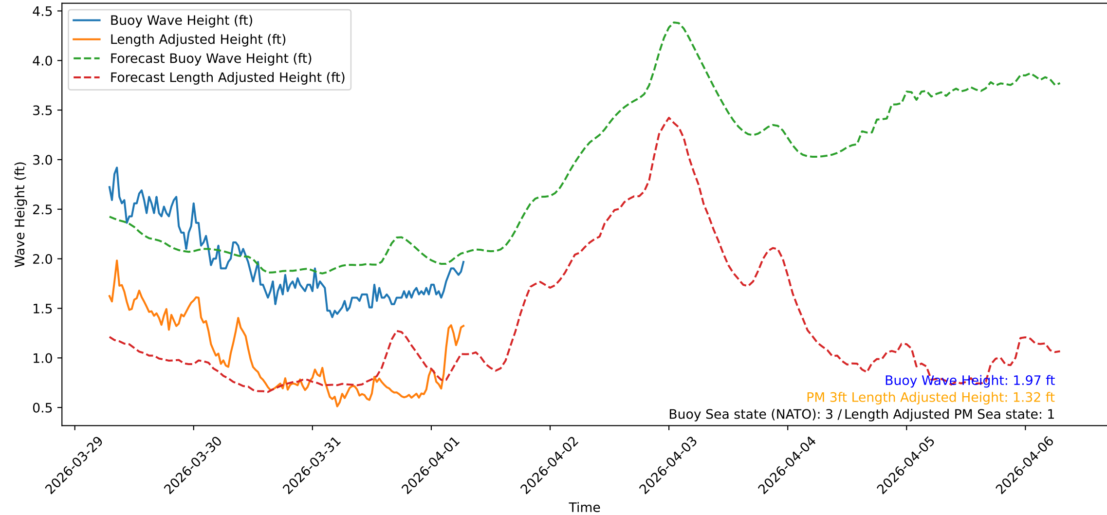
Wave Heights over Time for Green Beach at 2026-04-01 07:11:09
