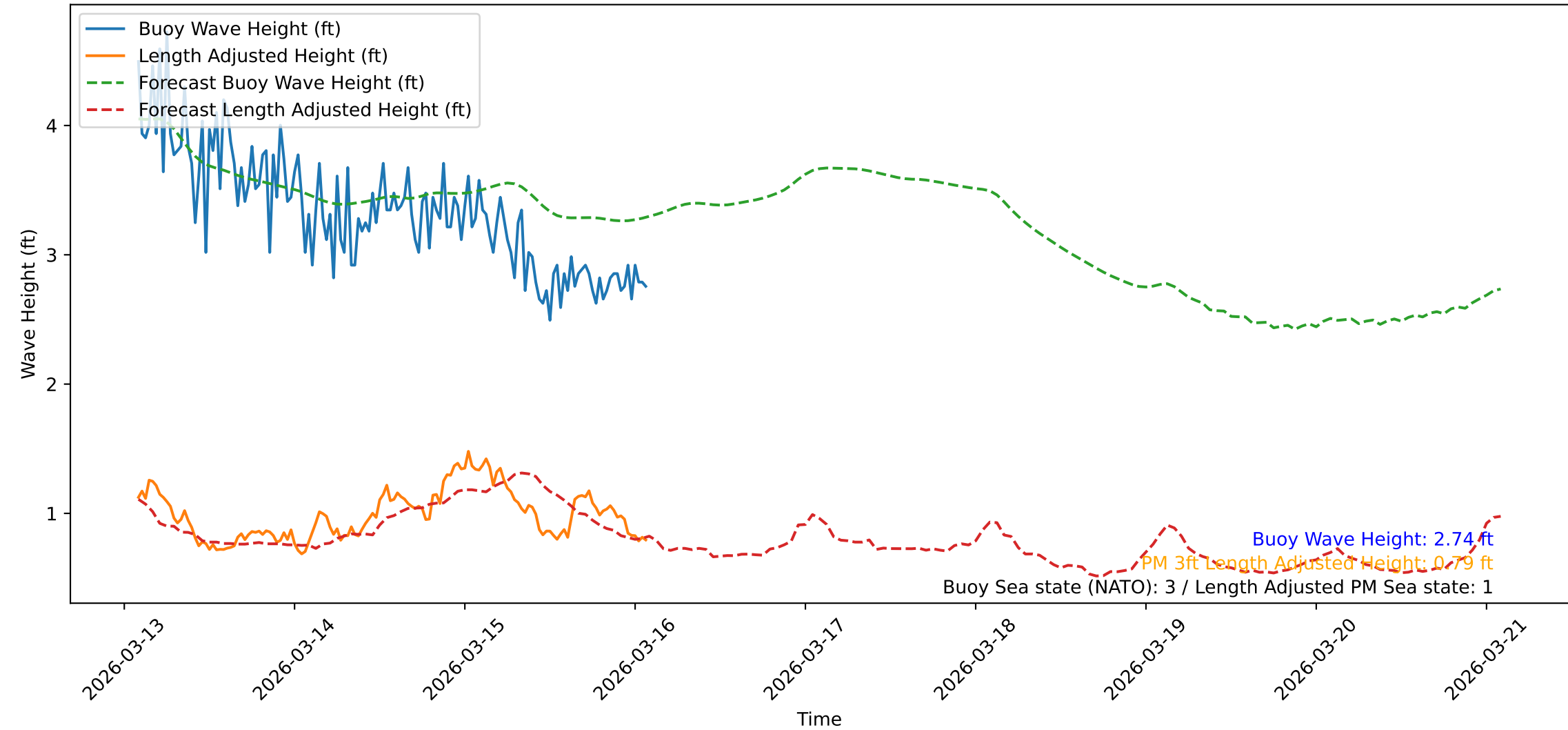
Wave Heights over Time for Oceanside Harbor at 2026-03-16 02:11:38
