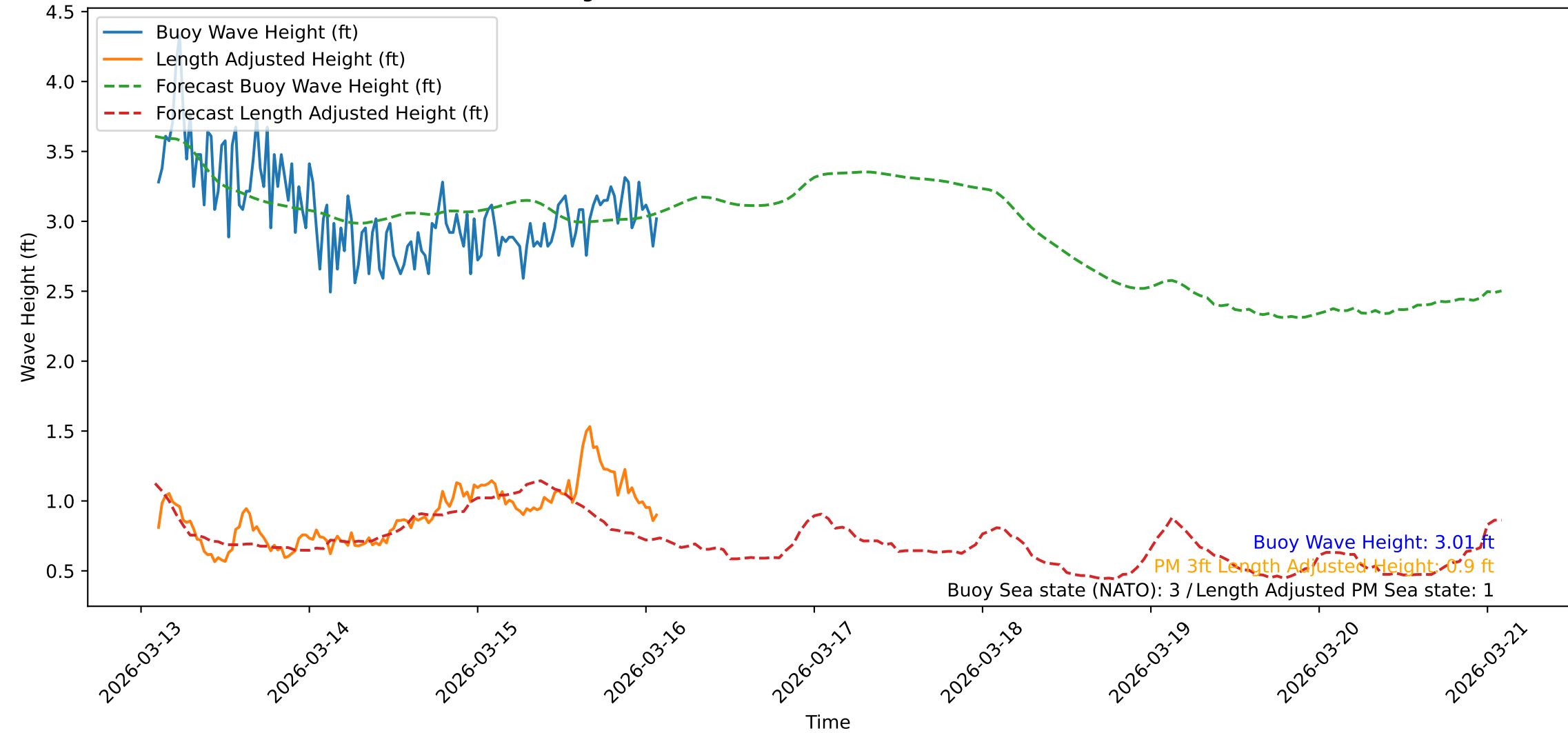
Wave Heights over Time for Red Beach at 2026-03-16 02:12:11
