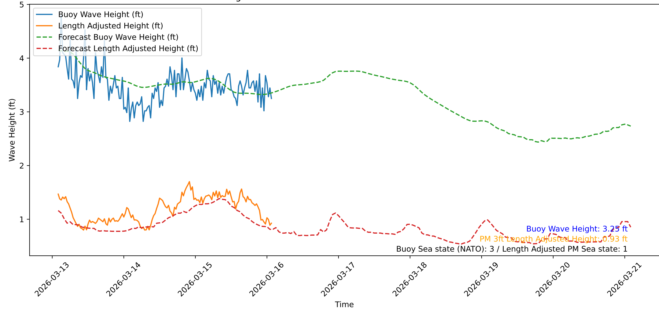
Wave Heights over Time for Green Beach at 2026-03-16 02:13:14
