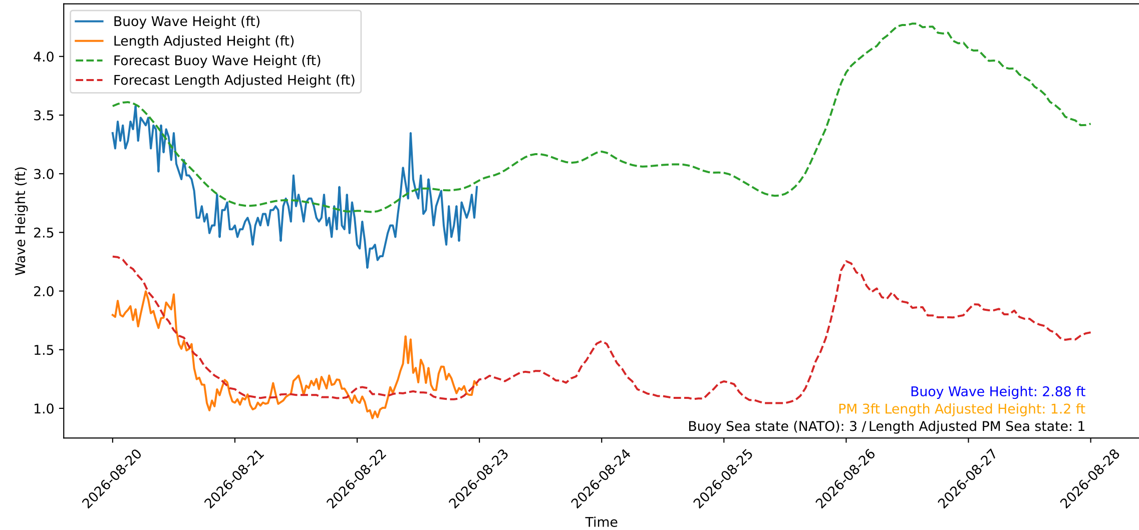
Wave Heights over Time for Oceanside Harbor at 2026-08-23 00:10:30
