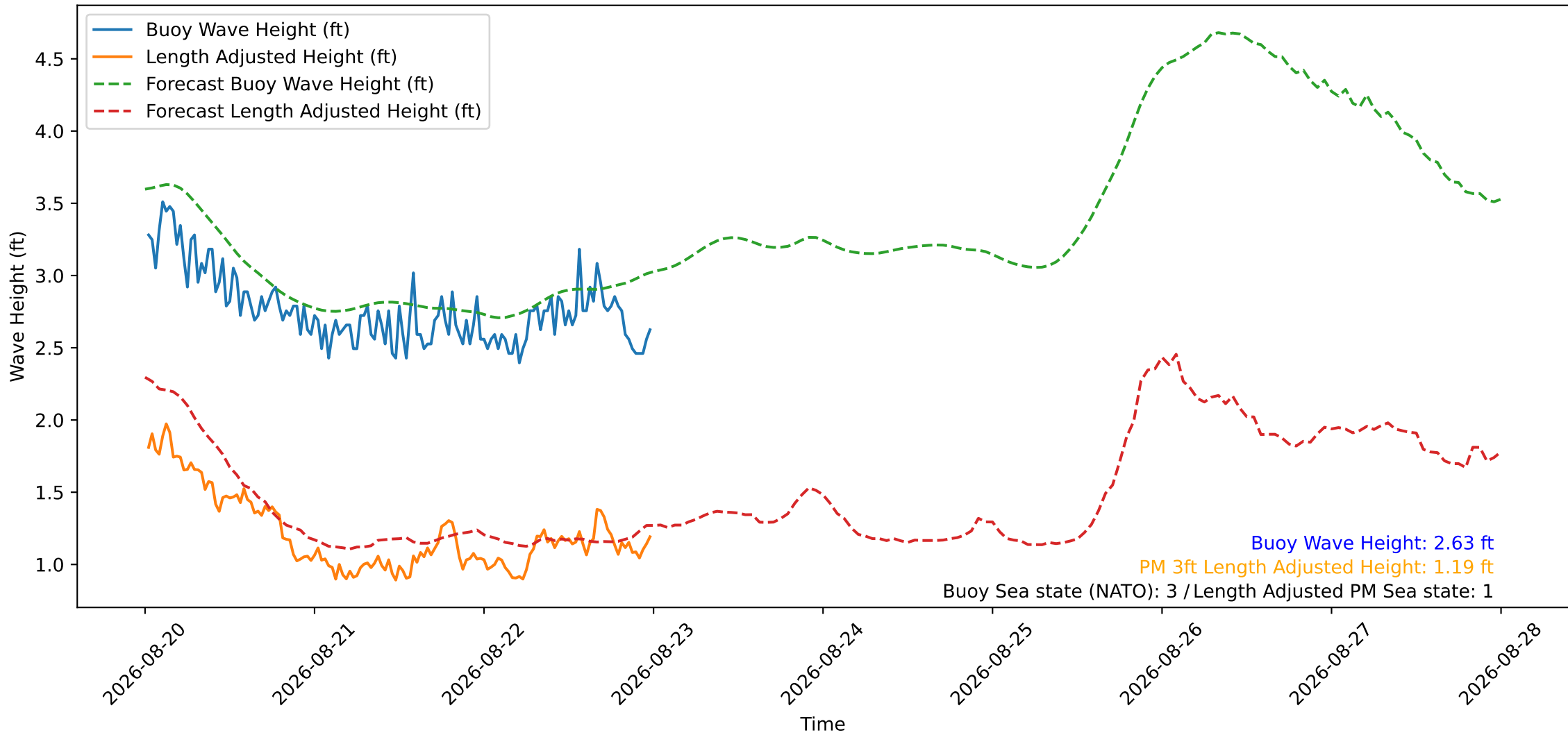
Wave Heights over Time for Green Beach at 2026-08-23 00:11:12
