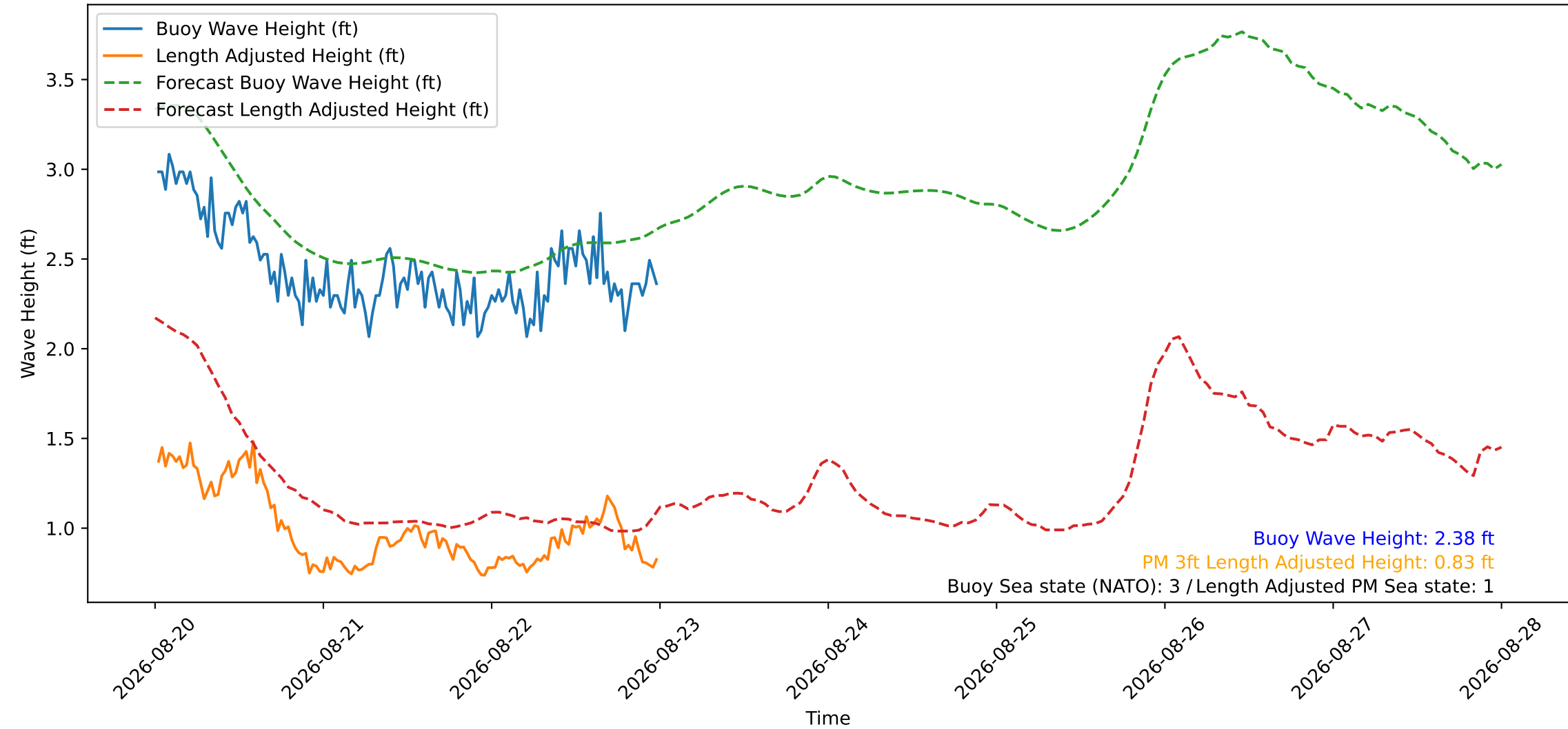
Wave Heights over Time for Red Beach at 2026-08-23 00:10:50
