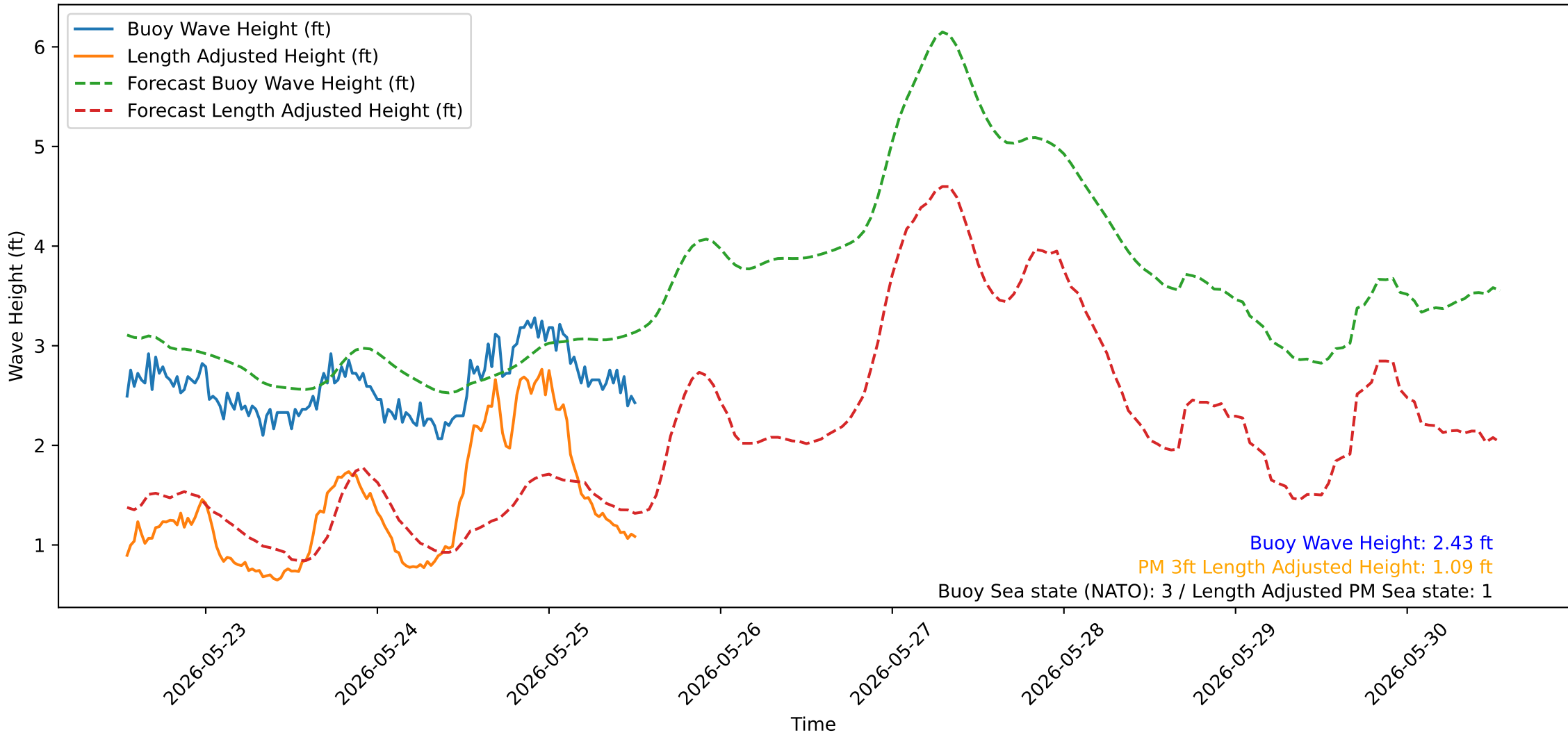
Wave Heights over Time for Green Beach at 2026-05-25 13:01:12
