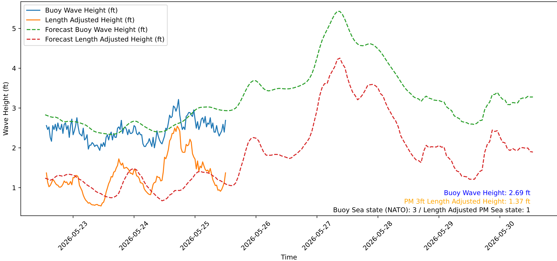
Wave Heights over Time for Red Beach at 2026-05-25 13:00:49
