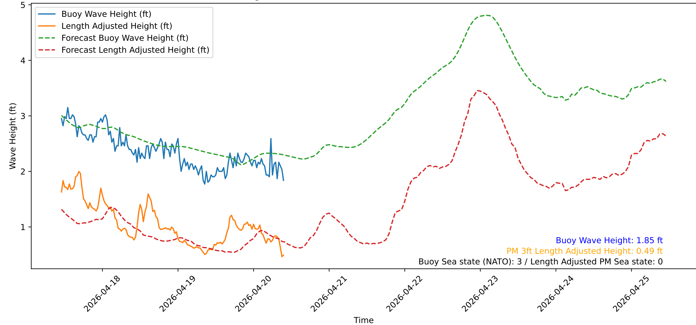
Wave Heights over Time for Red Beach at 2026-04-20 10:30:51
