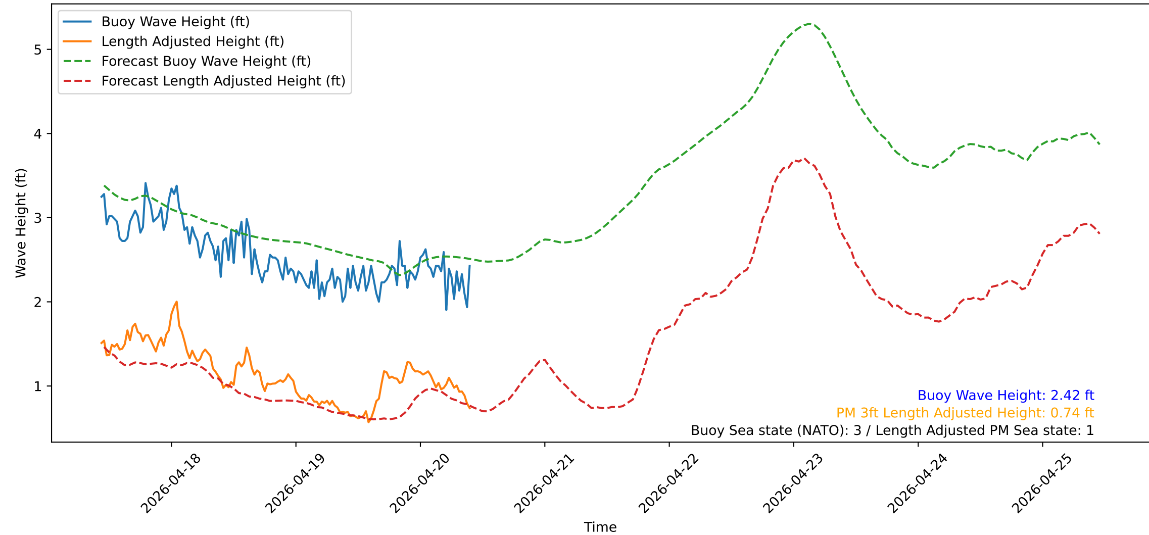
Wave Heights over Time for Oceanside Harbor at 2026-04-20 10:30:32
