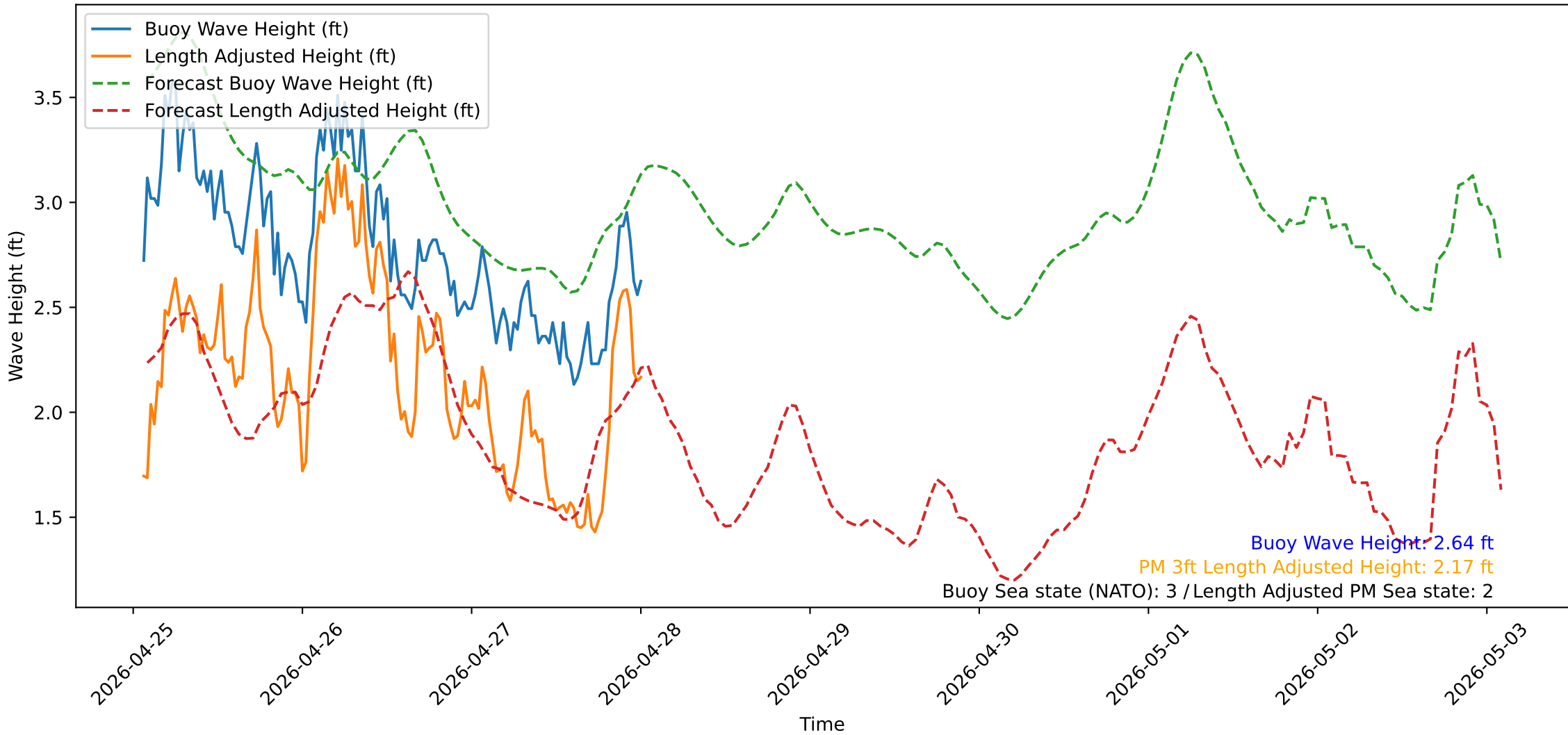
Wave Heights over Time for Green Beach at 2026-04-28 01:31:12
