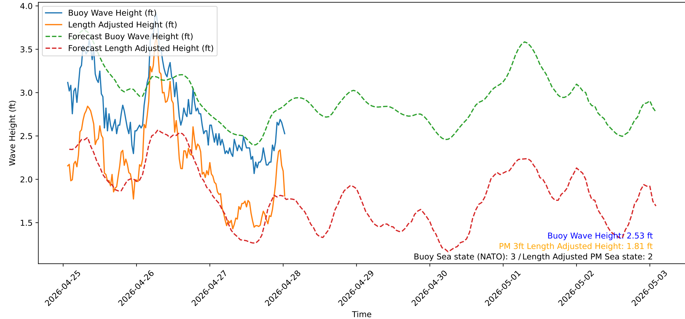
Wave Heights over Time for Oceanside Harbor at 2026-04-28 01:30:31
