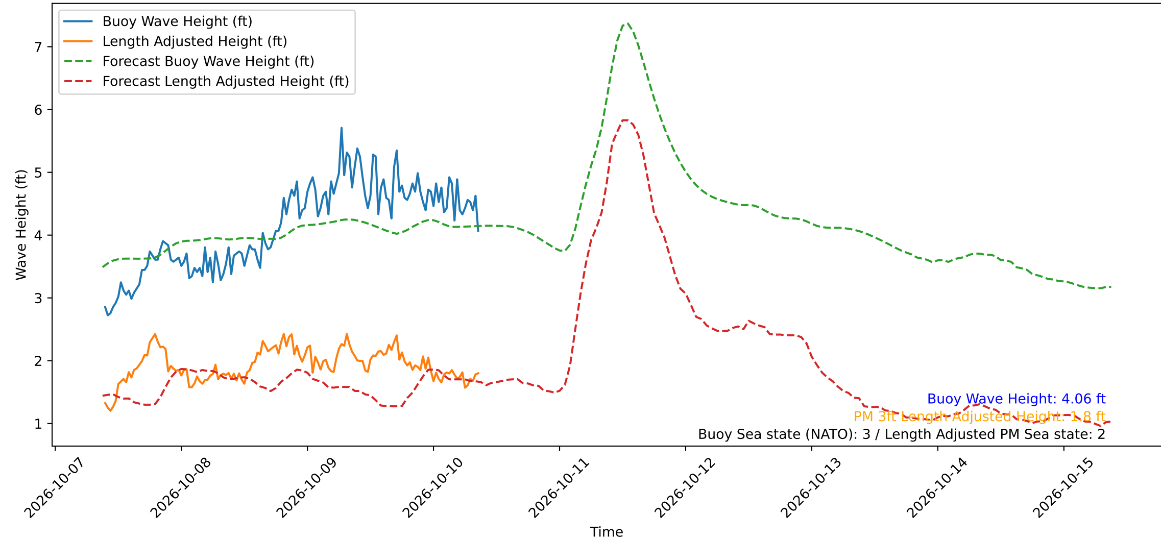
Wave Heights over Time for Red Beach at 2026-10-10 09:10:49
