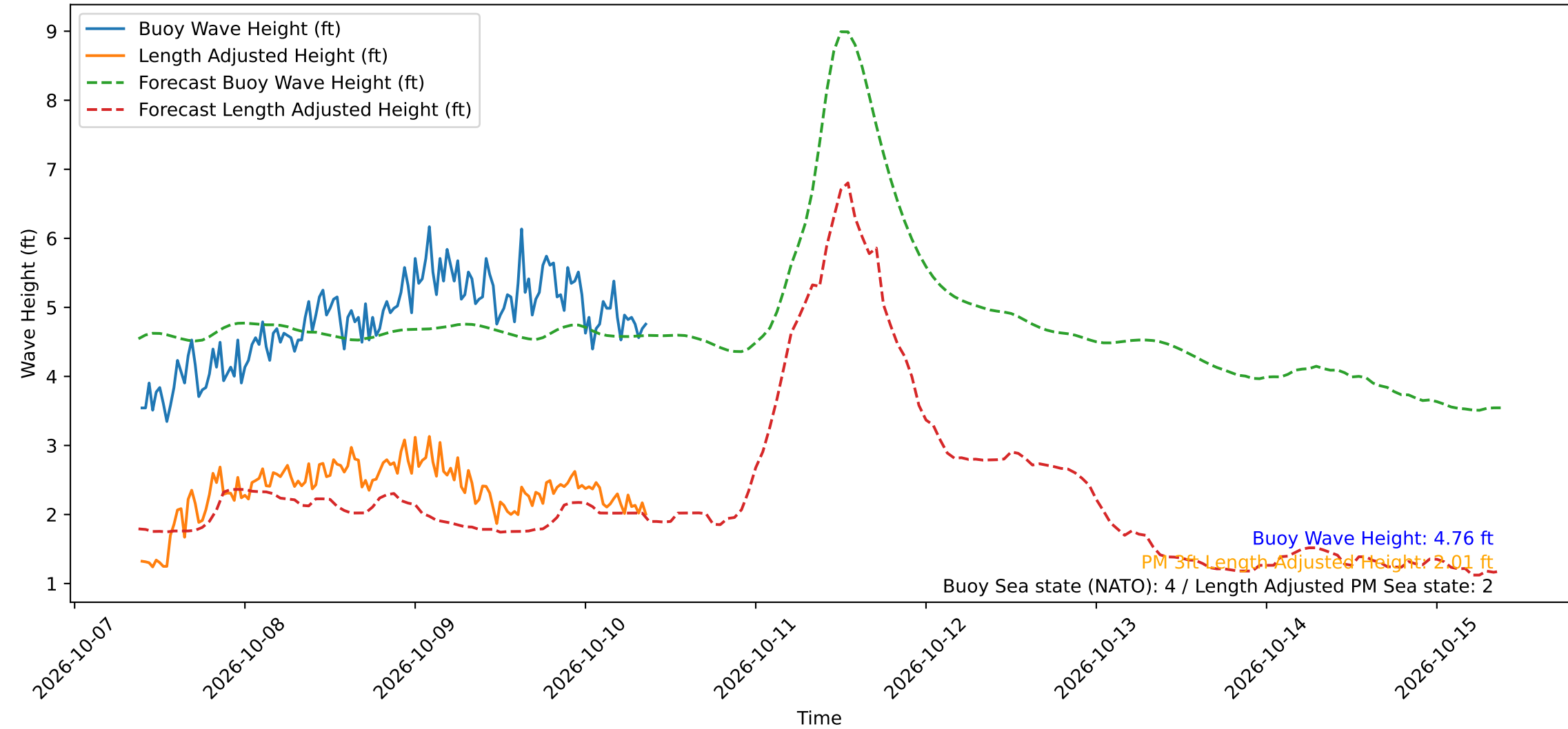
Wave Heights over Time for Green Beach at 2026-10-10 09:11:12
