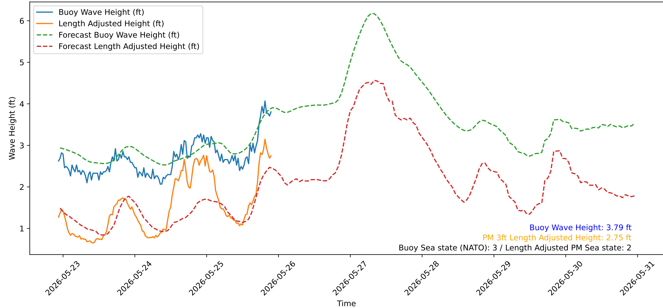
Wave Heights over Time for Green Beach at 2026-05-25 22:31:11
