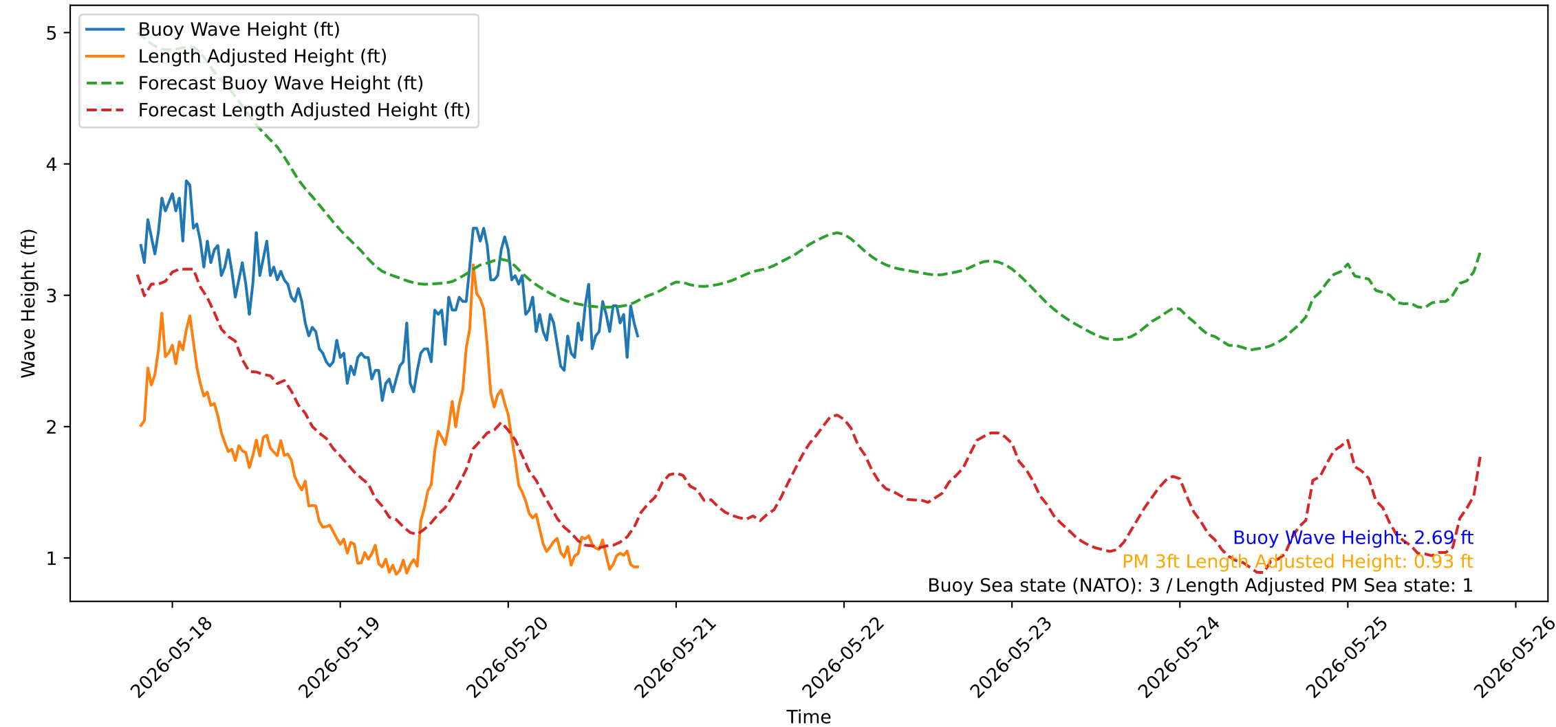
Wave Heights over Time for Oceanside Harbor at 2026-05-20 19:20:32
