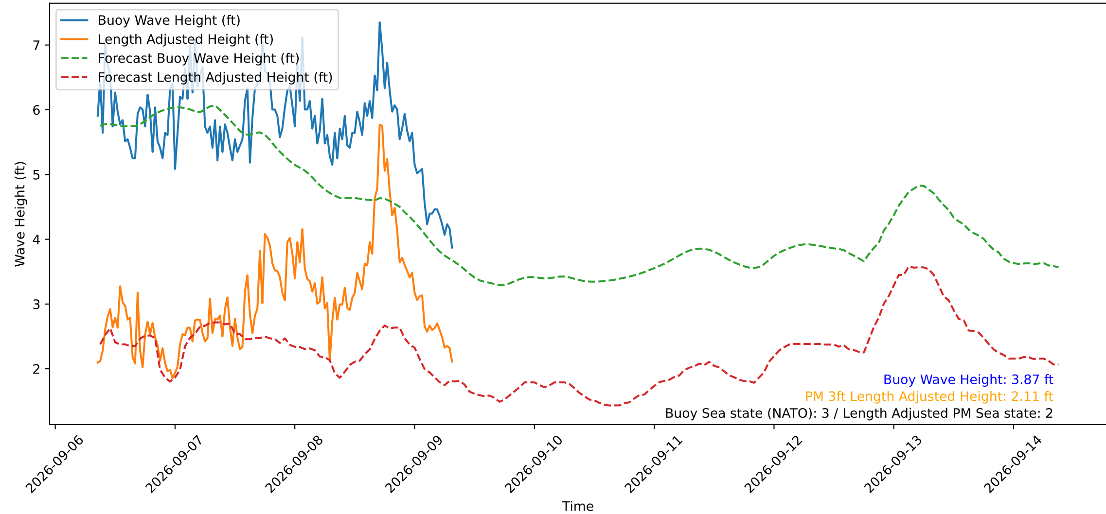
Wave Heights over Time for Oceanside Harbor at 2026-09-09 08:30:30
