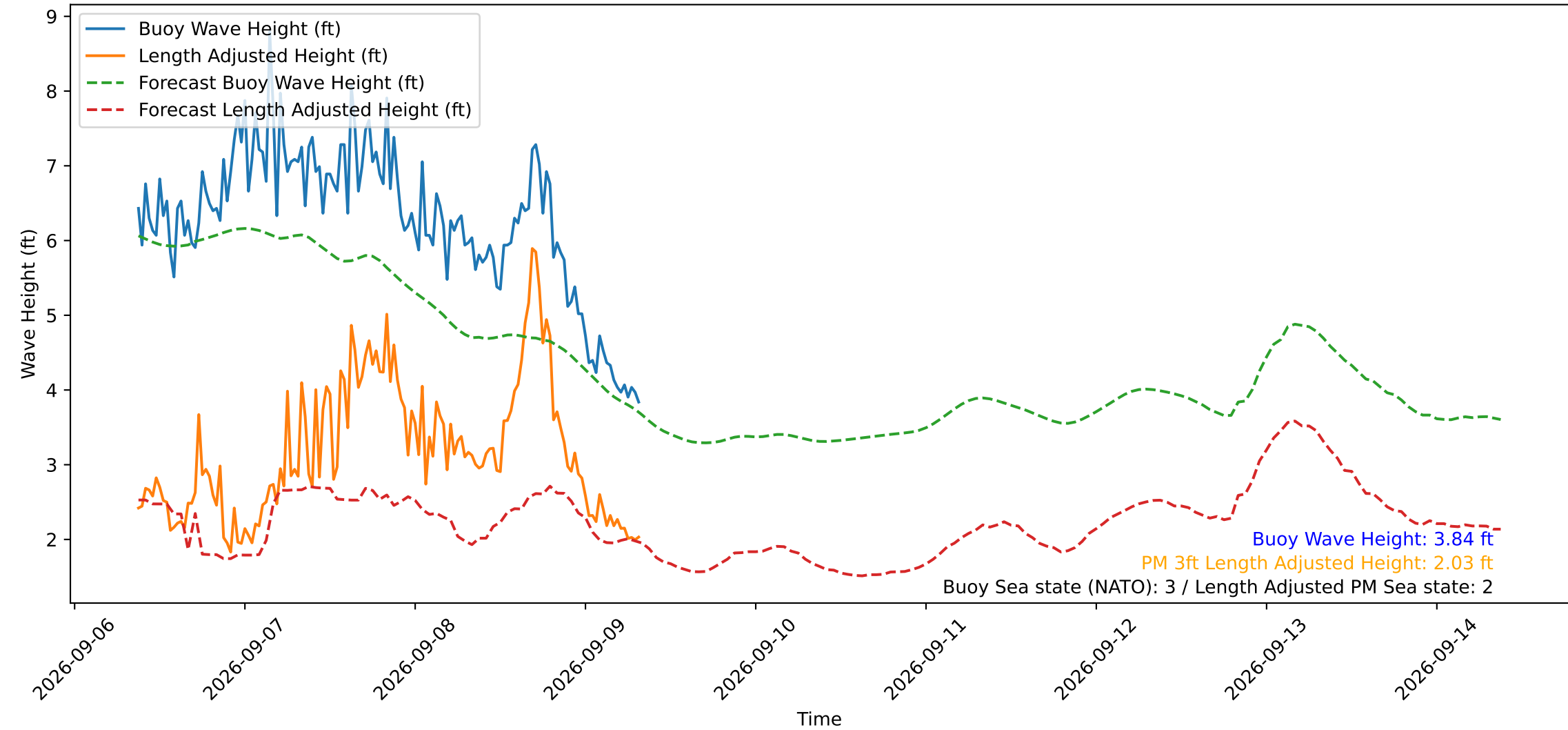
Wave Heights over Time for Green Beach at 2026-09-09 08:31:11
