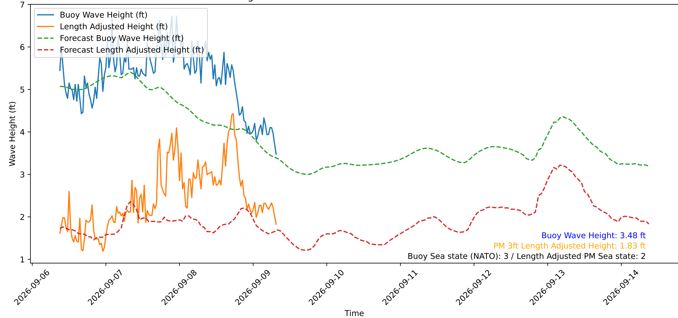
Wave Heights over Time for Red Beach at 2026-09-09 08:30:49
