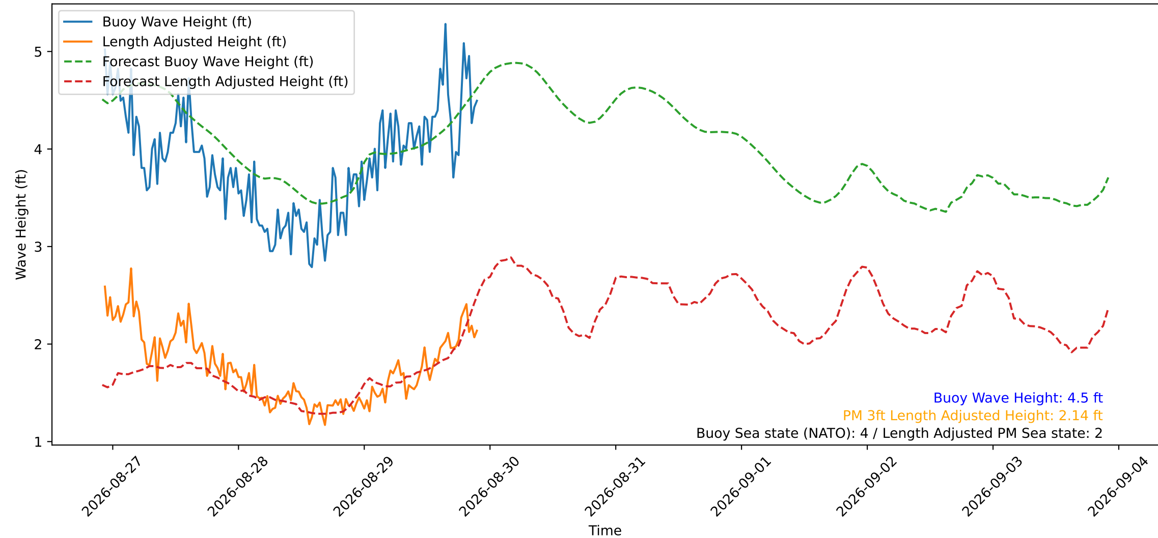
Wave Heights over Time for Oceanside Harbor at 2026-08-29 22:20:30
