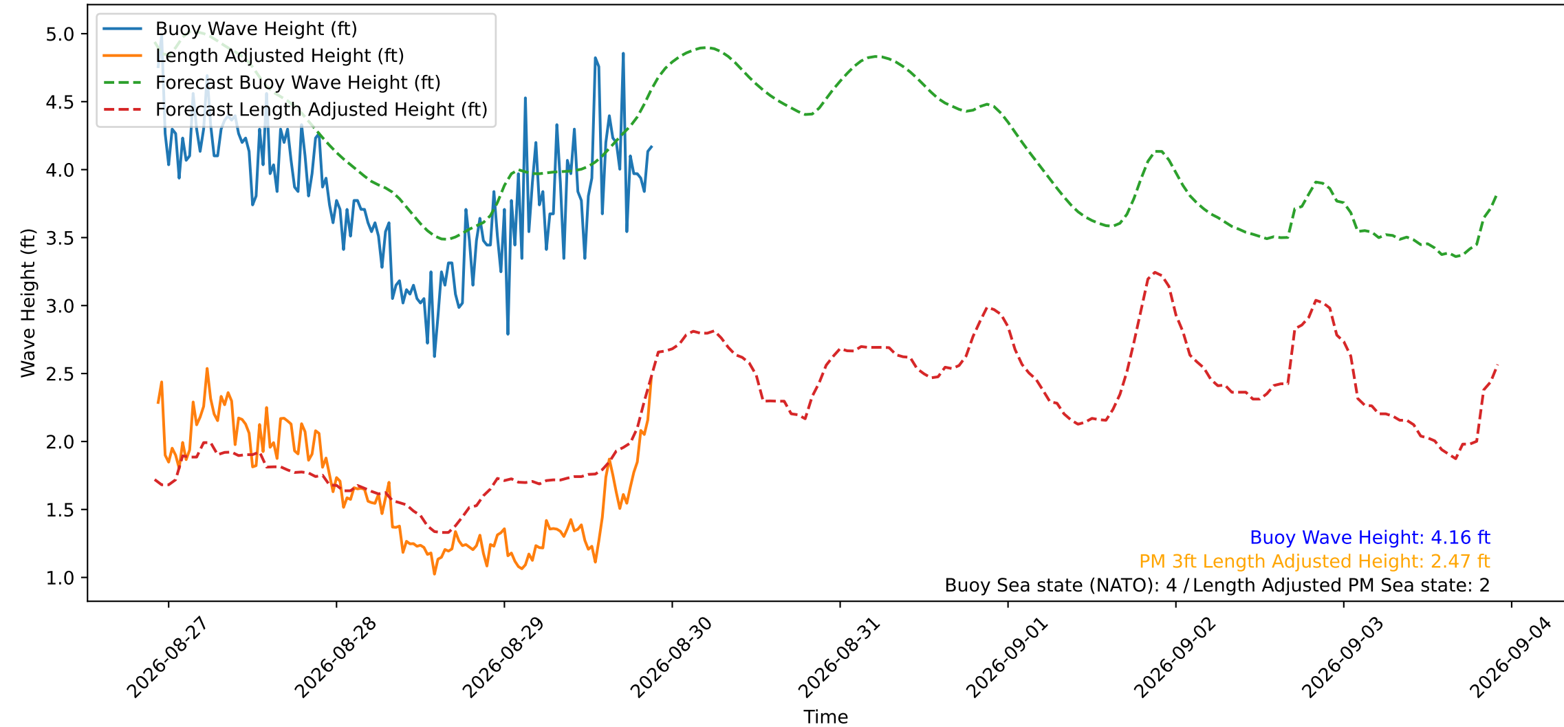
Wave Heights over Time for Green Beach at 2026-08-29 22:21:15
