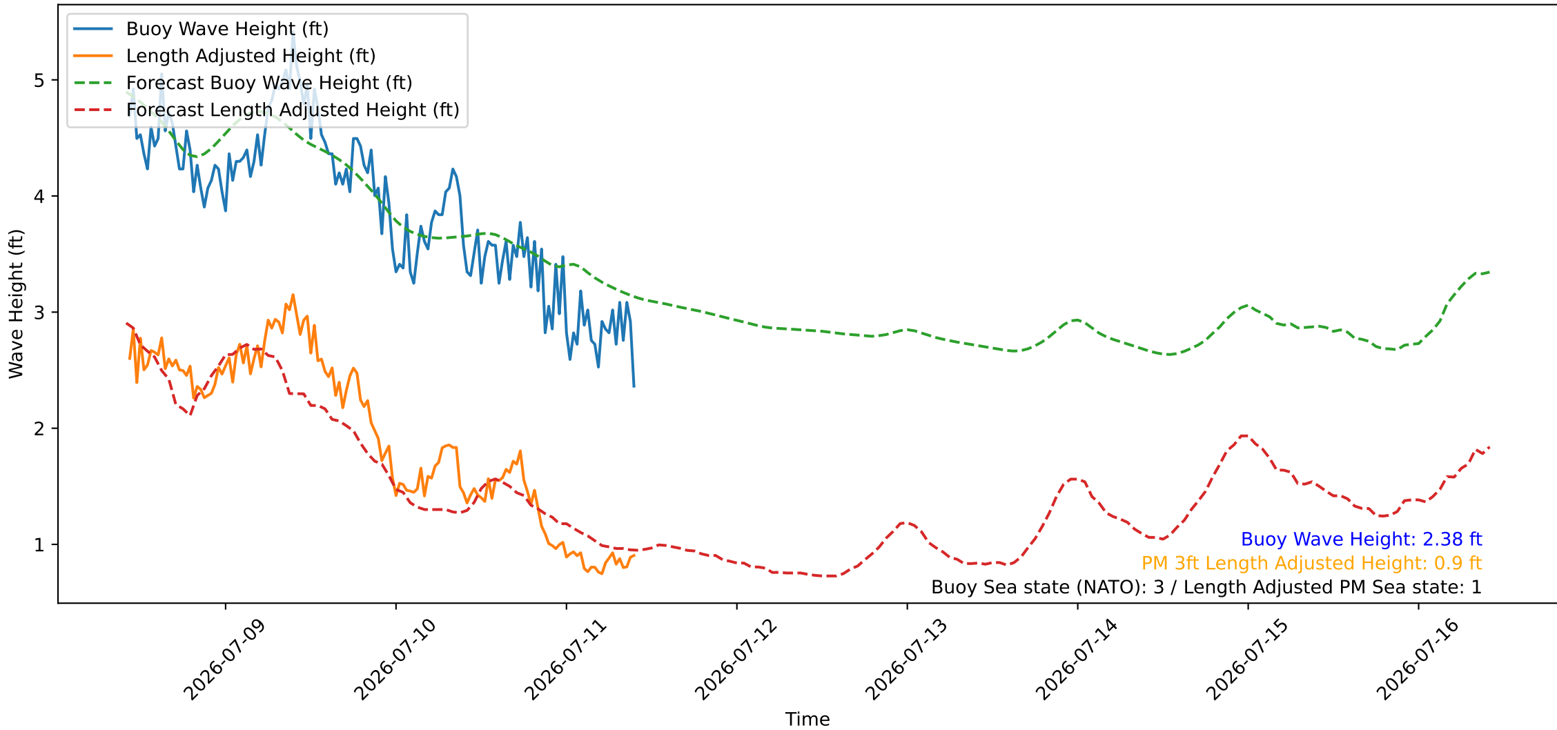
Wave Heights over Time for Oceanside Harbor at 2026-07-11 10:20:26
