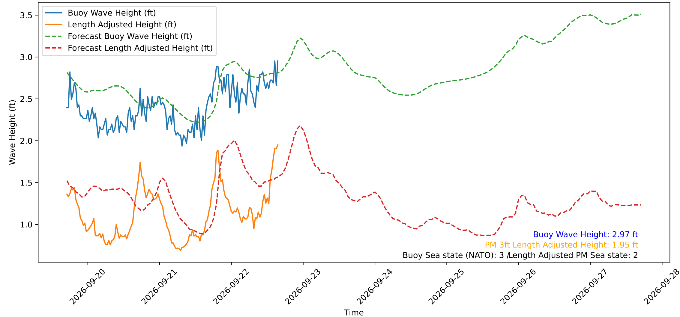
Wave Heights over Time for Red Beach at 2026-09-22 16:30:49
