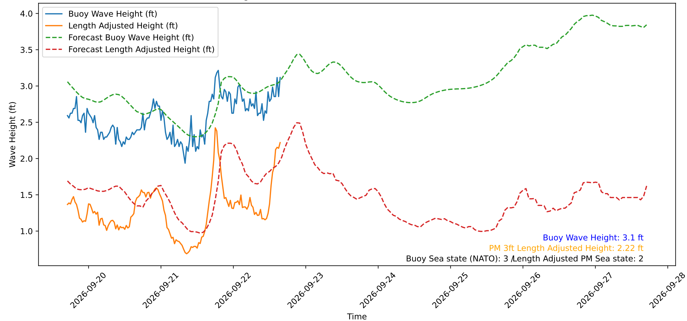
Wave Heights over Time for Green Beach at 2026-09-22 16:31:12
