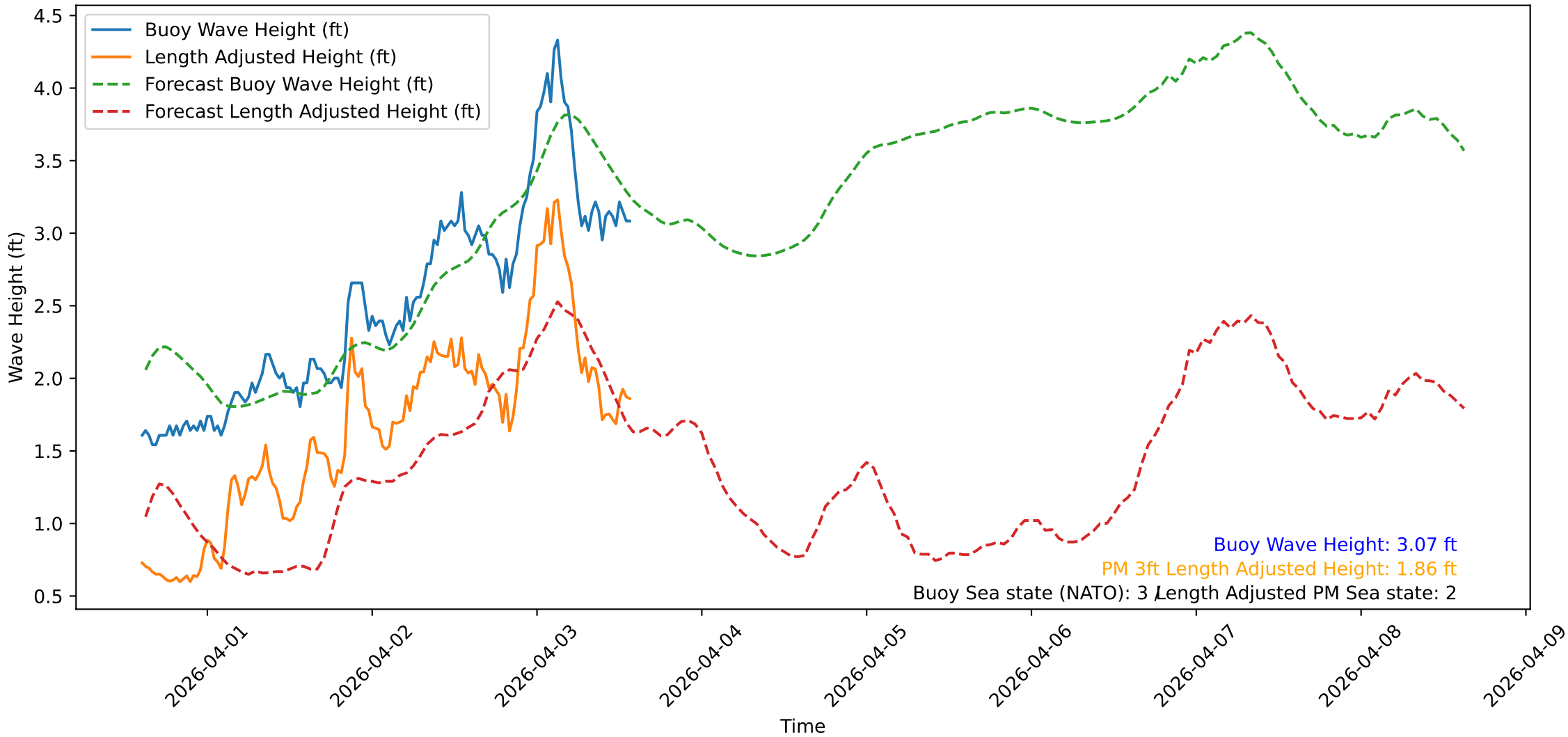
Wave Heights over Time for Green Beach at 2026-04-03 14:31:12
