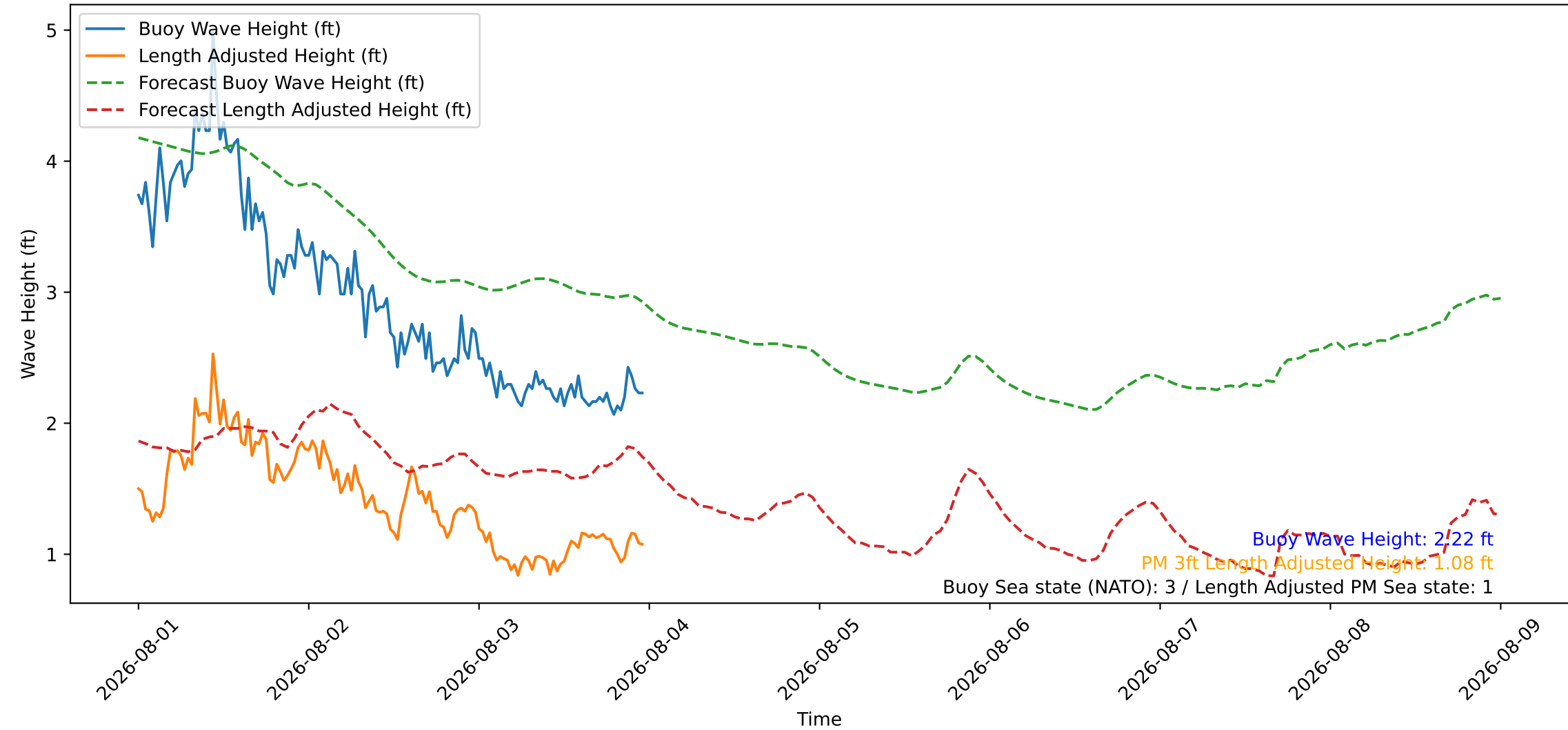
Wave Heights over Time for Green Beach at 2026-08-04 00:01:08
