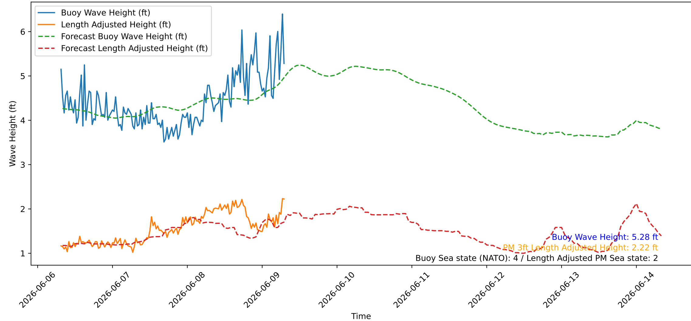
Wave Heights over Time for Oceanside Harbor at 2026-06-09 07:40:26
