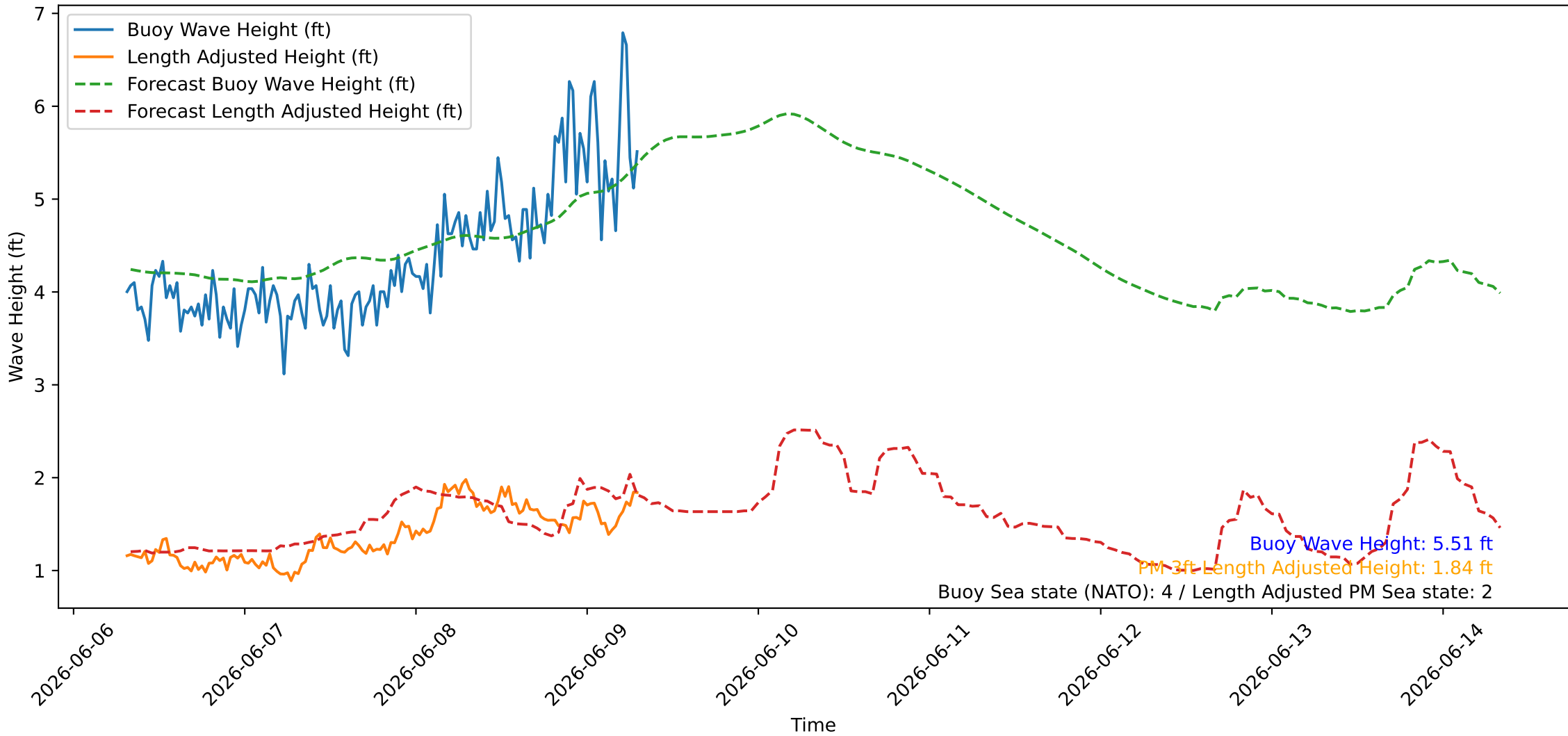
Wave Heights over Time for Green Beach at 2026-06-09 07:41:08
