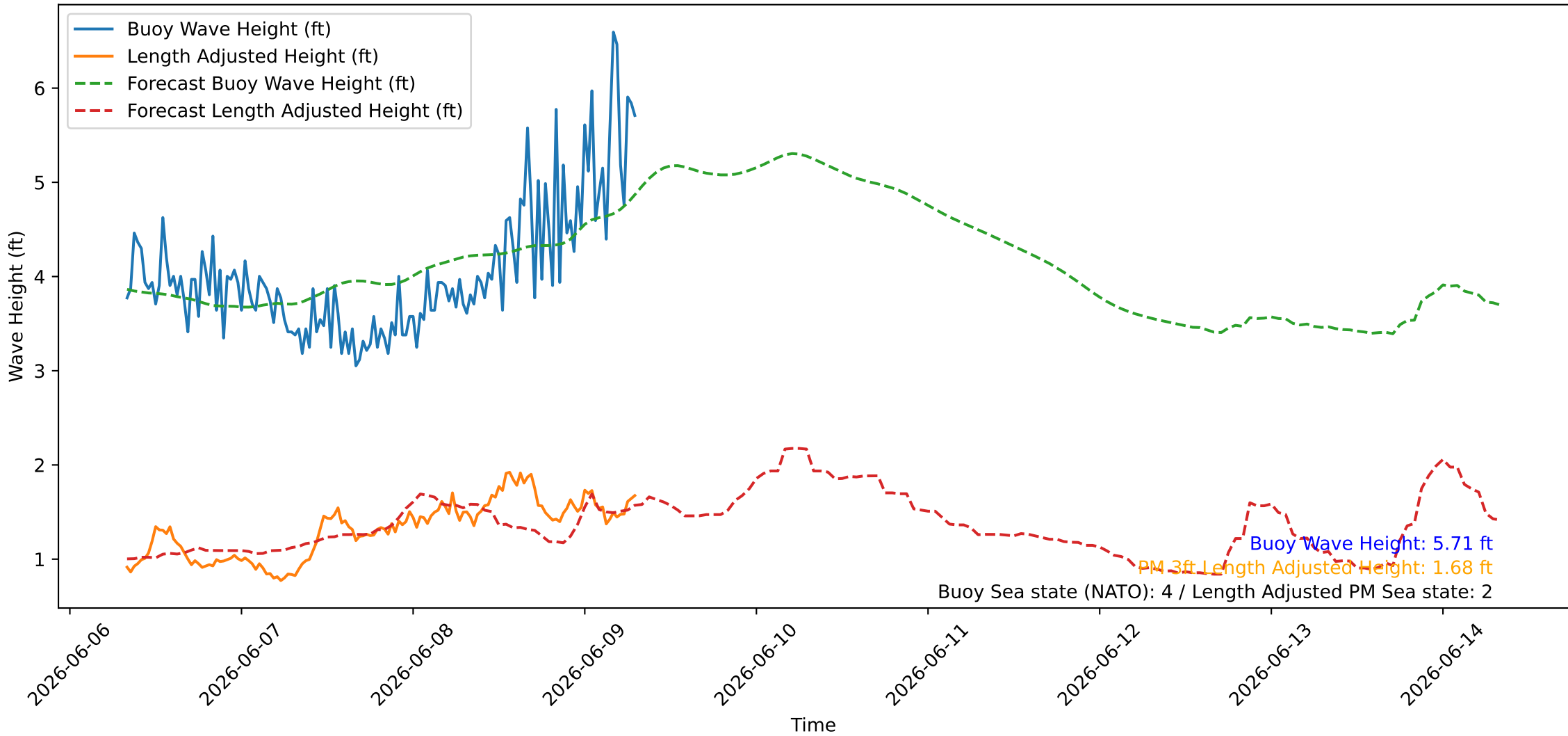
Wave Heights over Time for Red Beach at 2026-06-09 07:40:45
