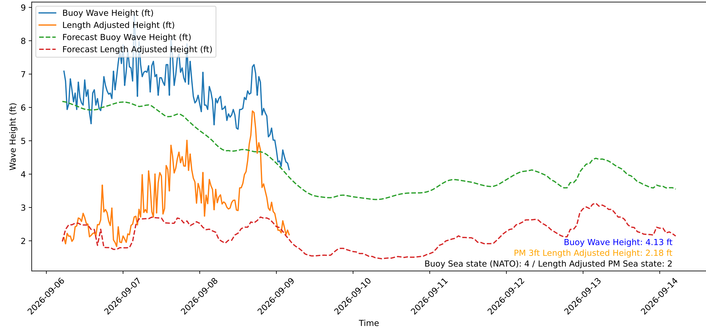
Wave Heights over Time for Green Beach at 2026-09-09 05:01:11
