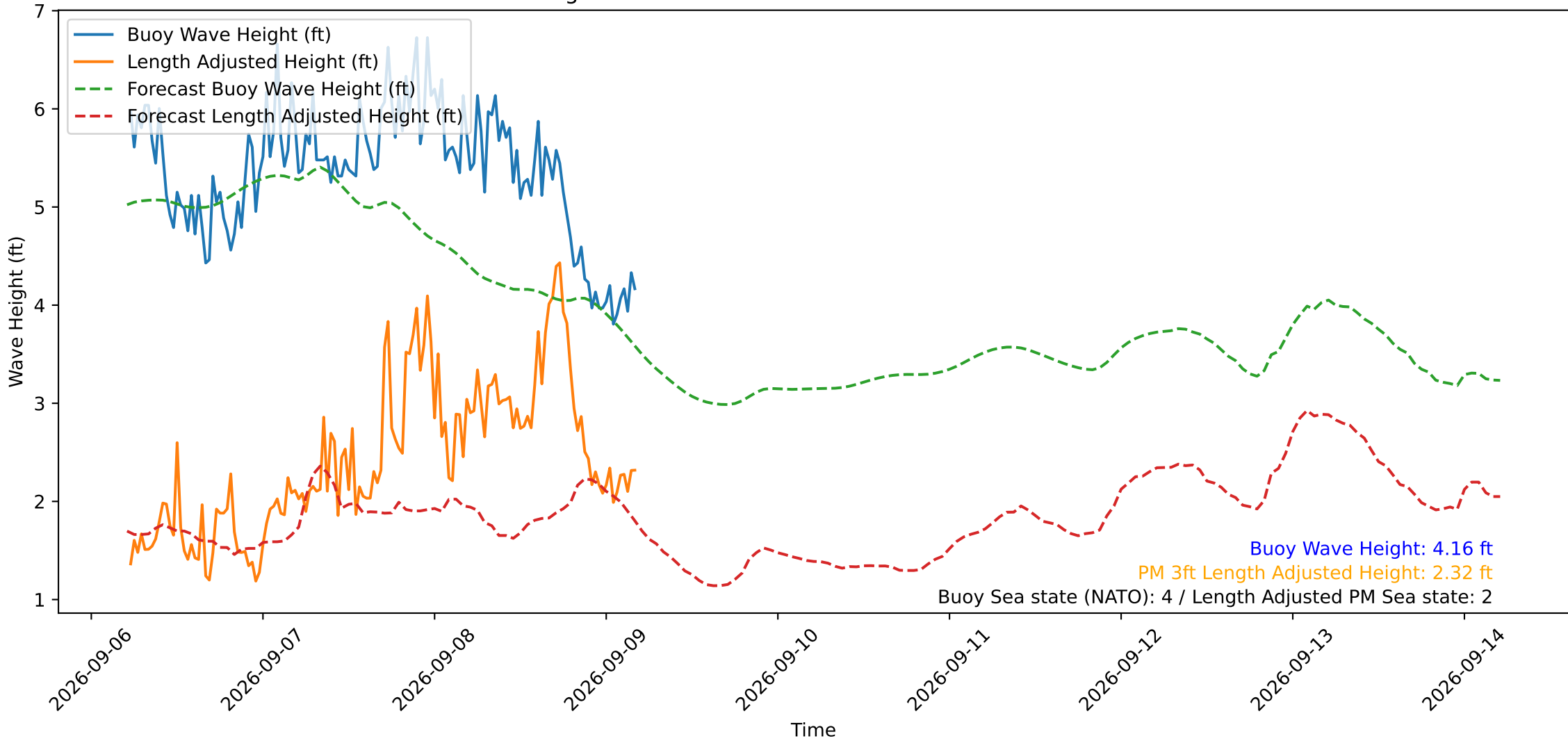
Wave Heights over Time for Red Beach at 2026-09-09 05:00:49
