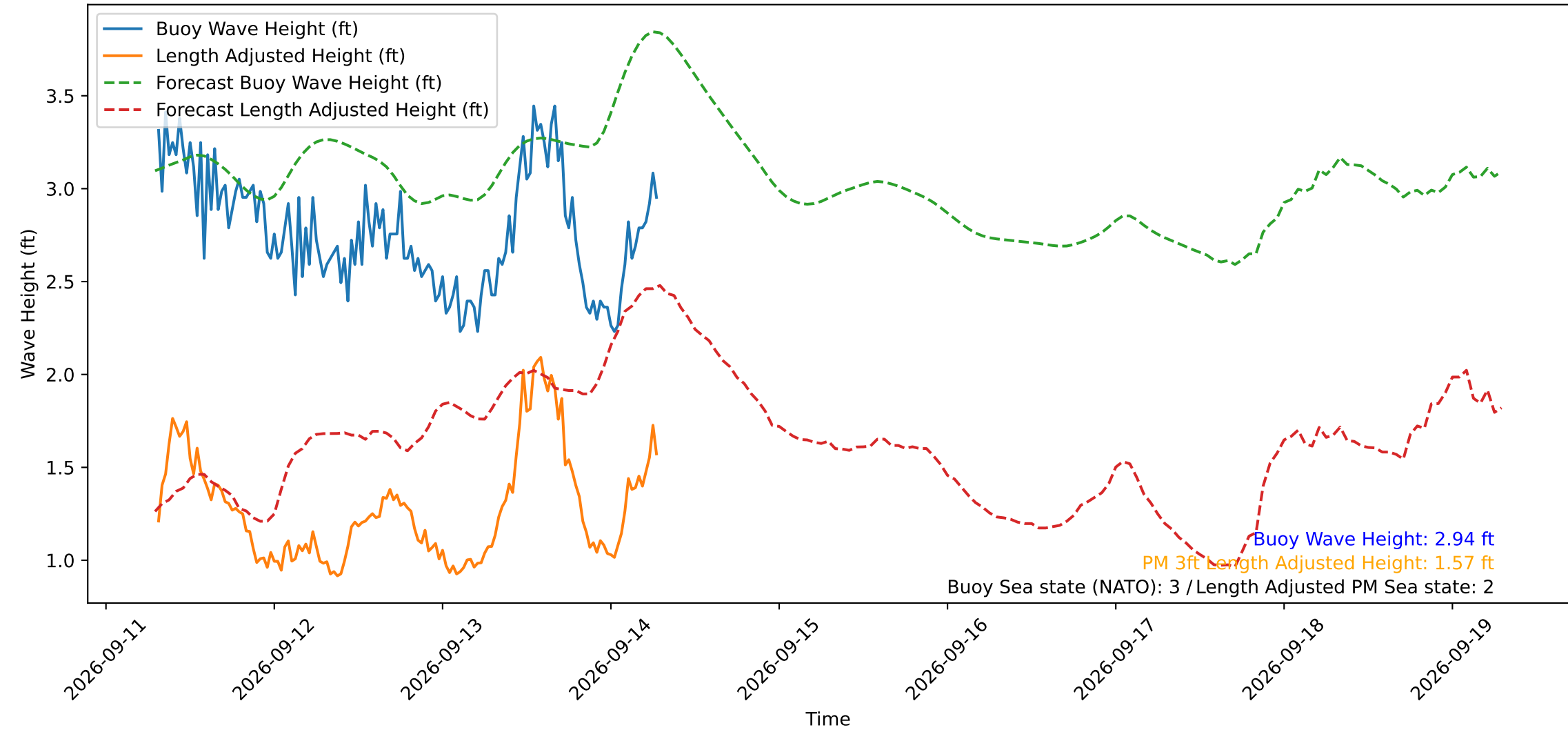
Wave Heights over Time for Red Beach at 2026-09-14 07:10:50
