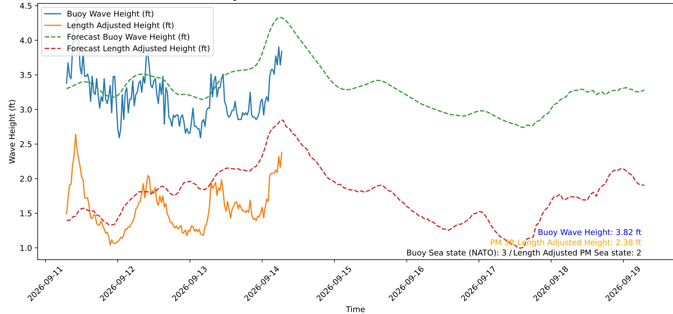
Wave Heights over Time for Oceanside Harbor at 2026-09-14 07:10:30
