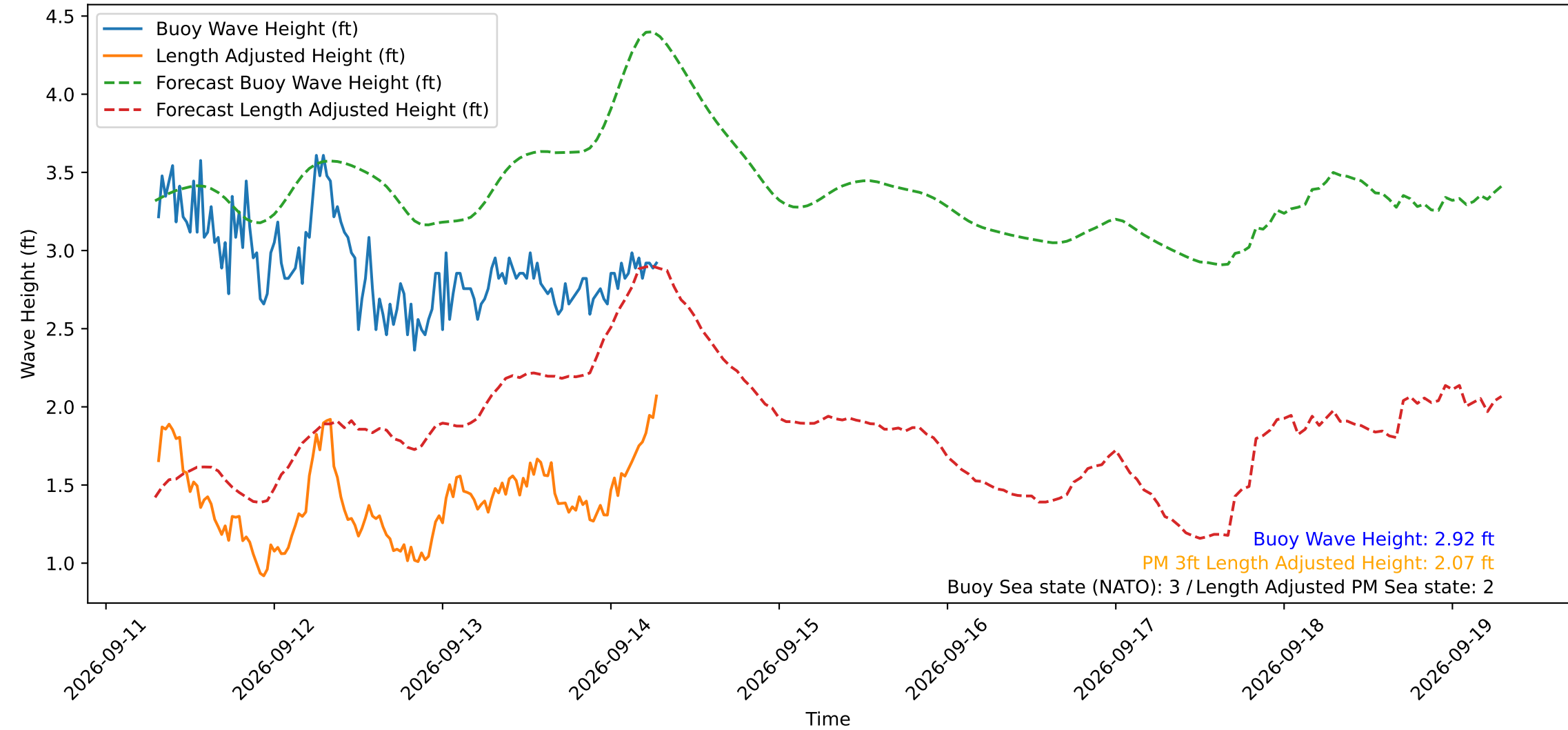
Wave Heights over Time for Green Beach at 2026-09-14 07:11:14
