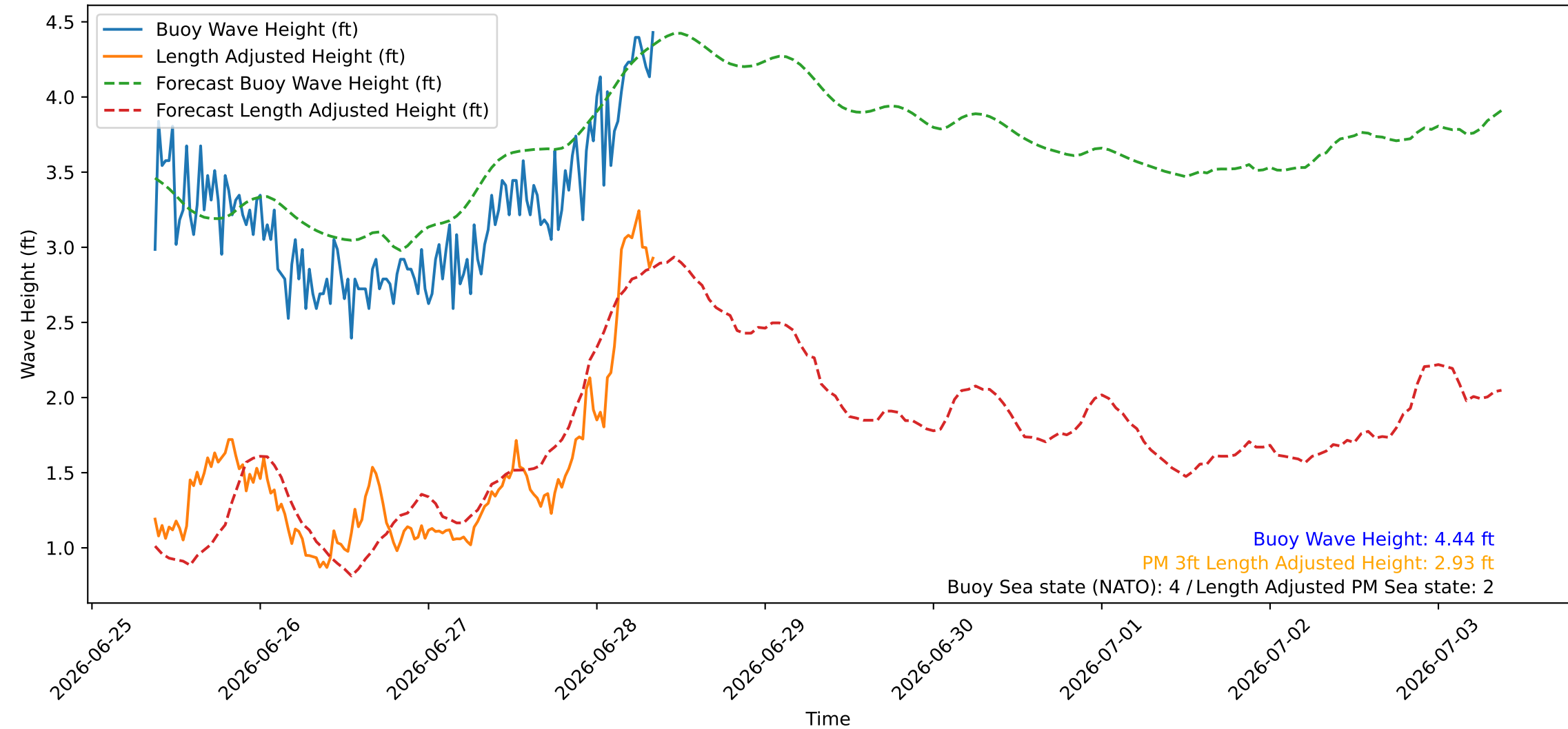
Wave Heights over Time for Oceanside Harbor at 2026-06-28 08:50:26
