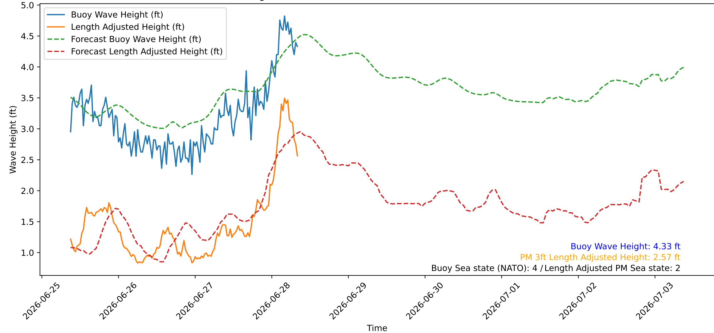
Wave Heights over Time for Green Beach at 2026-06-28 08:51:09
