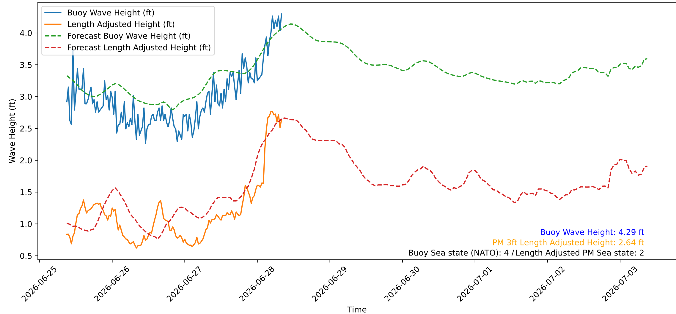
Wave Heights over Time for Red Beach at 2026-06-28 08:50:46
