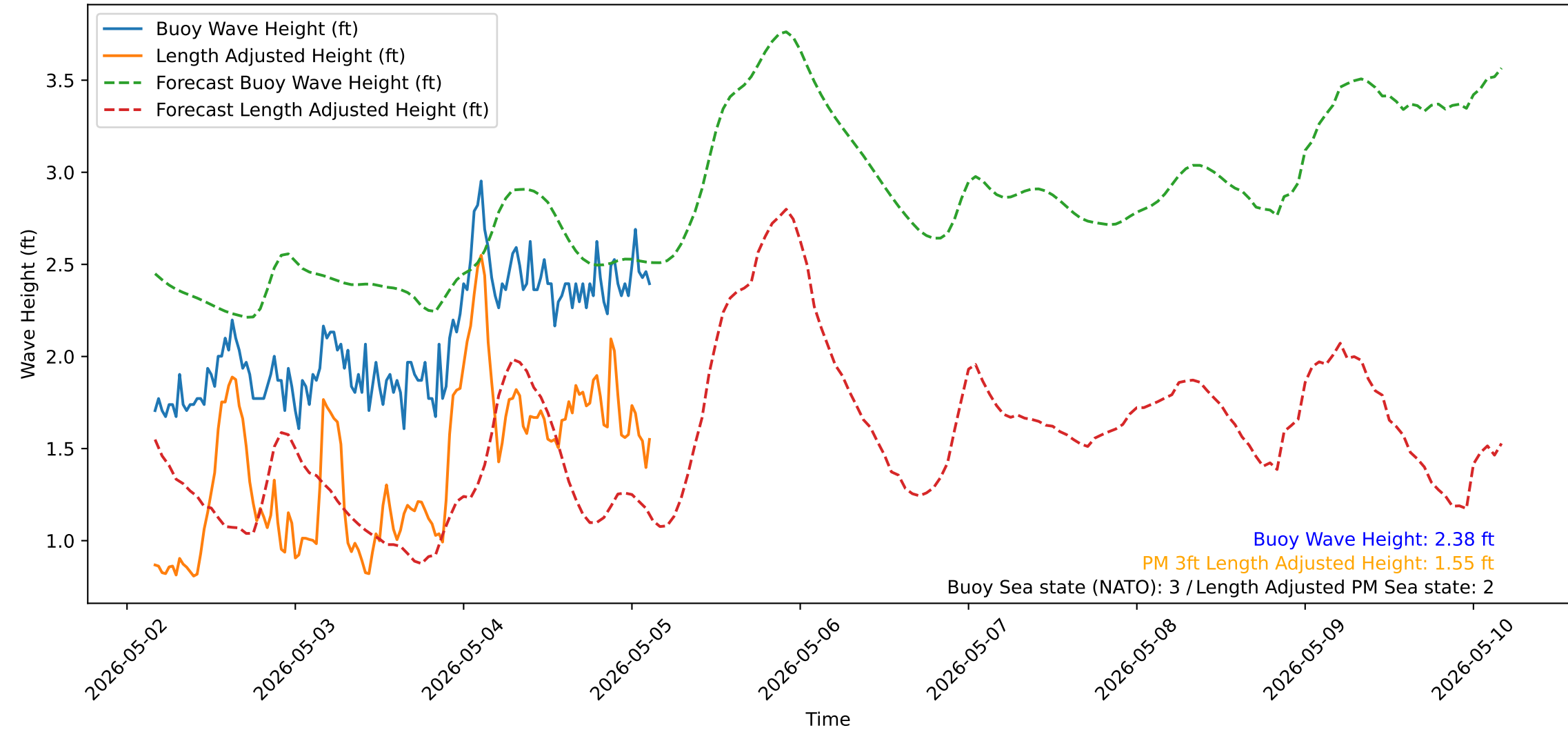
Wave Heights over Time for Red Beach at 2026-05-05 03:30:50
