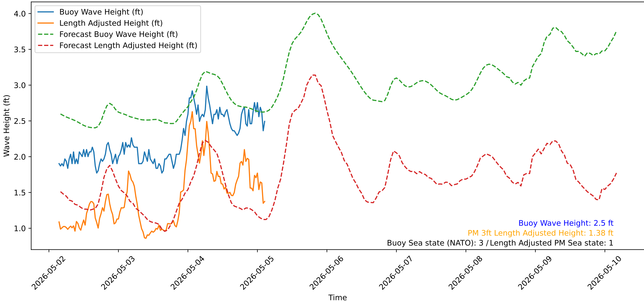
Wave Heights over Time for Green Beach at 2026-05-05 03:31:12
