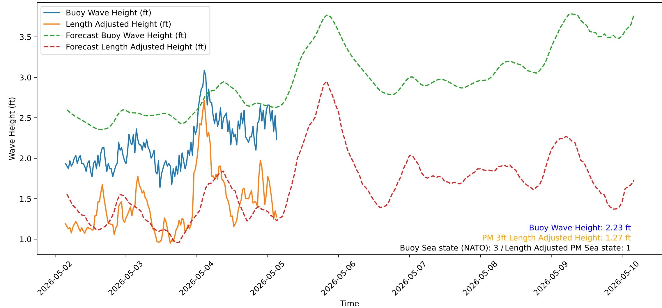
Wave Heights over Time for Oceanside Harbor at 2026-05-05 03:30:31
