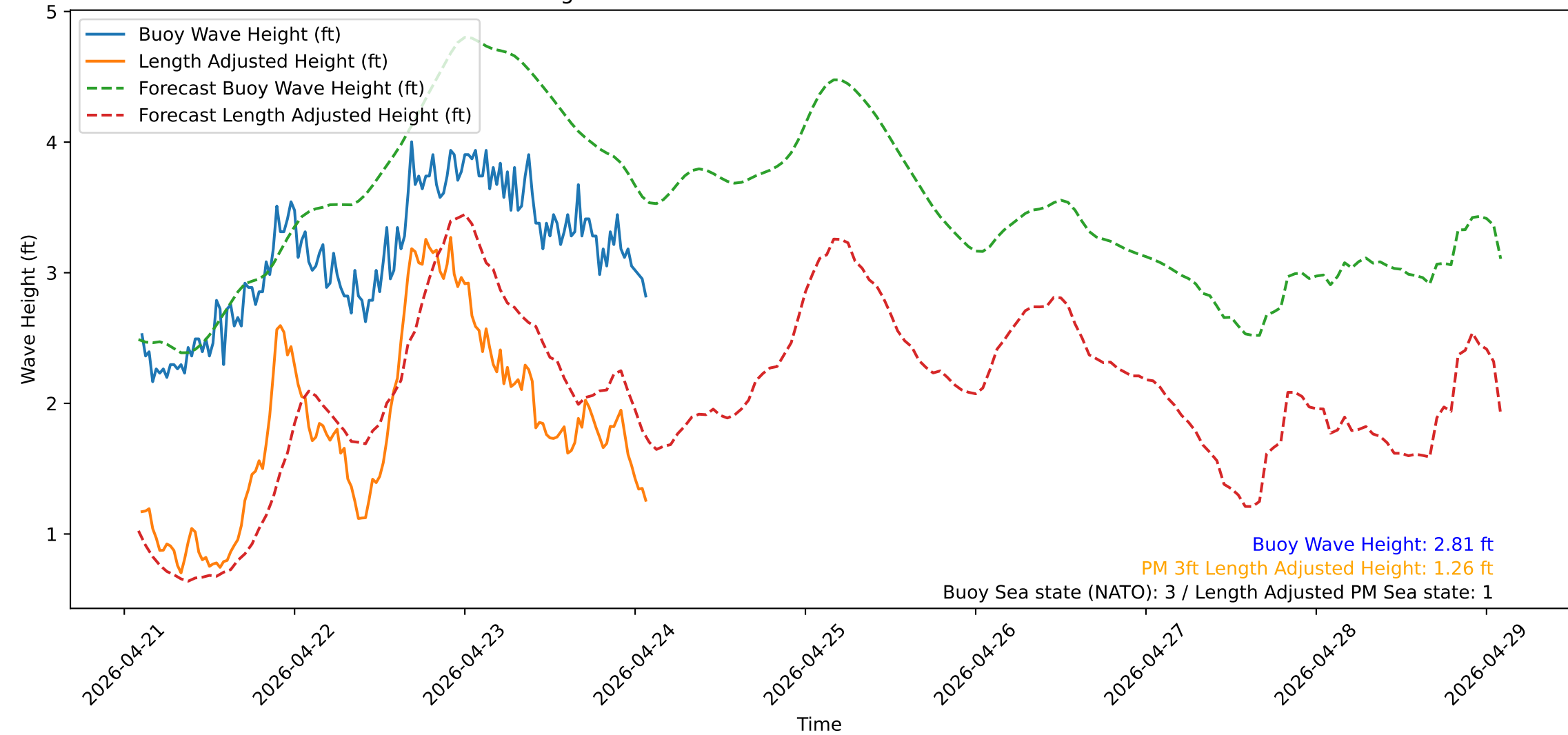
Wave Heights over Time for Green Beach at 2026-04-24 02:21:13
