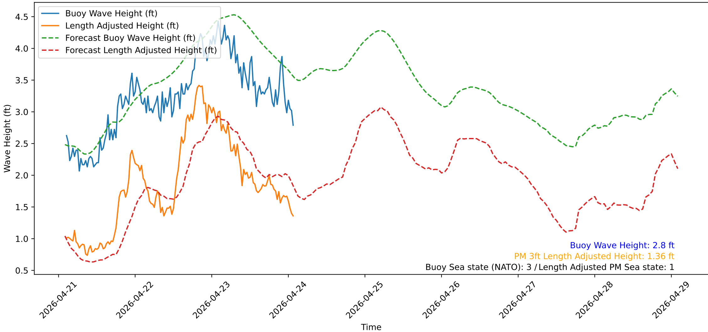
Wave Heights over Time for Oceanside Harbor at 2026-04-24 02:20:30
