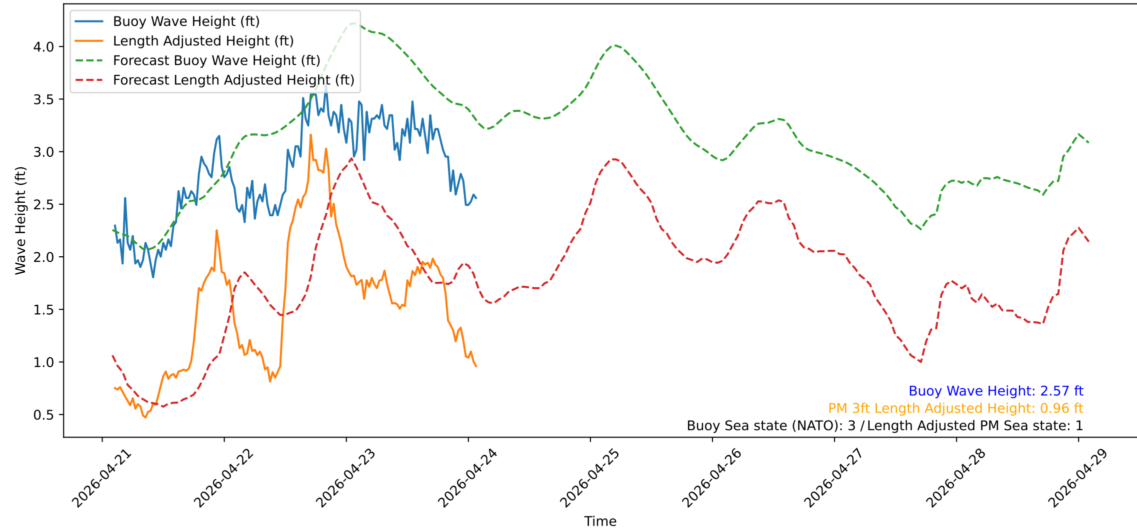
Wave Heights over Time for Red Beach at 2026-04-24 02:20:51
