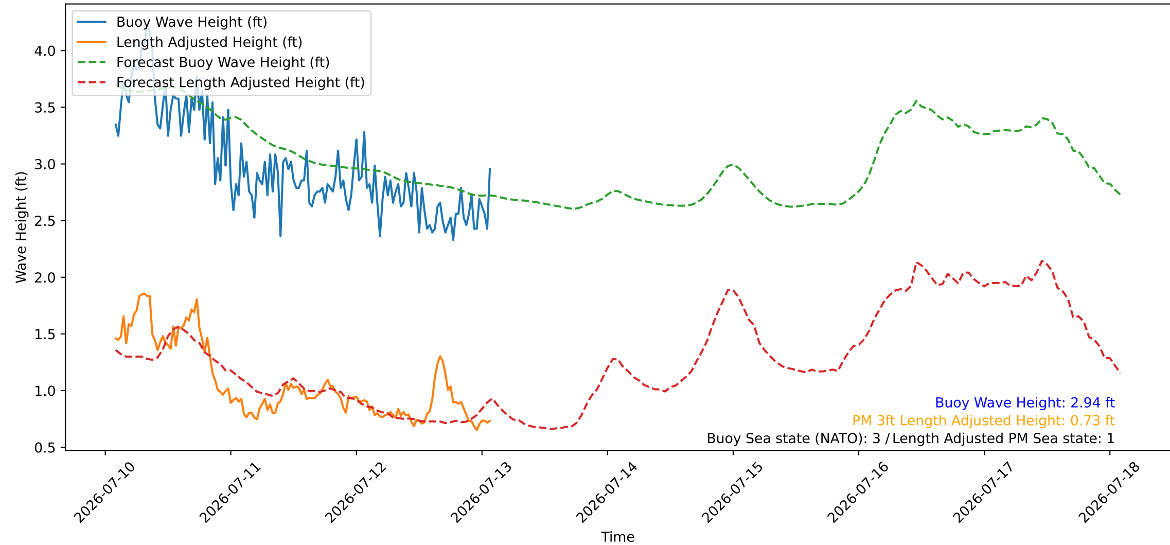
Wave Heights over Time for Oceanside Harbor at 2026-07-13 02:00:26
