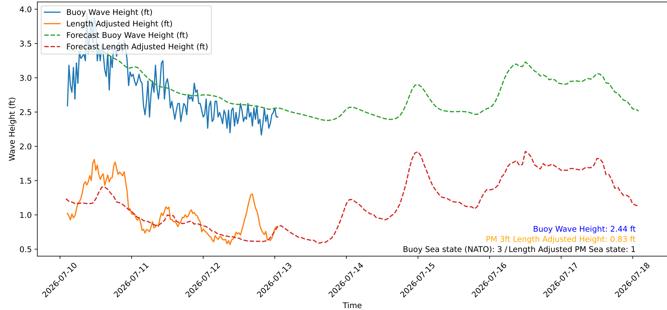
Wave Heights over Time for Red Beach at 2026-07-13 02:00:45
