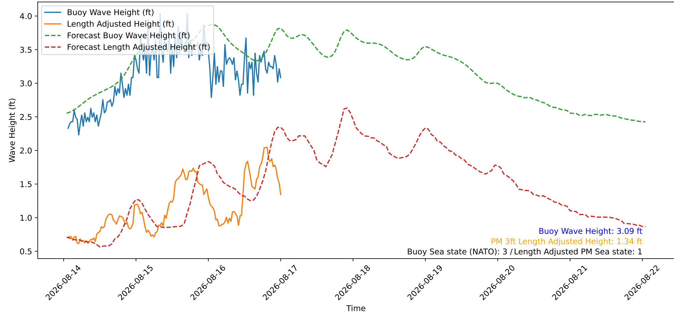
Wave Heights over Time for Red Beach at 2026-08-17 01:20:47
