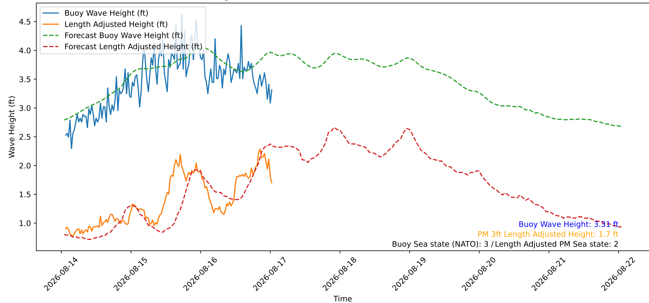
Wave Heights over Time for Oceanside Harbor at 2026-08-17 01:20:26
