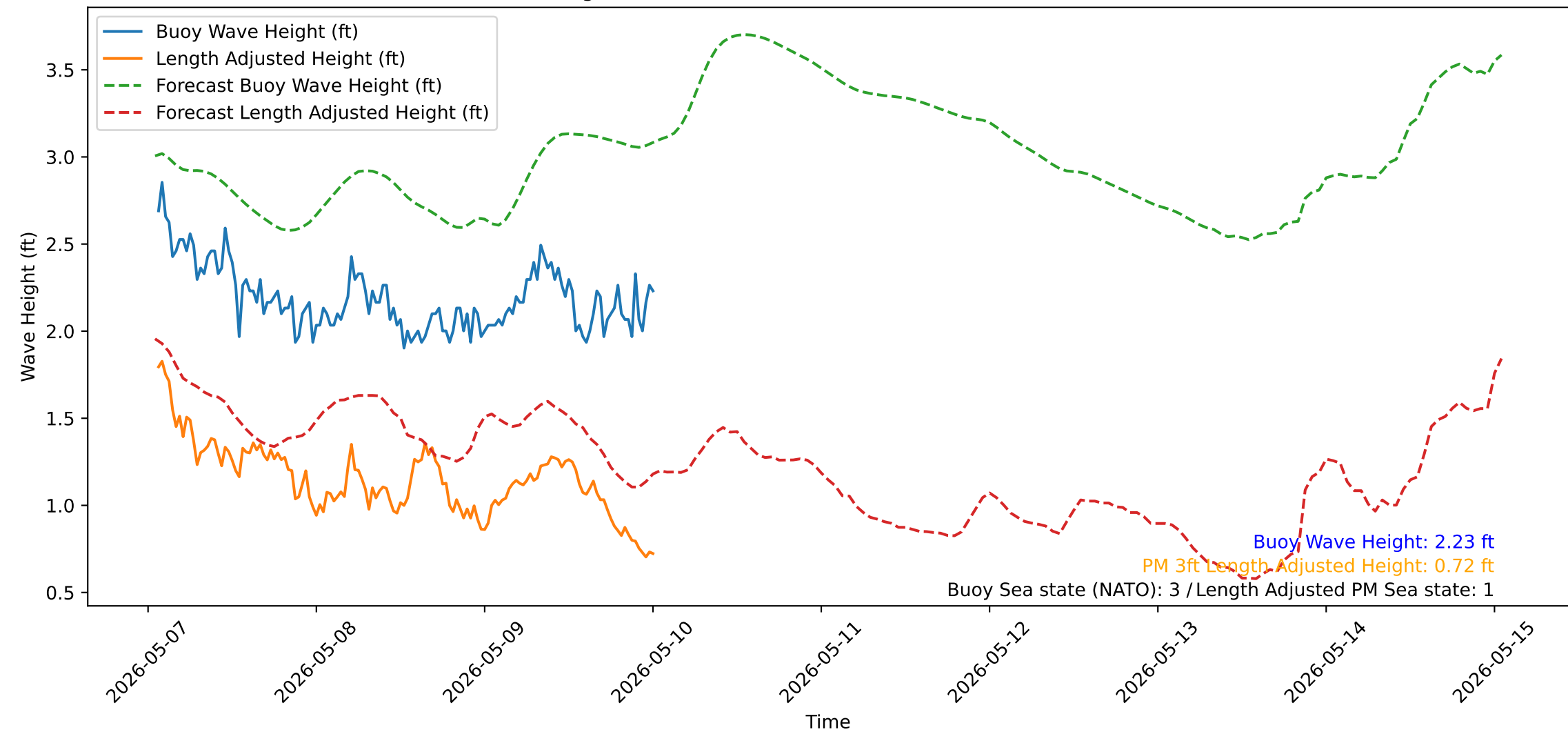
Wave Heights over Time for Red Beach at 2026-05-10 01:00:50
