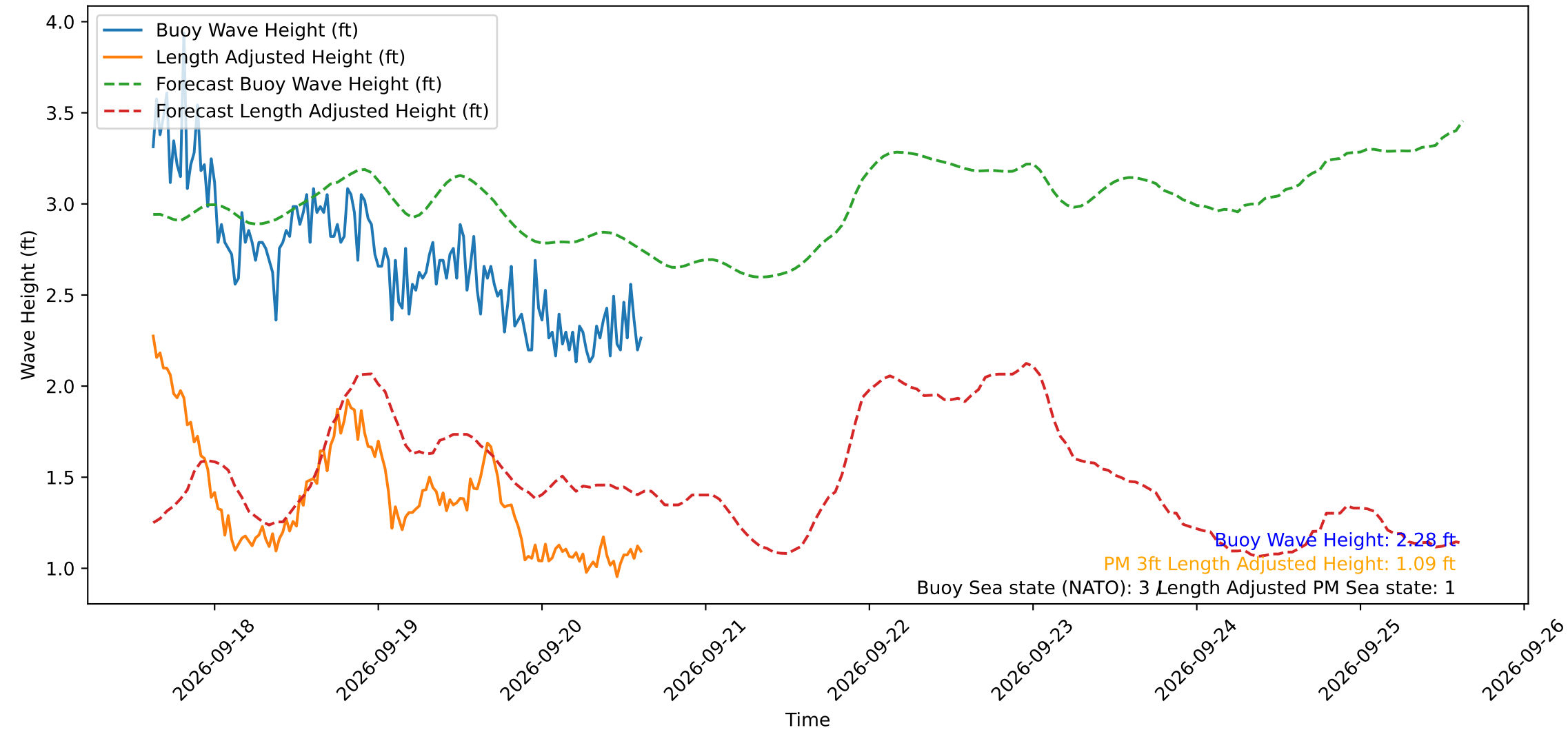
Wave Heights over Time for Oceanside Harbor at 2026-09-20 15:10:30
