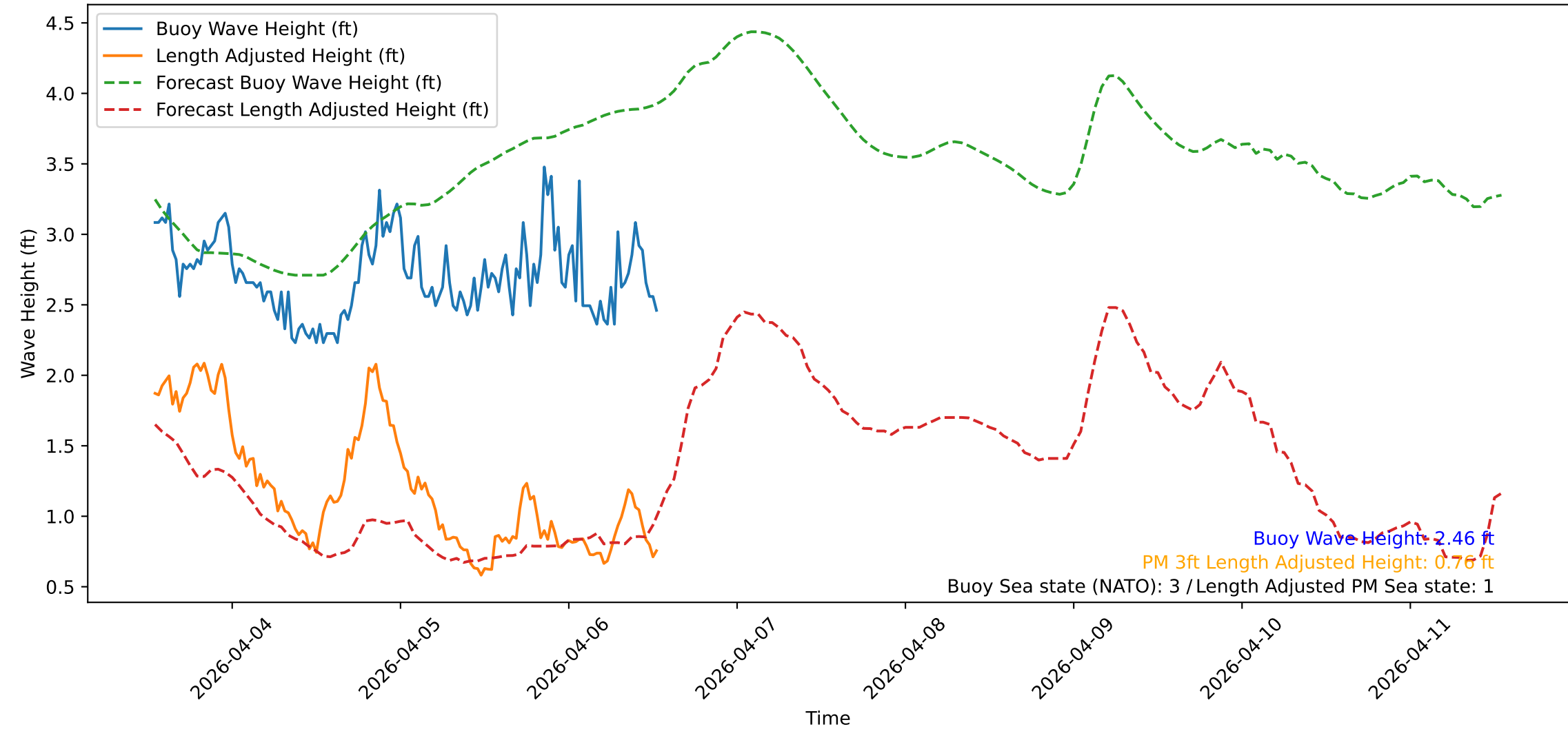
Wave Heights over Time for Green Beach at 2026-04-06 13:11:10
