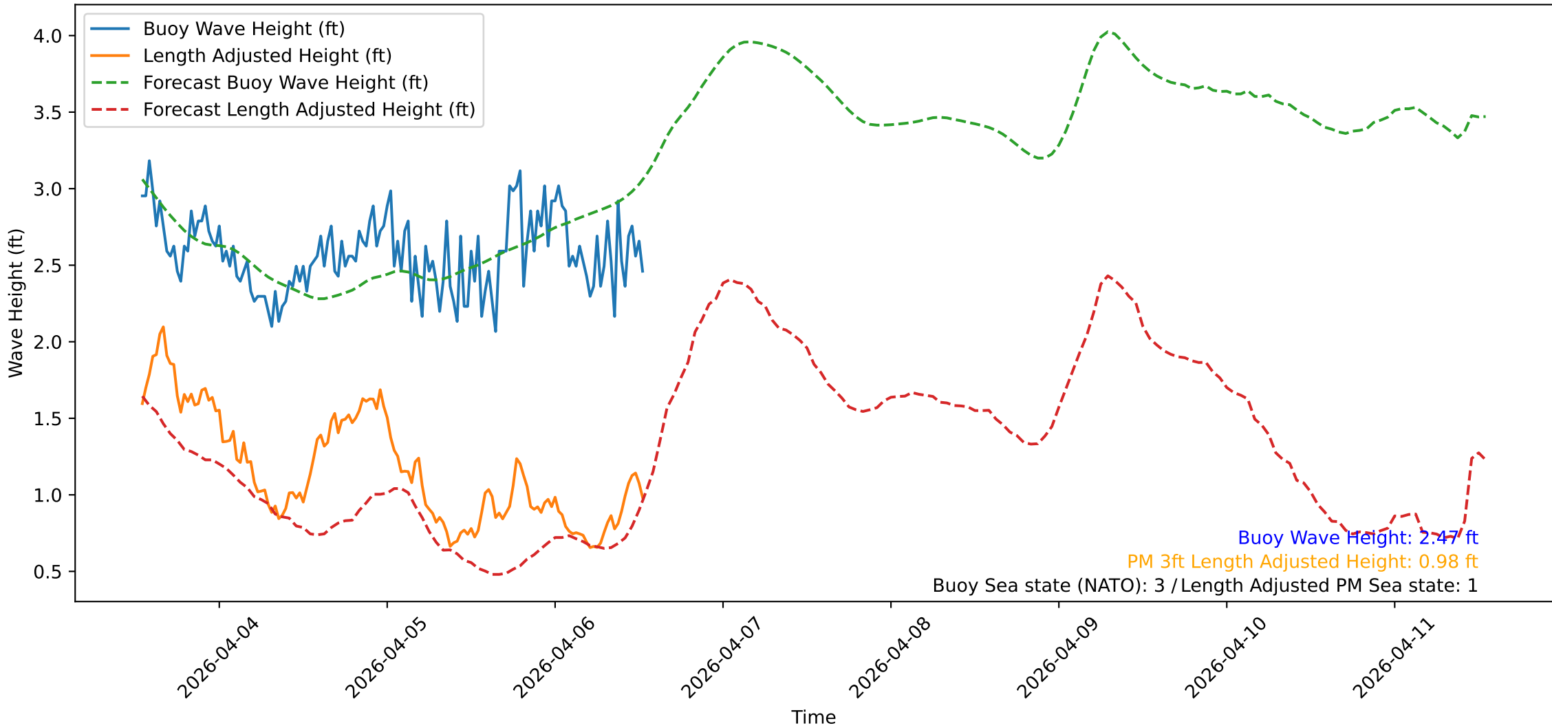
Wave Heights over Time for Oceanside Harbor at 2026-04-06 13:10:32
