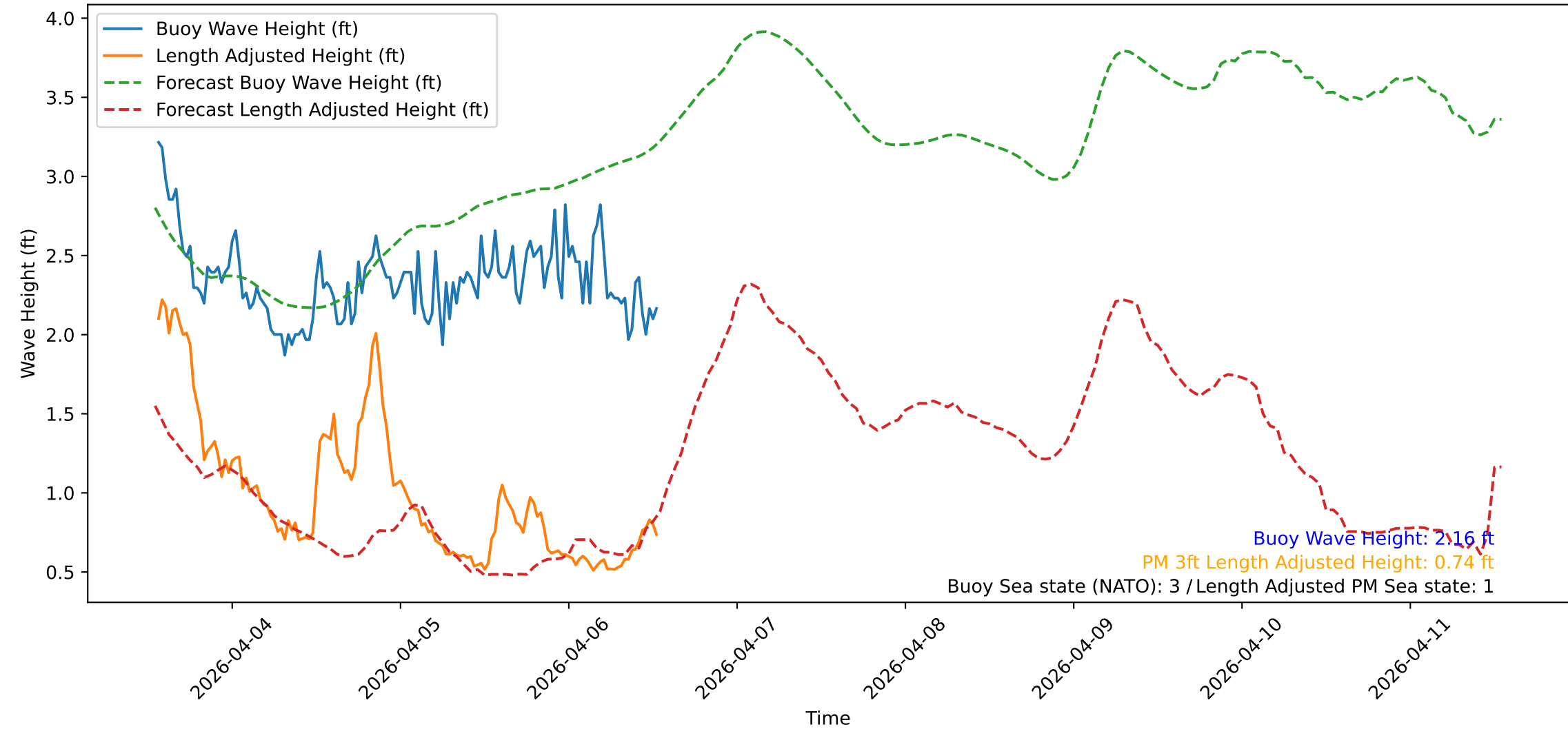
Wave Heights over Time for Red Beach at 2026-04-06 13:10:48
