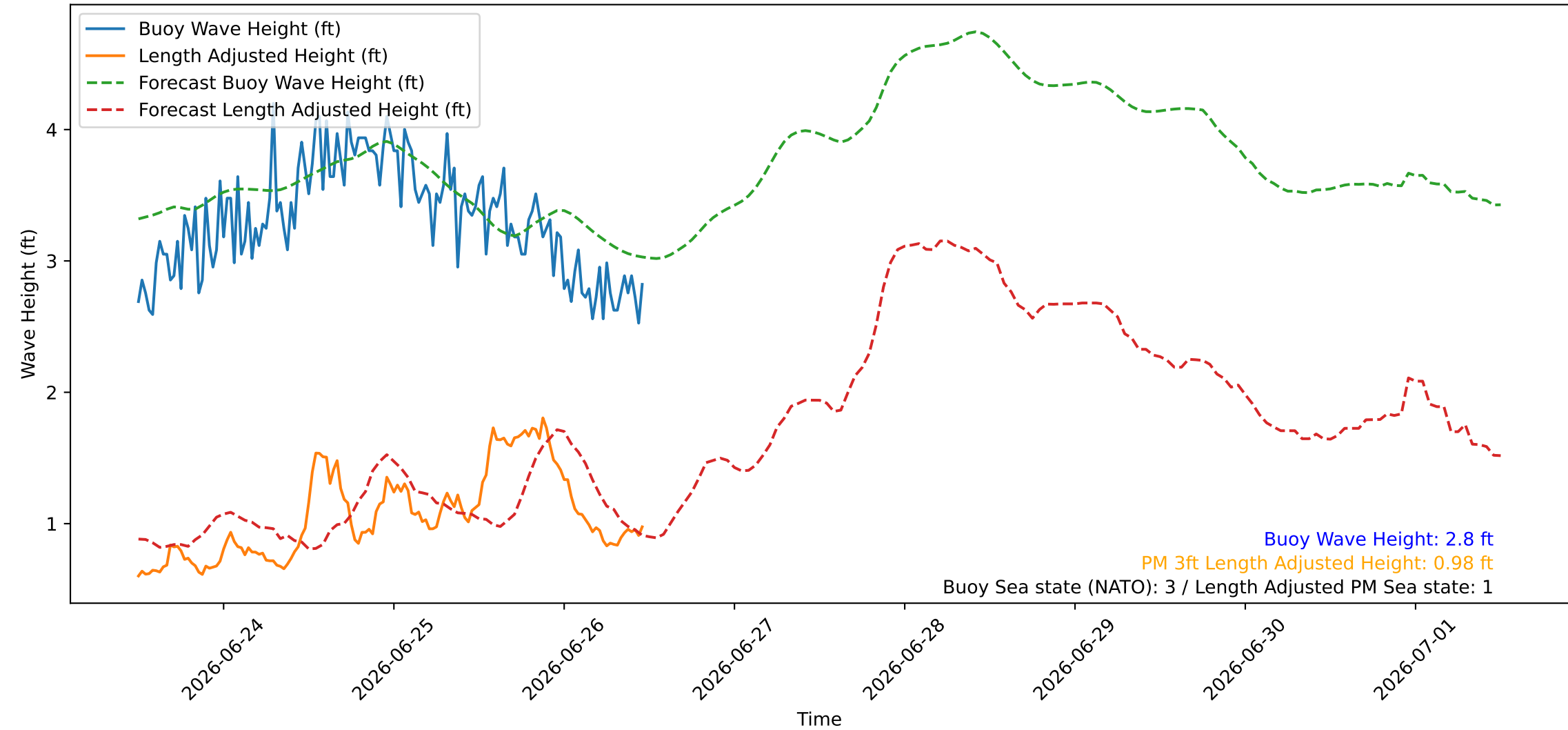
Wave Heights over Time for Green Beach at 2026-06-26 12:01:08
