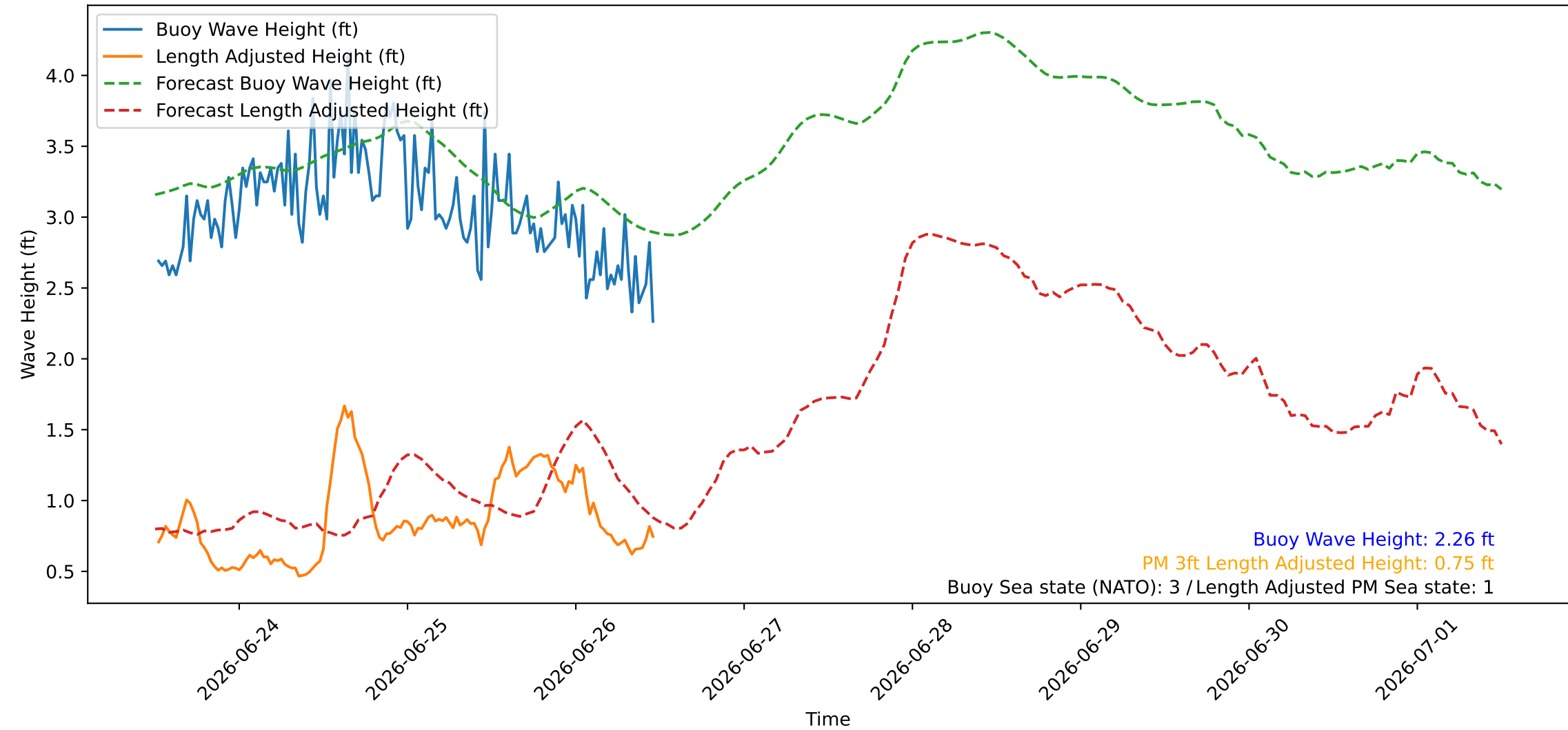
Wave Heights over Time for Red Beach at 2026-06-26 12:00:45
