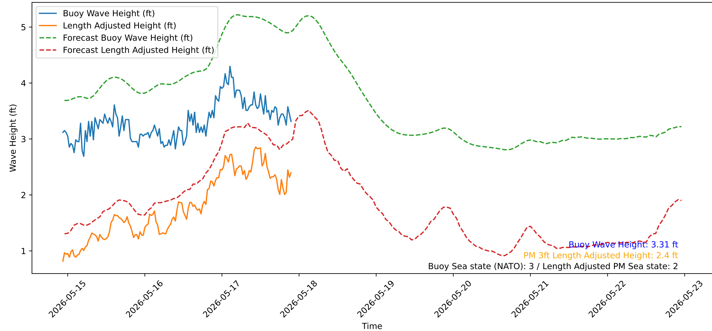
Wave Heights over Time for Oceanside Harbor at 2026-05-17 22:30:32
