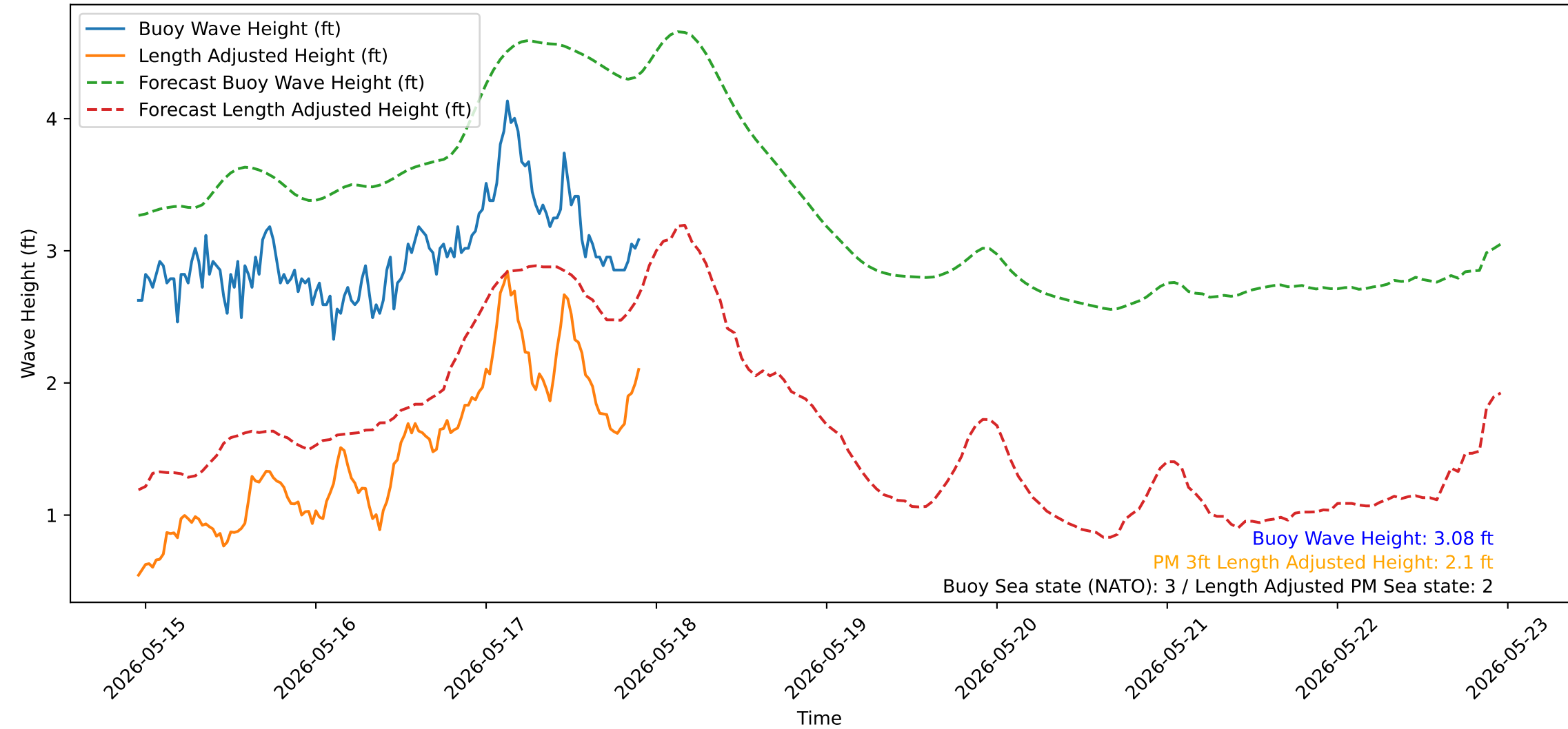
Wave Heights over Time for Red Beach at 2026-05-17 22:30:51
