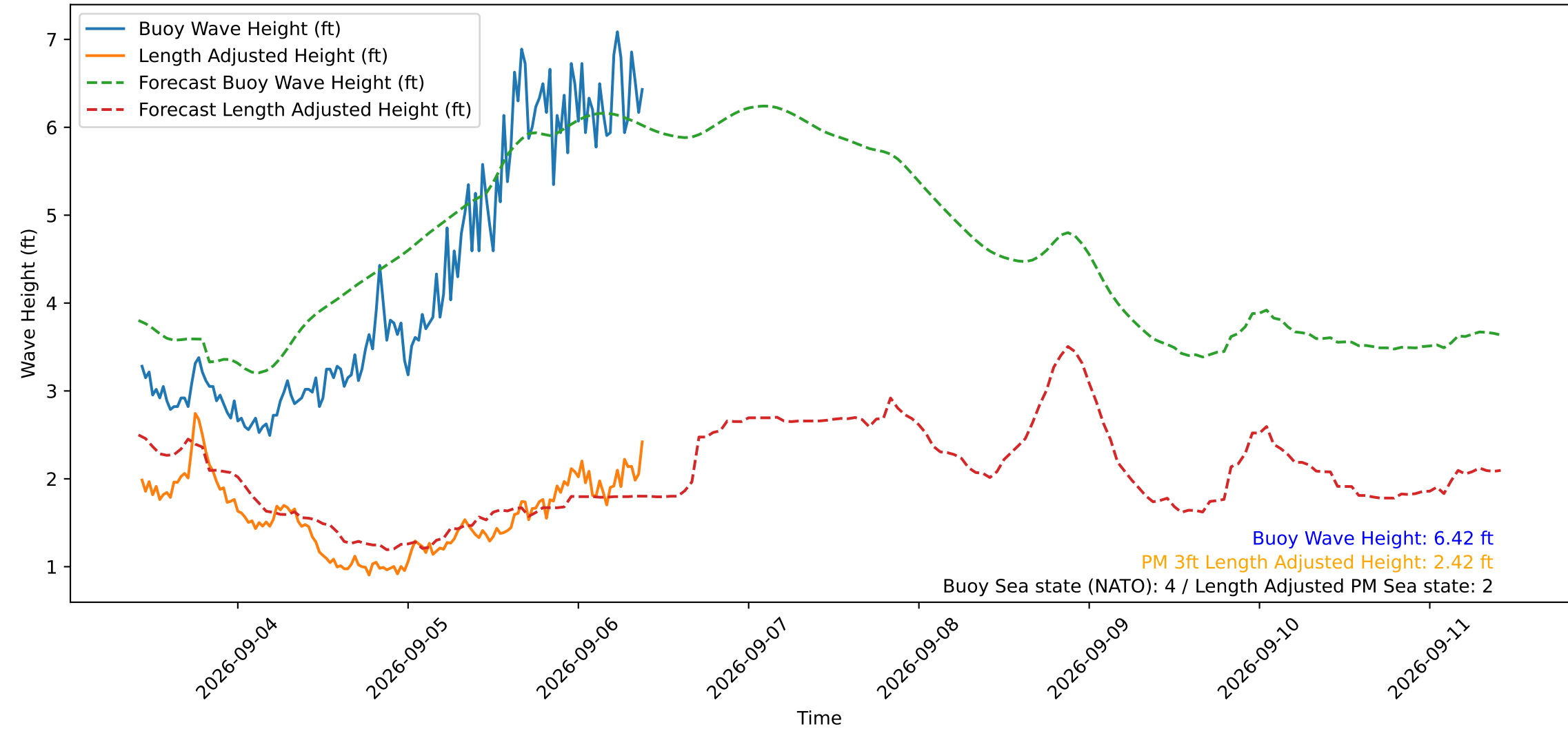
Wave Heights over Time for Green Beach at 2026-09-06 10:01:12
