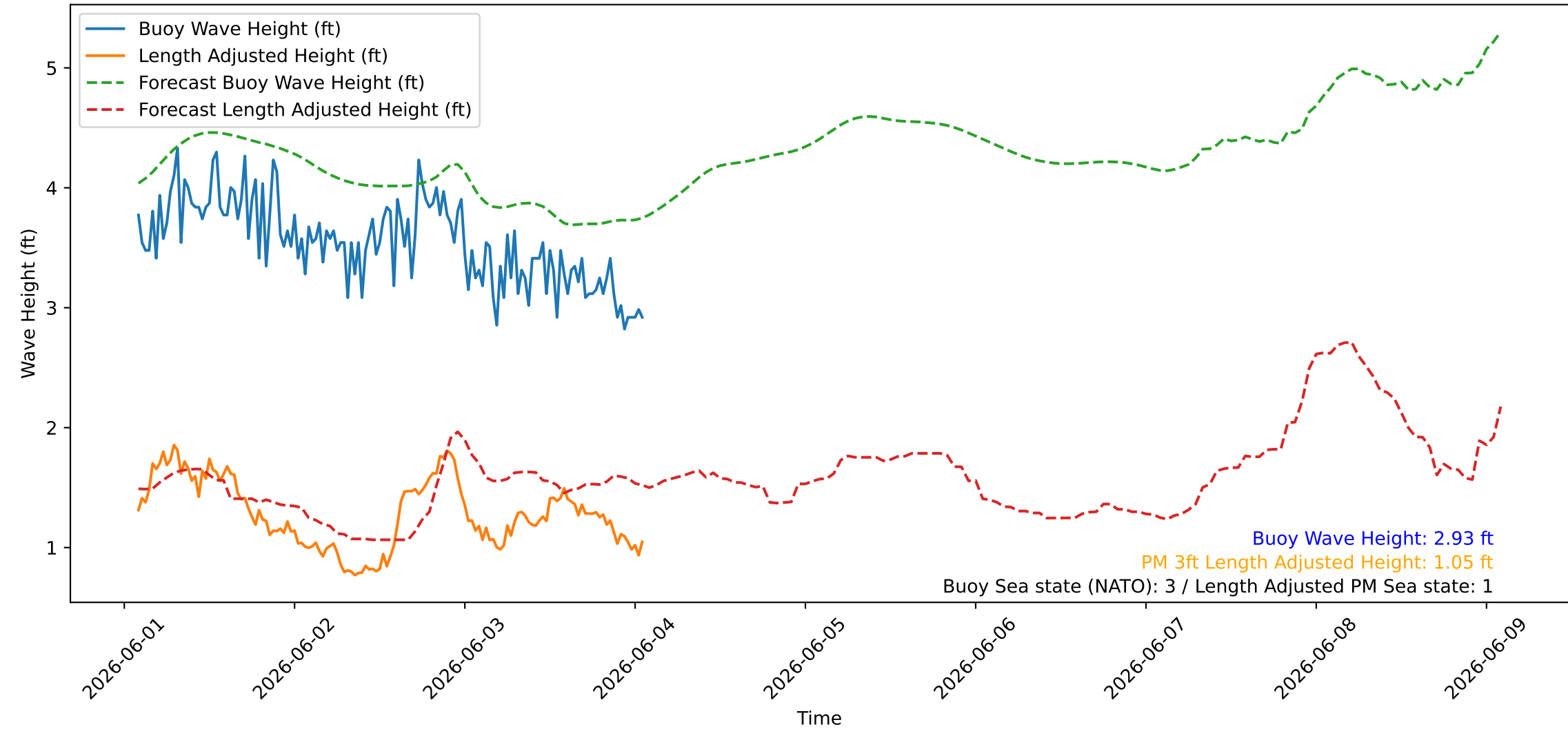
Wave Heights over Time for Green Beach at 2026-06-04 01:51:08
