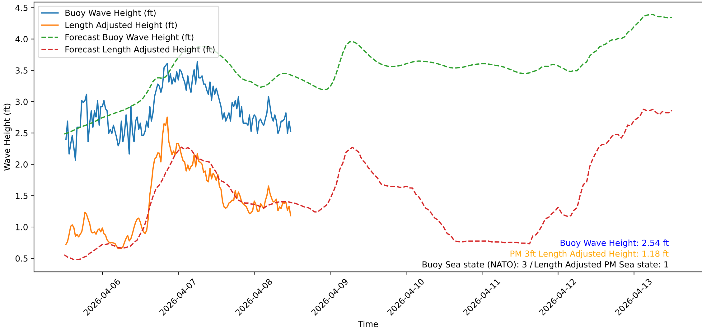
Wave Heights over Time for Oceanside Harbor at 2026-04-08 12:20:31
