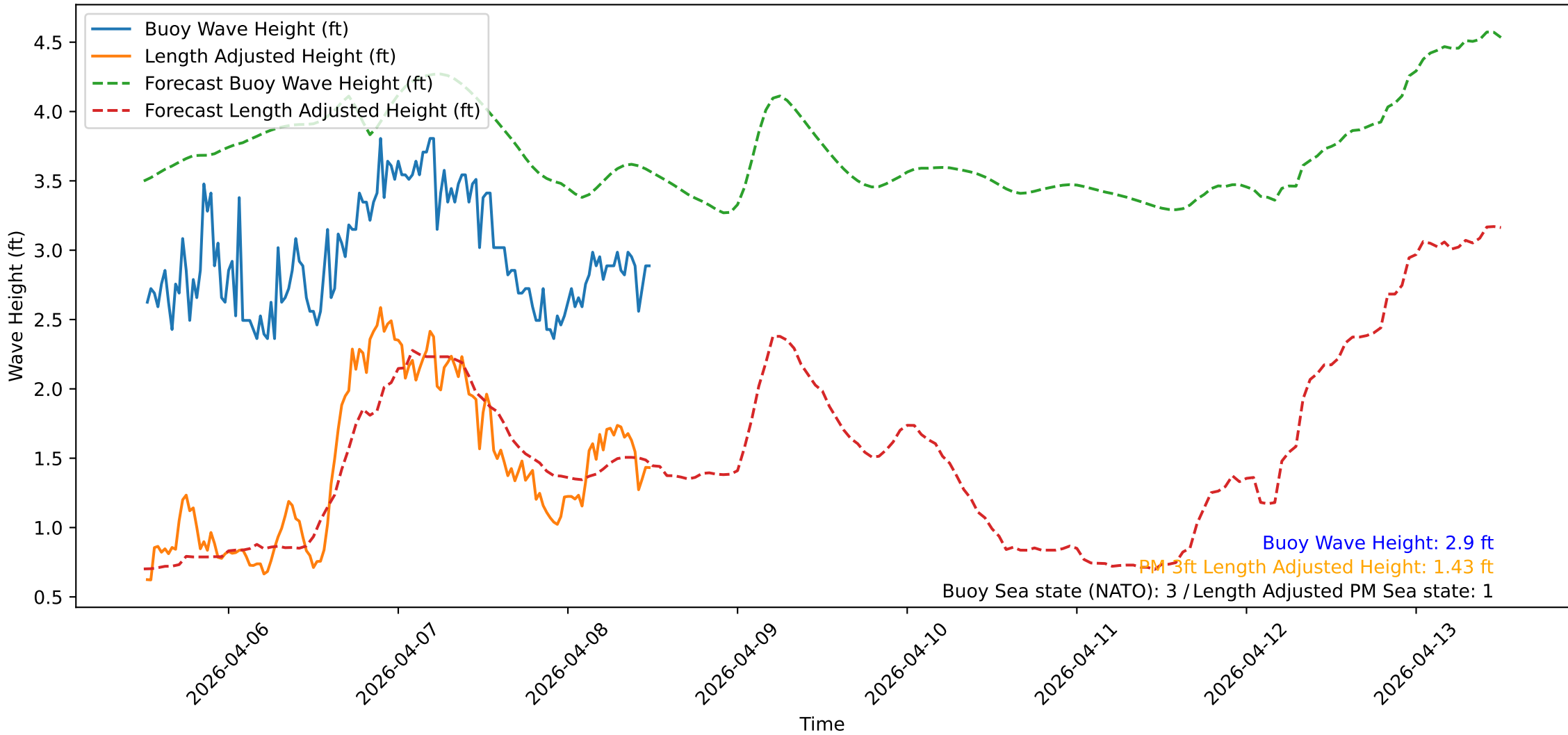
Wave Heights over Time for Green Beach at 2026-04-08 12:21:09
