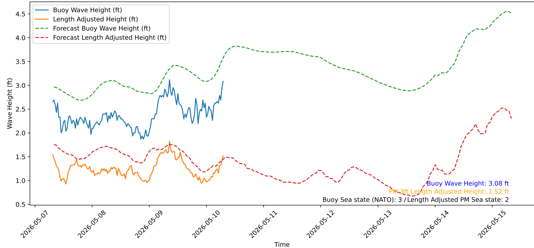
Wave Heights over Time for Oceanside Harbor at 2026-05-10 07:30:31
