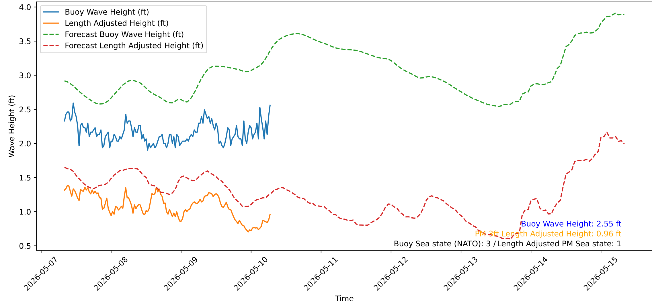
Wave Heights over Time for Red Beach at 2026-05-10 07:30:51
