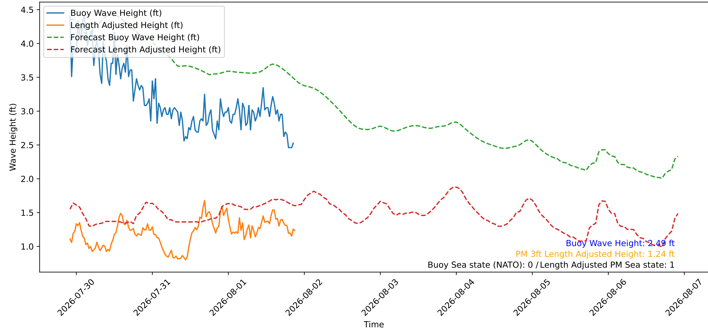
Wave Heights over Time for Red Beach at 2026-08-01 21:50:48
