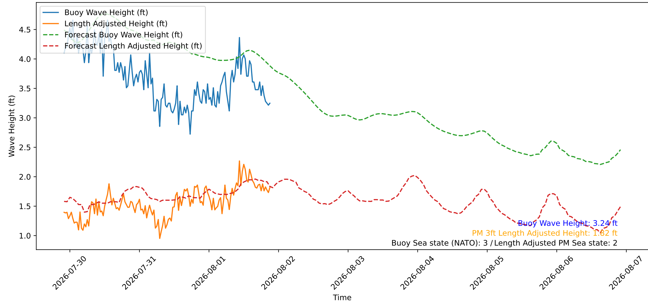
Wave Heights over Time for Oceanside Harbor at 2026-08-01 21:50:27
