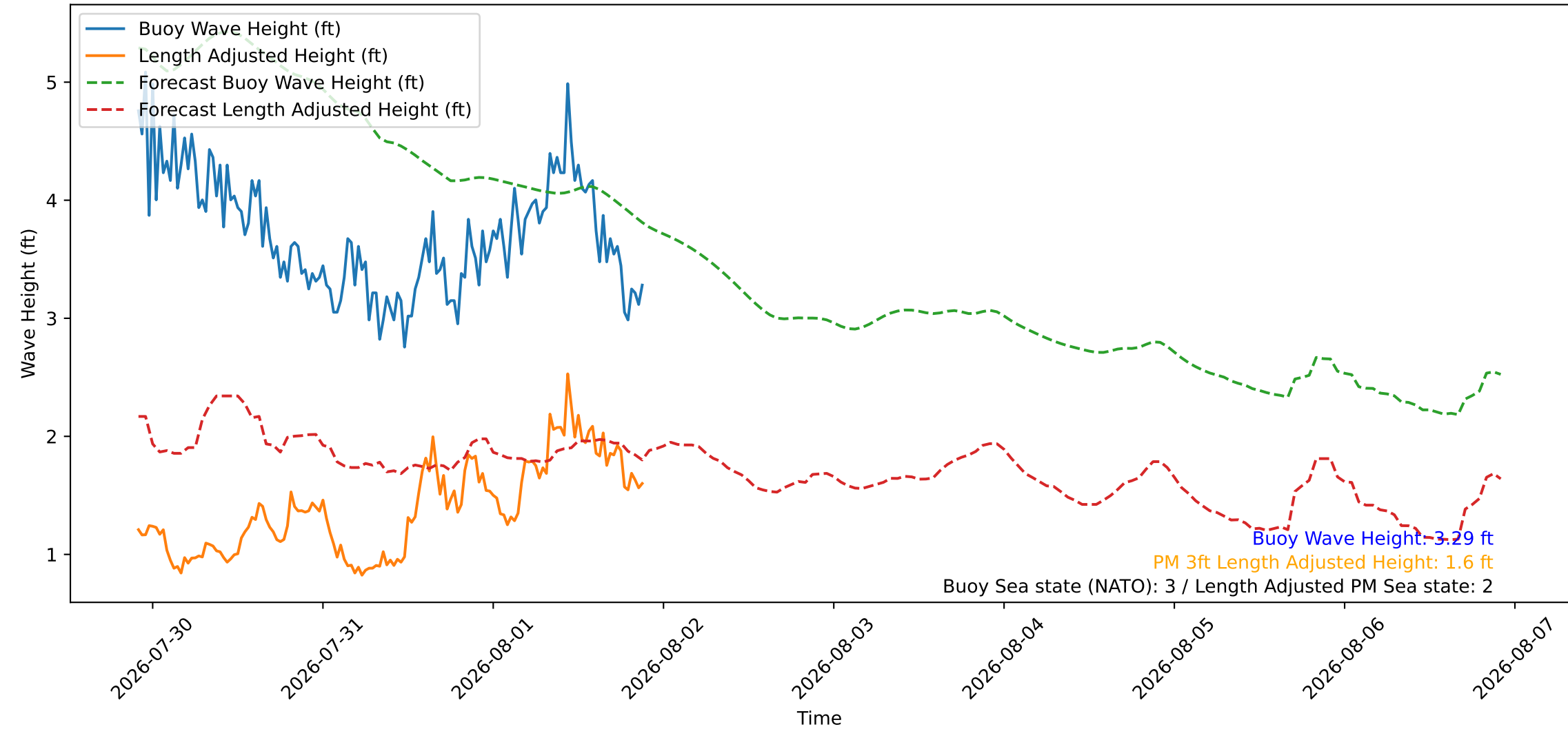
Wave Heights over Time for Green Beach at 2026-08-01 21:51:10
