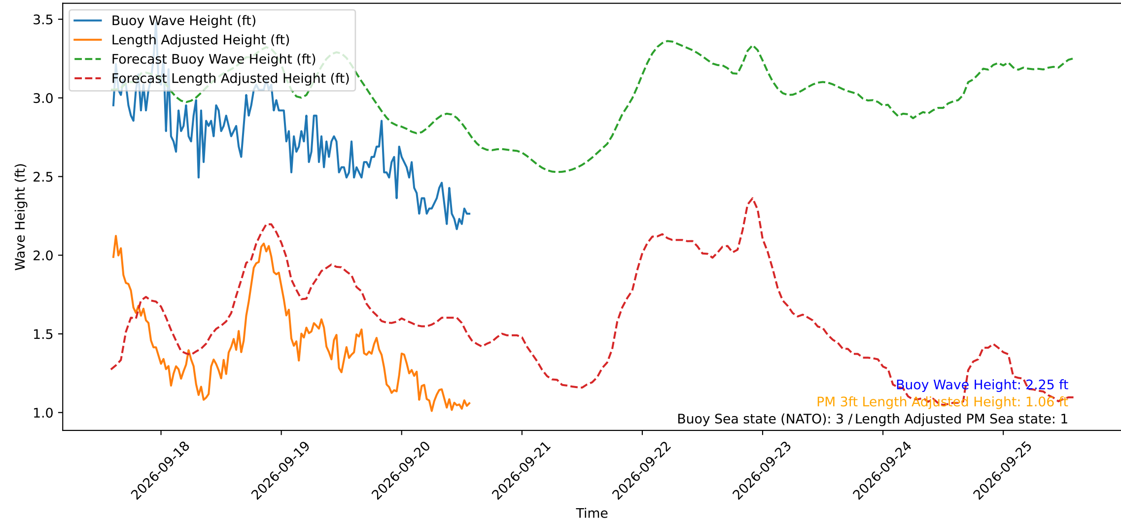
Wave Heights over Time for Green Beach at 2026-09-20 14:11:12
