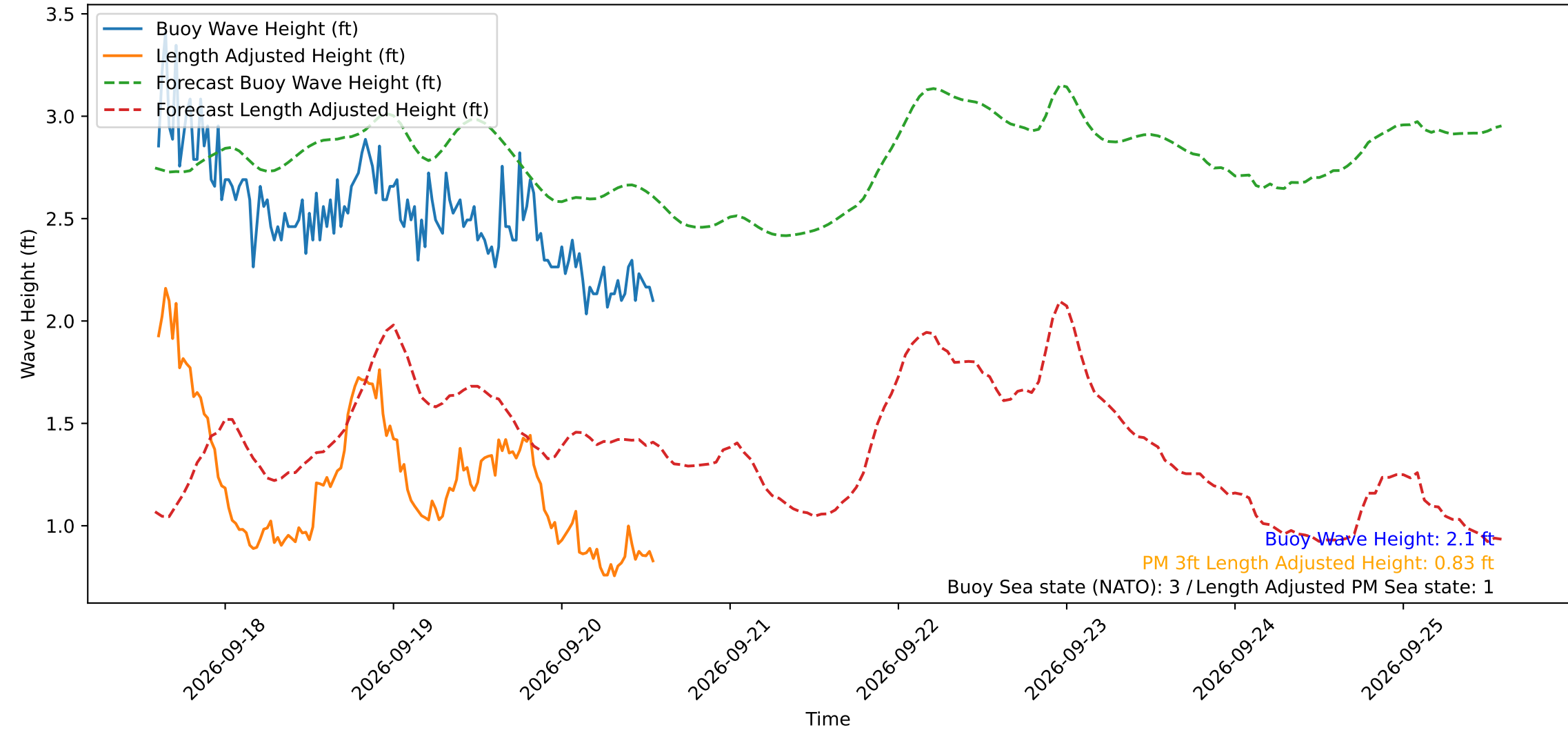
Wave Heights over Time for Red Beach at 2026-09-20 14:10:50
