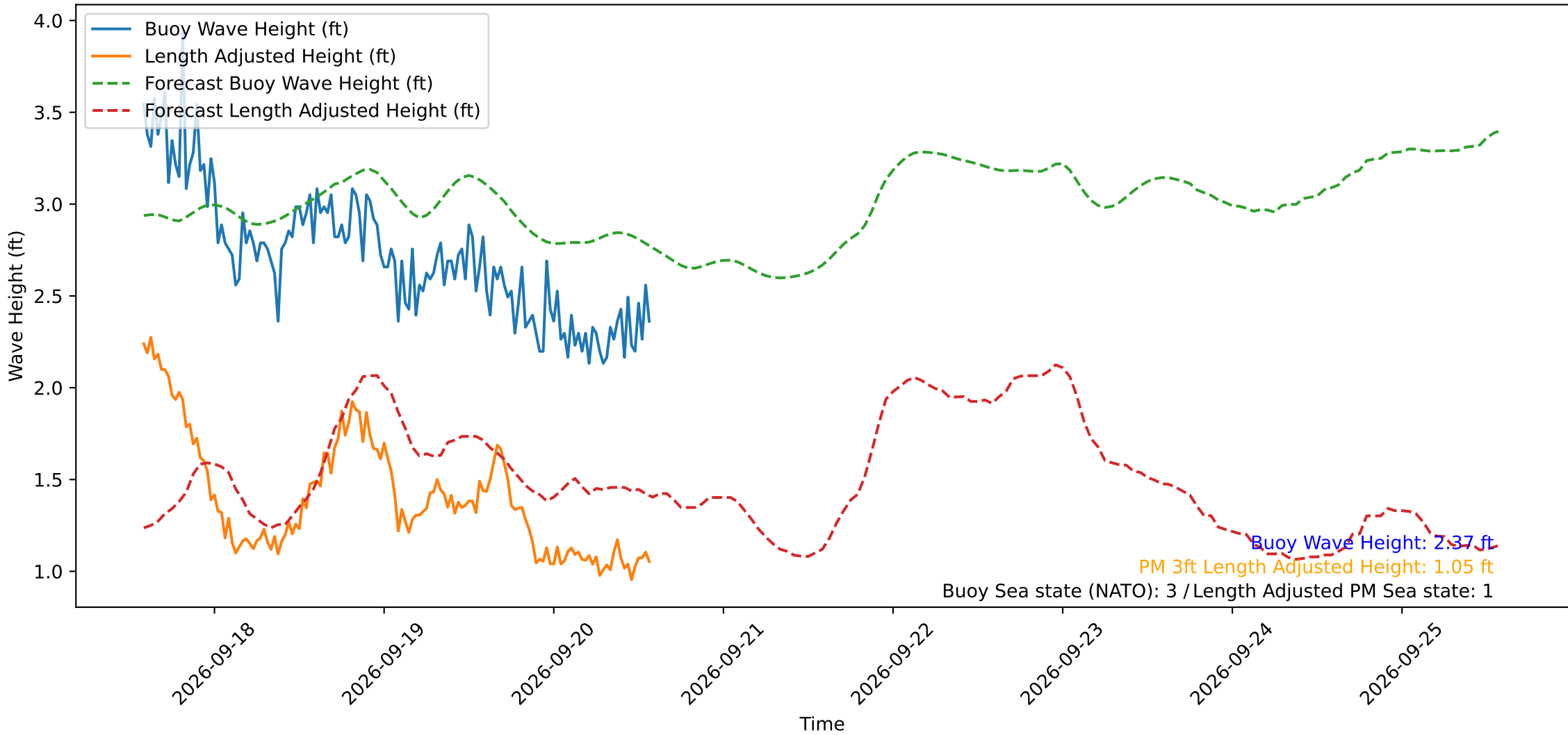
Wave Heights over Time for Oceanside Harbor at 2026-09-20 14:10:30
