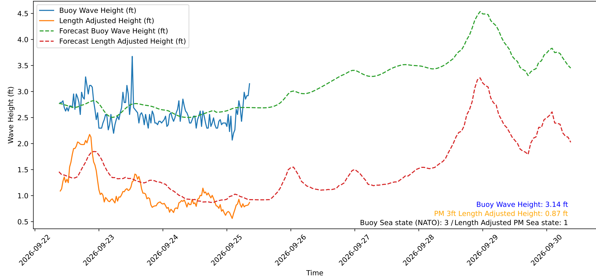
Wave Heights over Time for Red Beach at 2026-09-25 09:20:49
