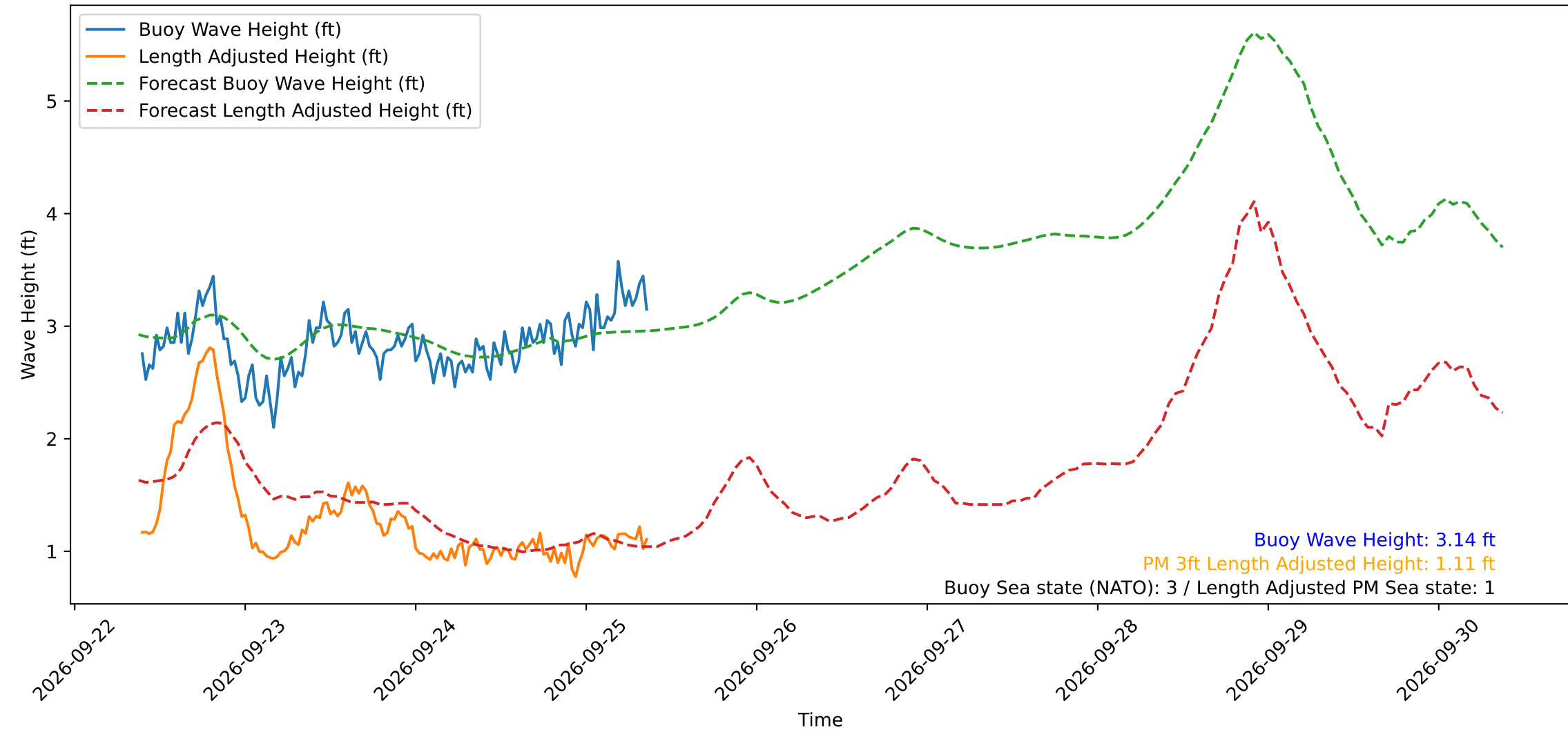
Wave Heights over Time for Green Beach at 2026-09-25 09:21:13
