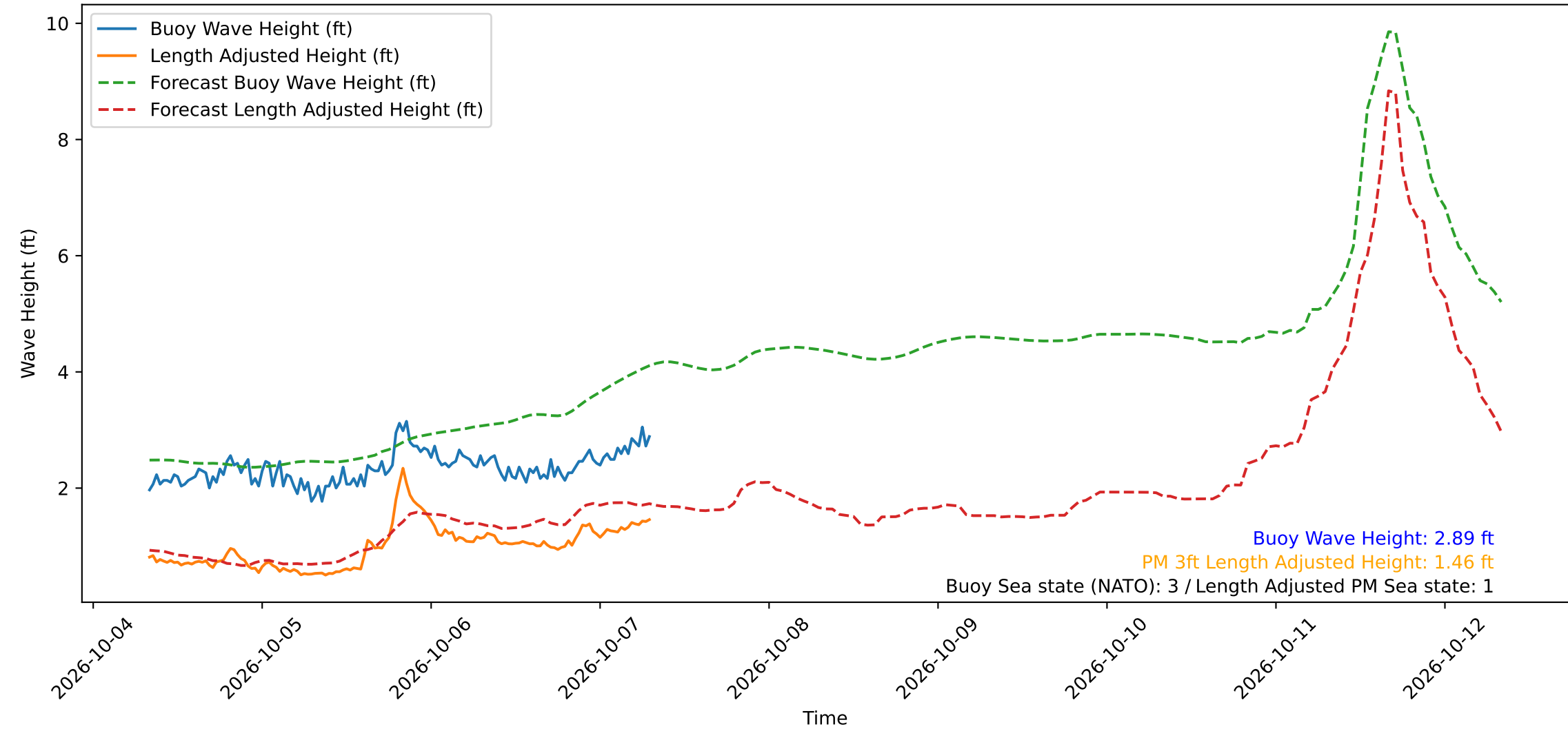
Wave Heights over Time for Green Beach at 2026-10-07 07:51:15
