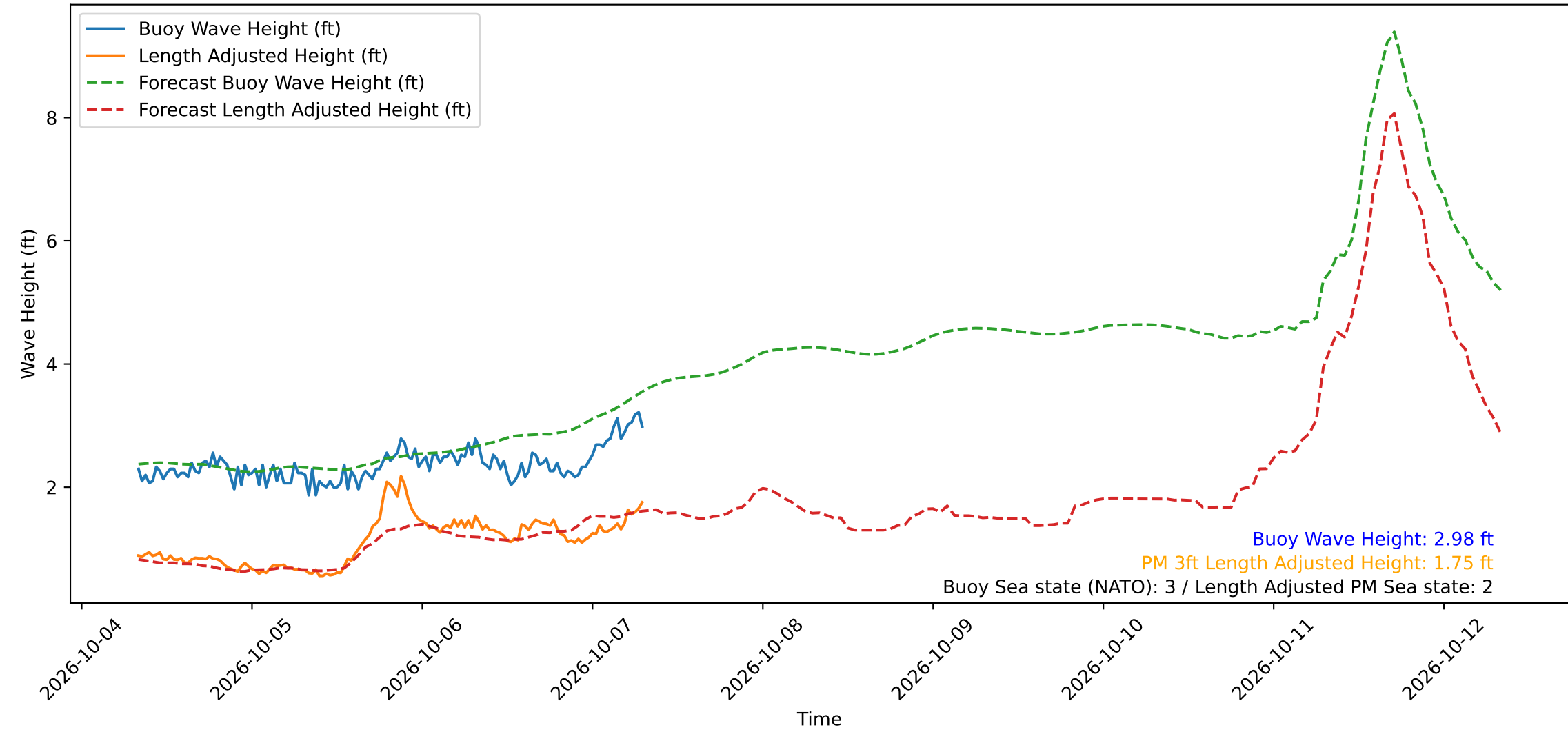
Wave Heights over Time for Oceanside Harbor at 2026-10-07 07:50:30
