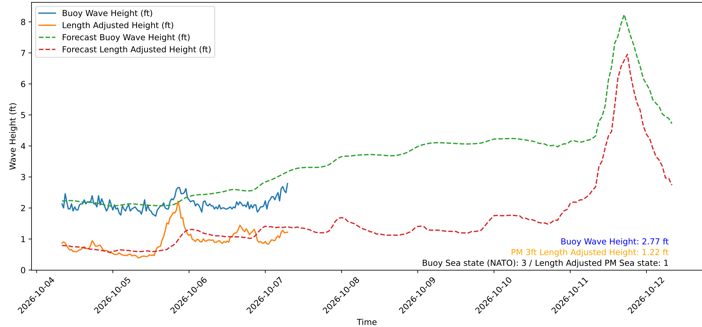
Wave Heights over Time for Red Beach at 2026-10-07 07:50:50
