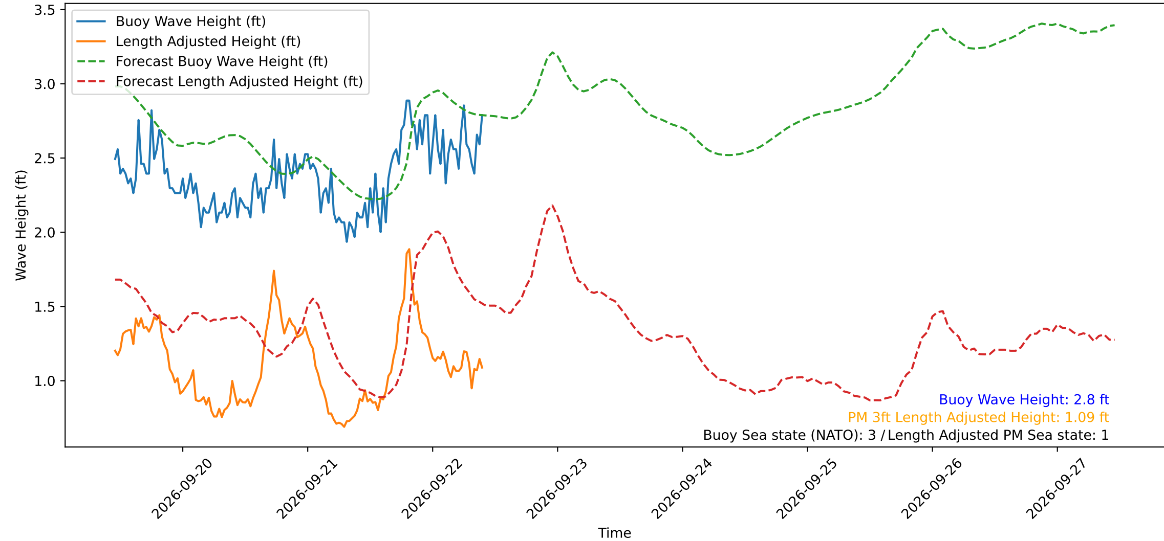
Wave Heights over Time for Red Beach at 2026-09-22 10:30:48
