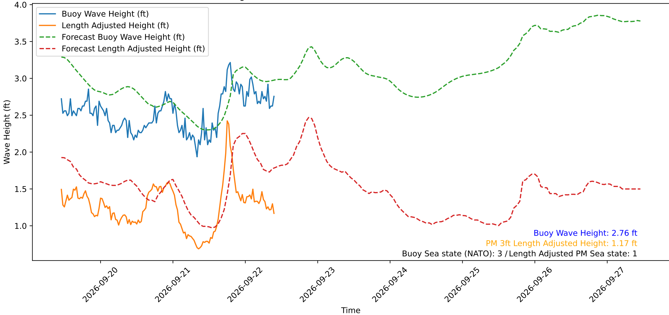
Wave Heights over Time for Green Beach at 2026-09-22 10:31:11
