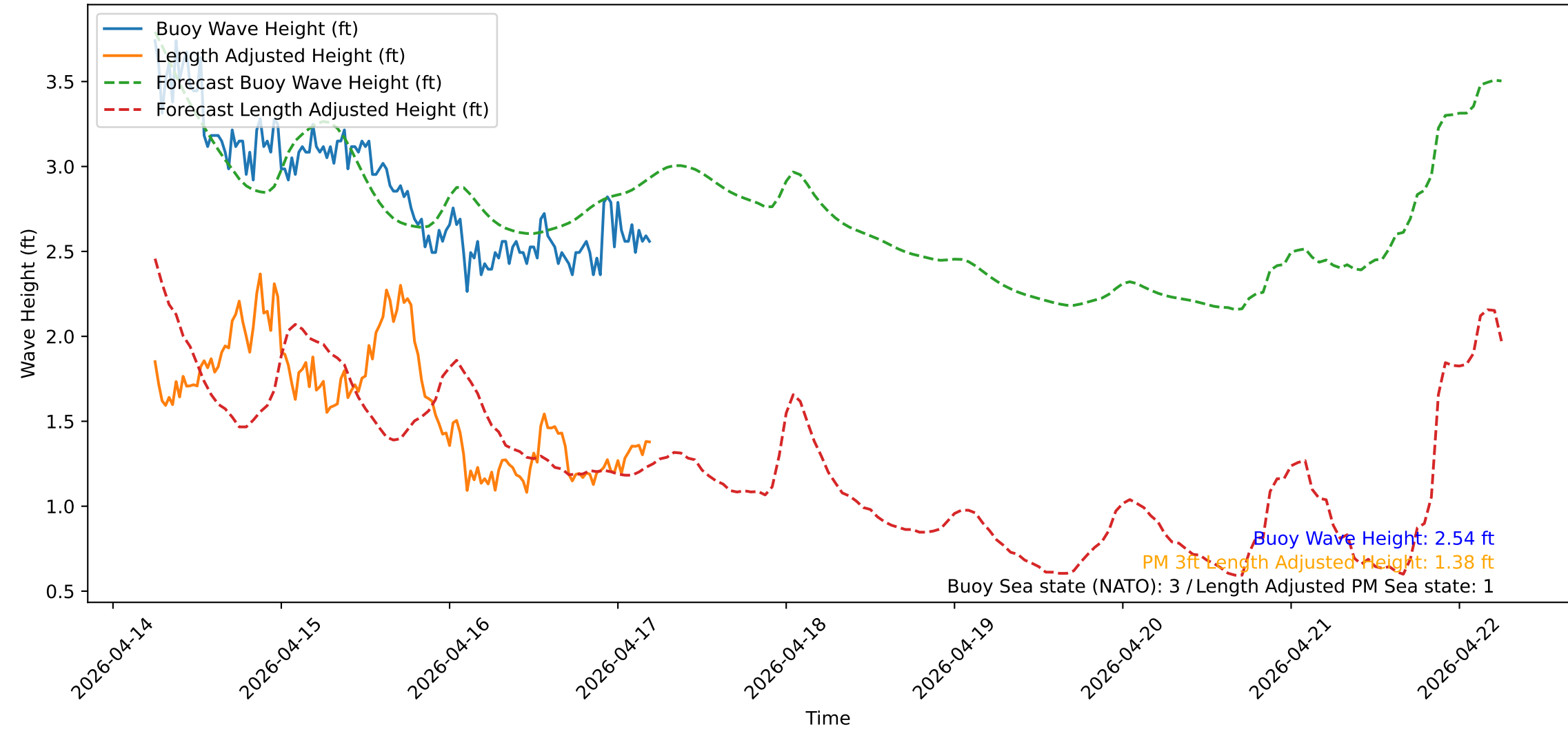
Wave Heights over Time for Red Beach at 2026-04-17 05:30:51
