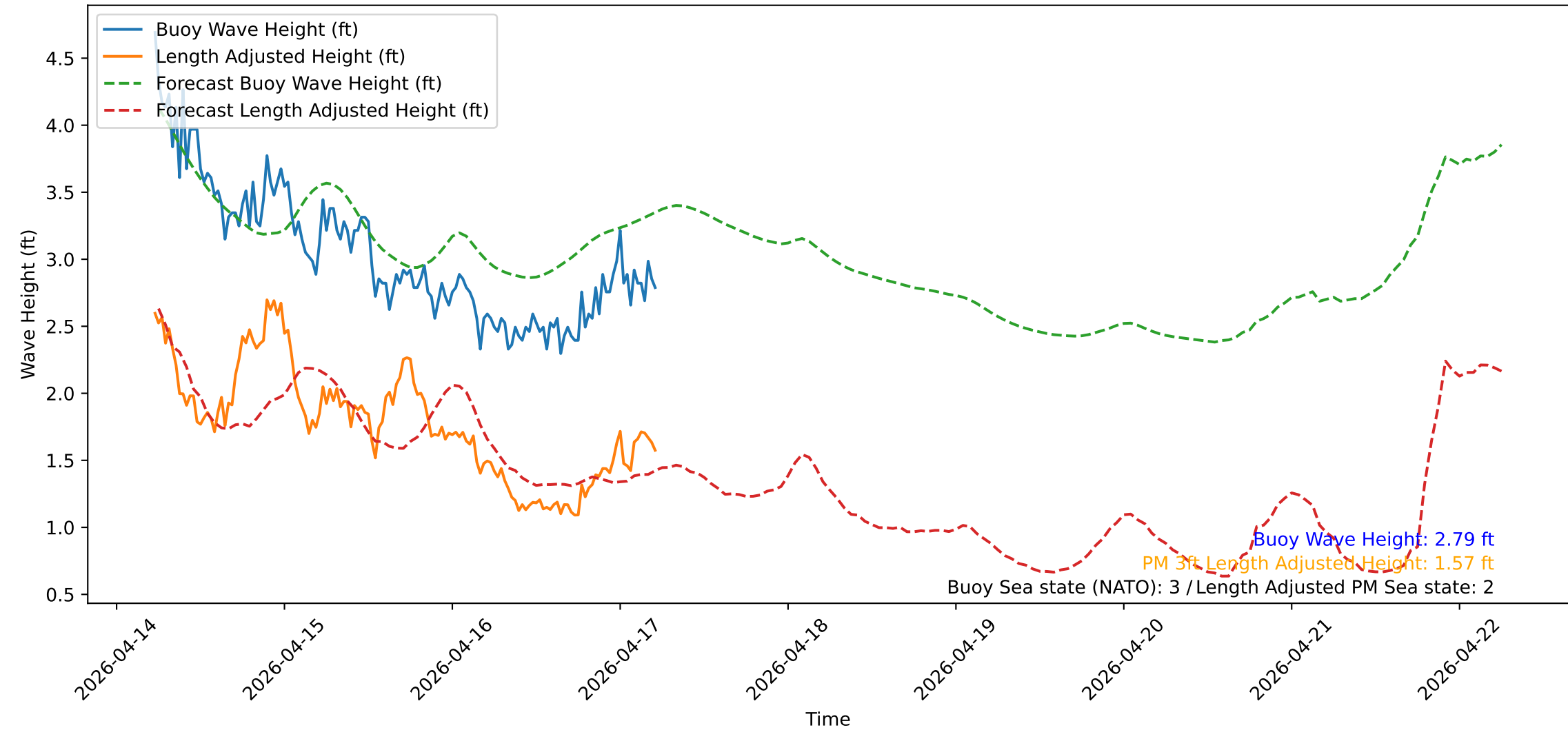
Wave Heights over Time for Oceanside Harbor at 2026-04-17 05:30:32
