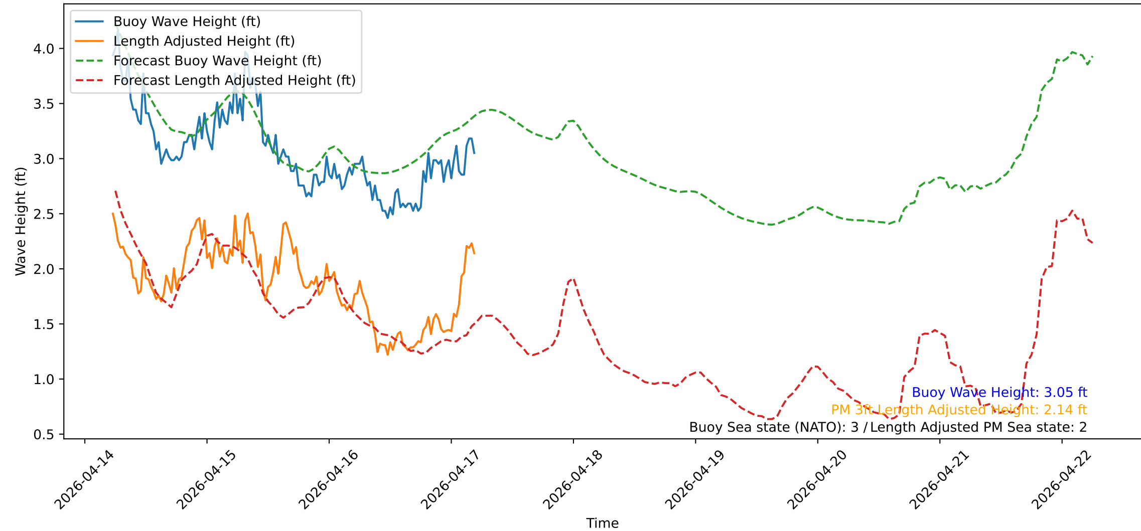
Wave Heights over Time for Green Beach at 2026-04-17 05:31:20
