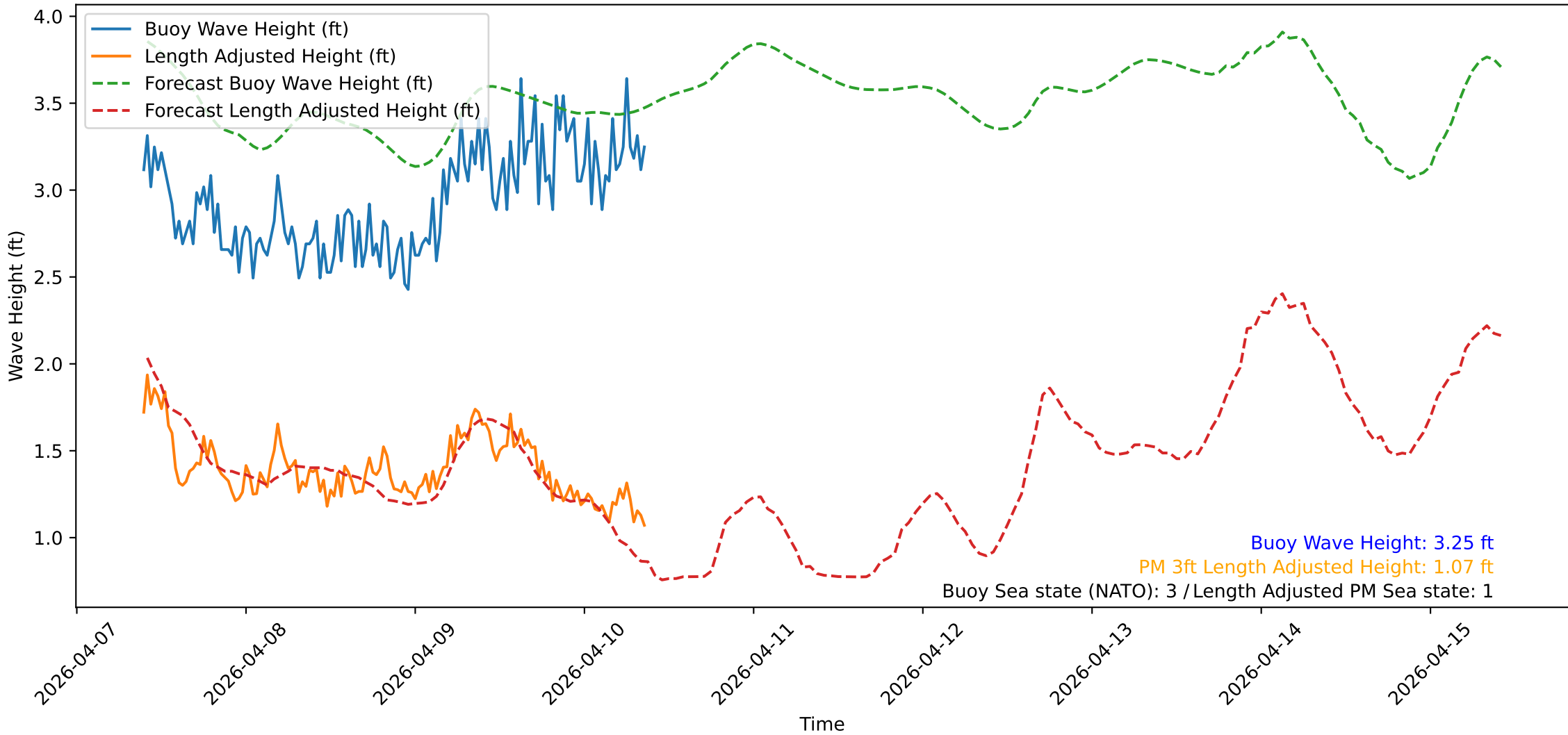
Wave Heights over Time for Oceanside Harbor at 2026-04-10 09:30:31
