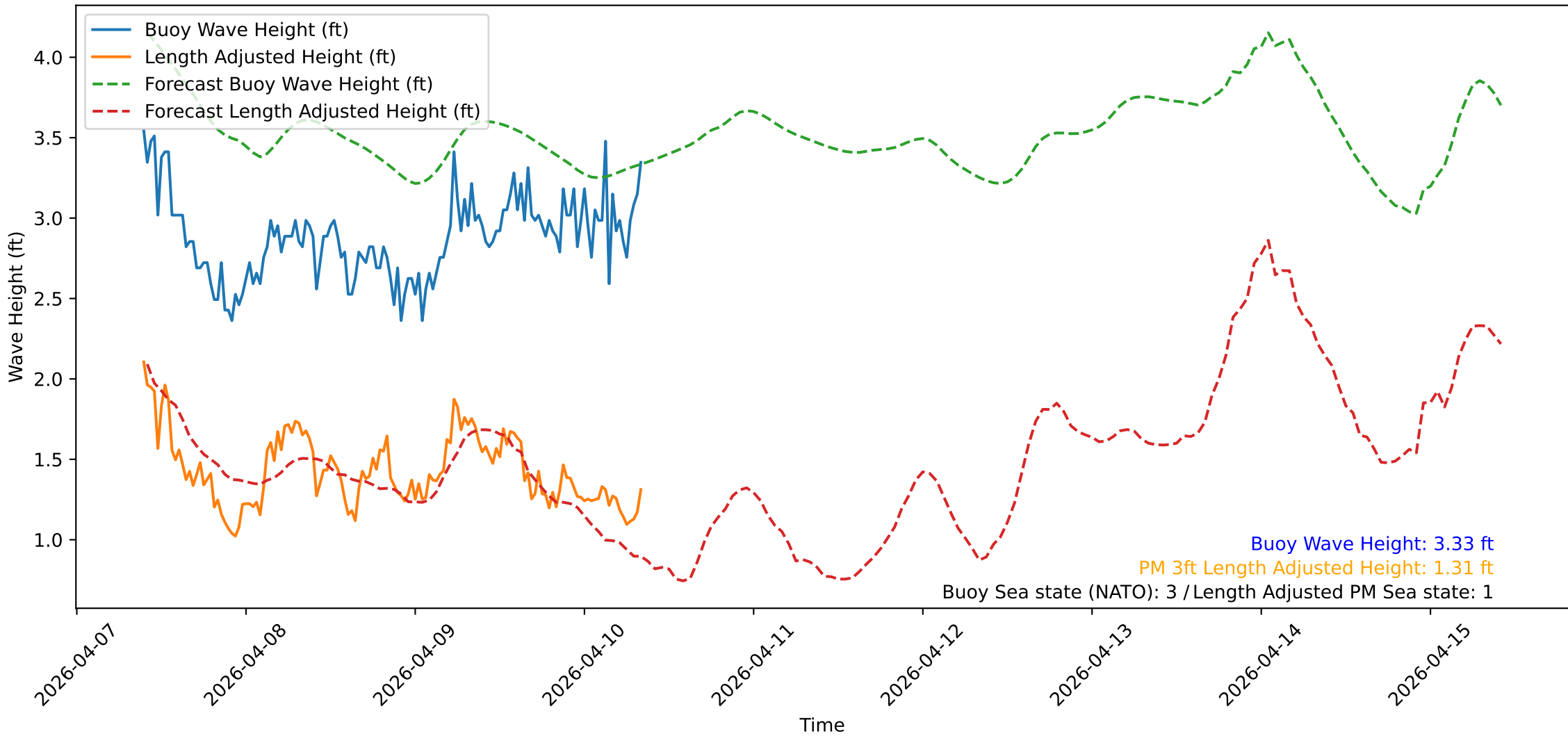
Wave Heights over Time for Green Beach at 2026-04-10 09:31:12
