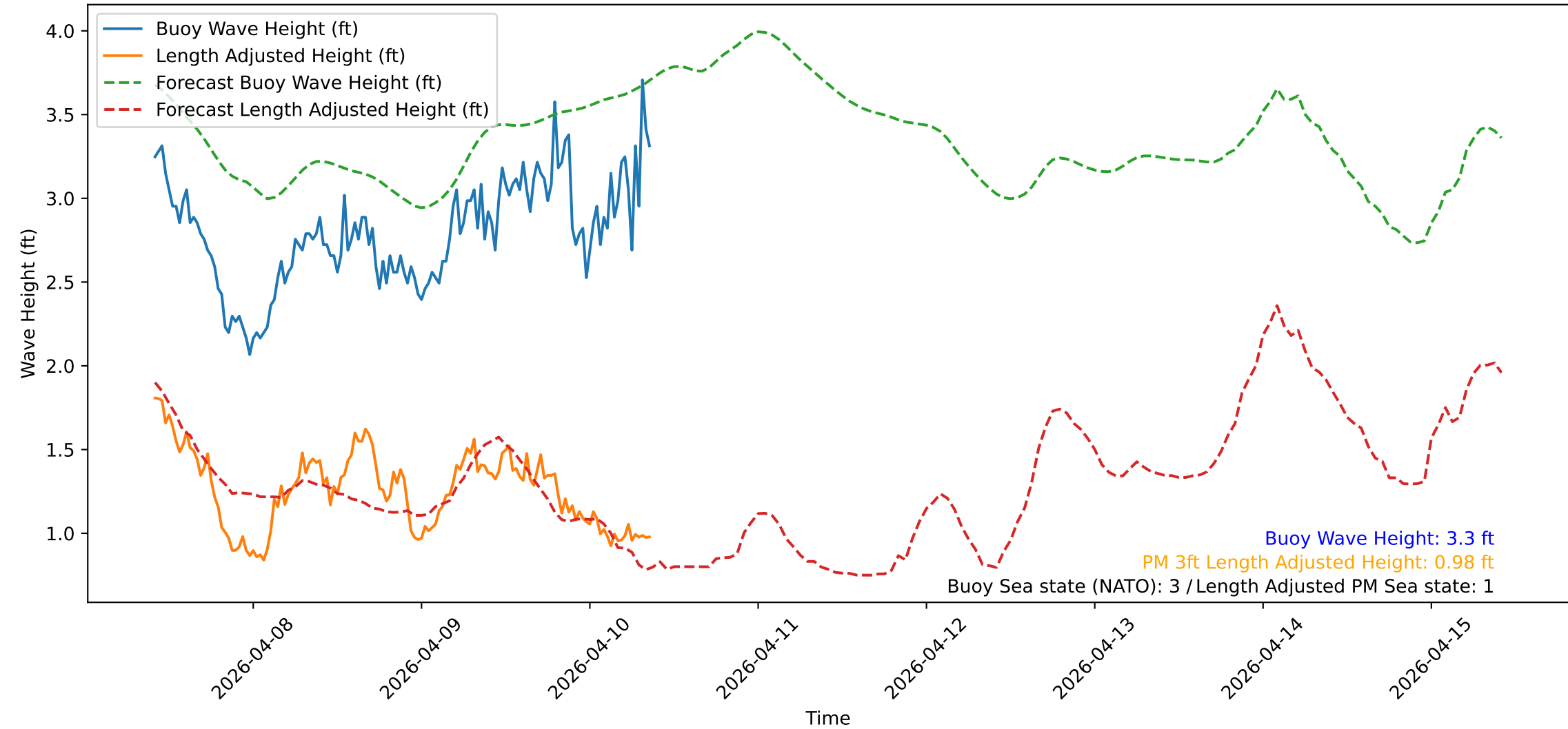
Wave Heights over Time for Red Beach at 2026-04-10 09:30:50
