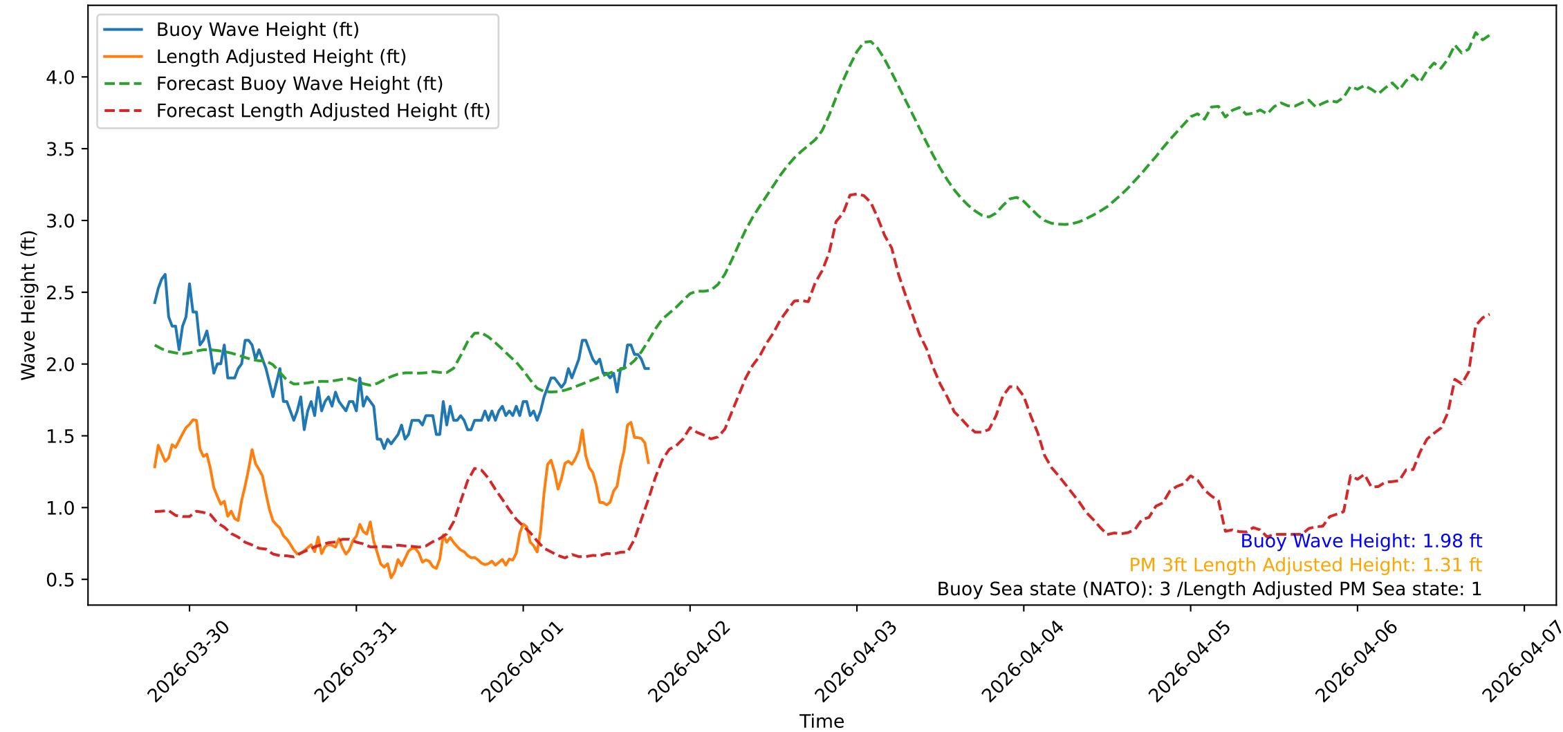
Wave Heights over Time for Green Beach at 2026-04-01 19:01:10
